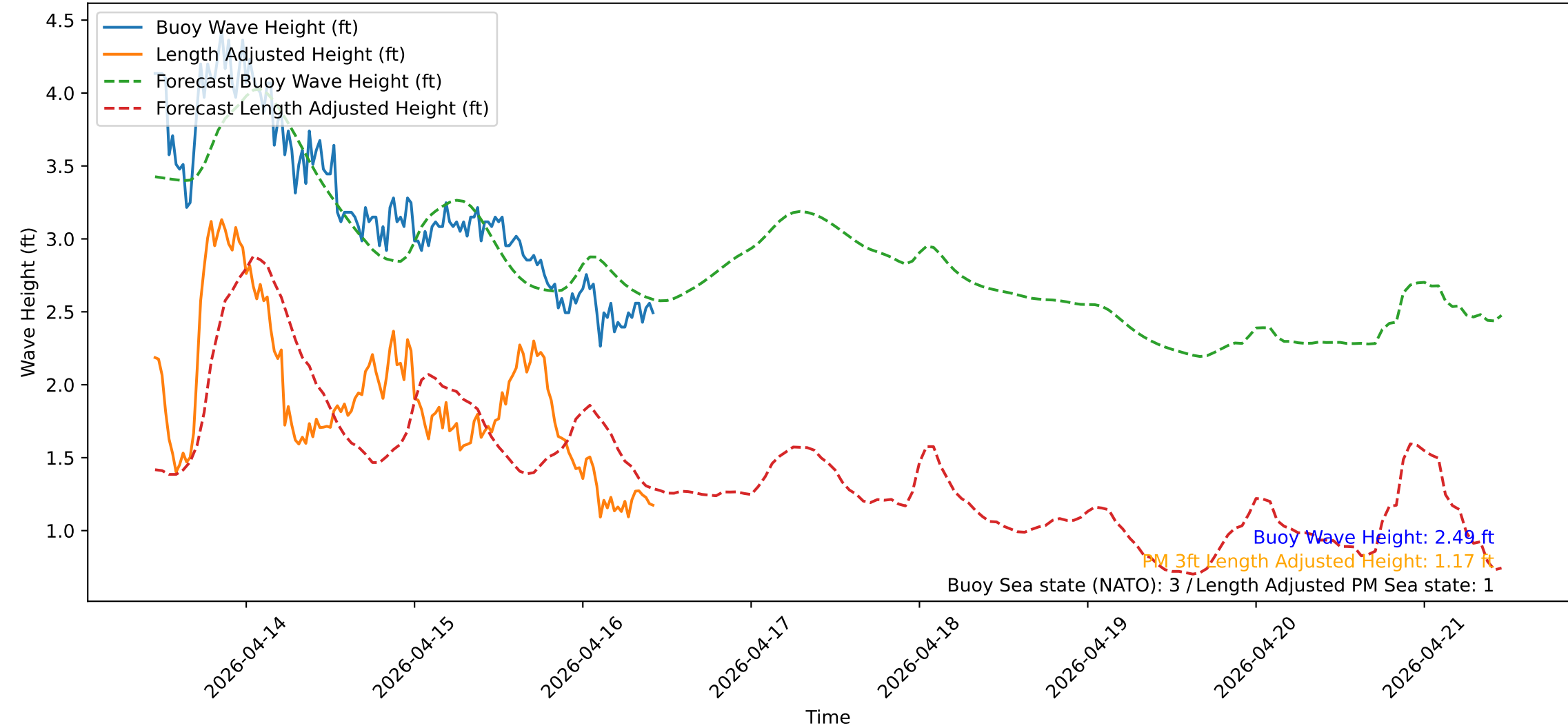
Wave Heights over Time for Red Beach at 2026-04-16 10:50:52
