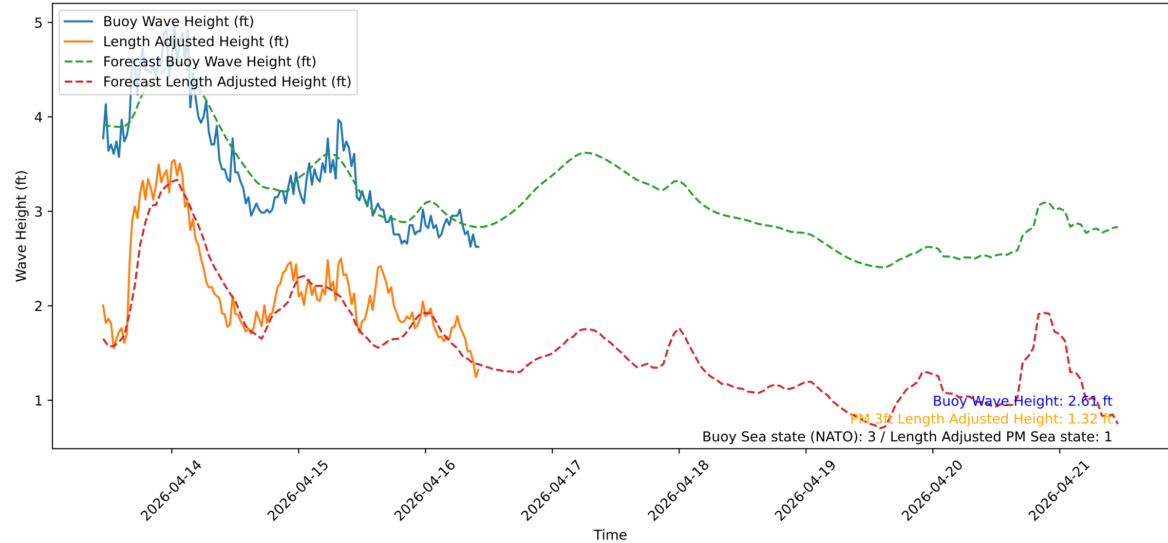
Wave Heights over Time for Green Beach at 2026-04-16 10:51:14
