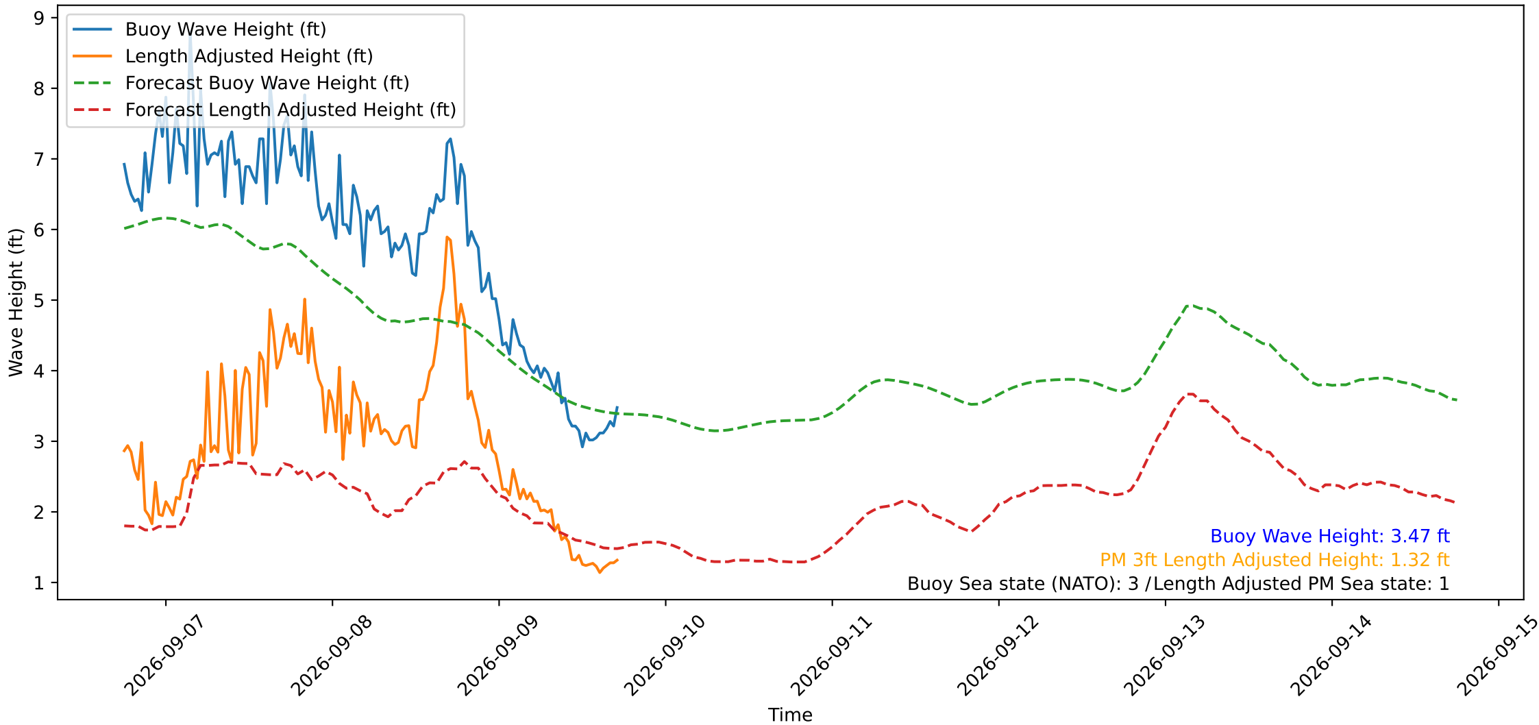
Wave Heights over Time for Green Beach at 2026-09-09 17:51:12
