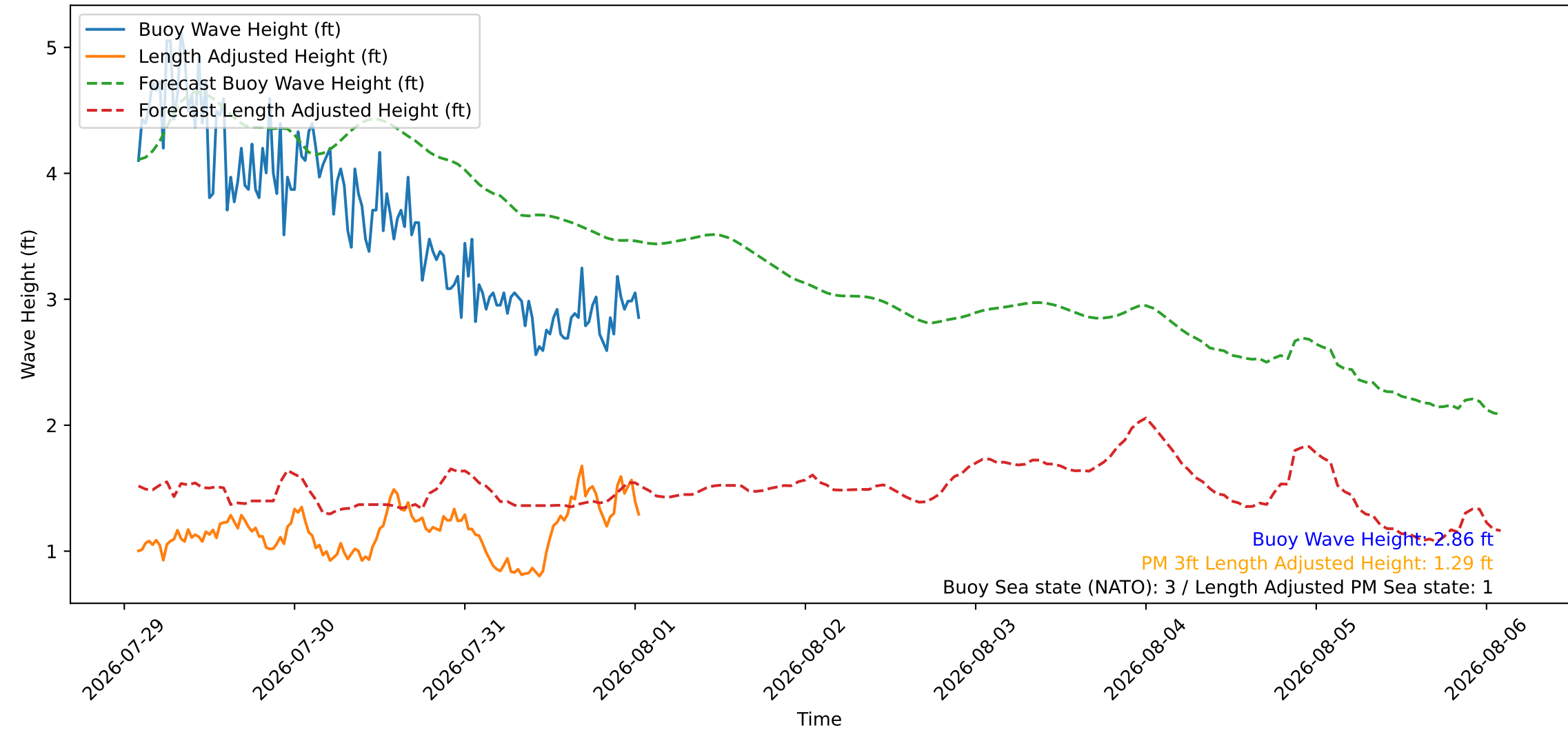
Wave Heights over Time for Red Beach at 2026-08-01 01:30:46
