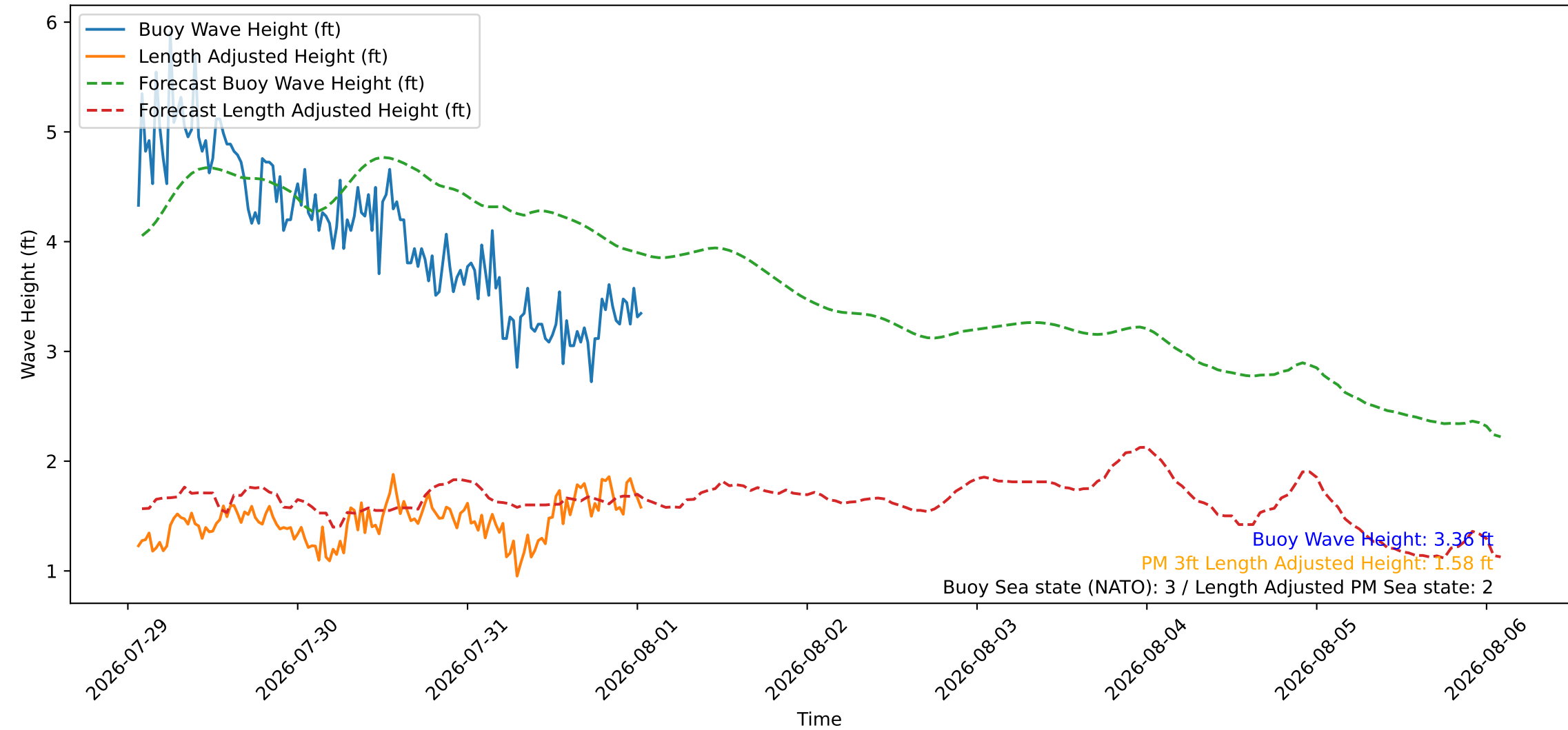
Wave Heights over Time for Oceanside Harbor at 2026-08-01 01:30:26
