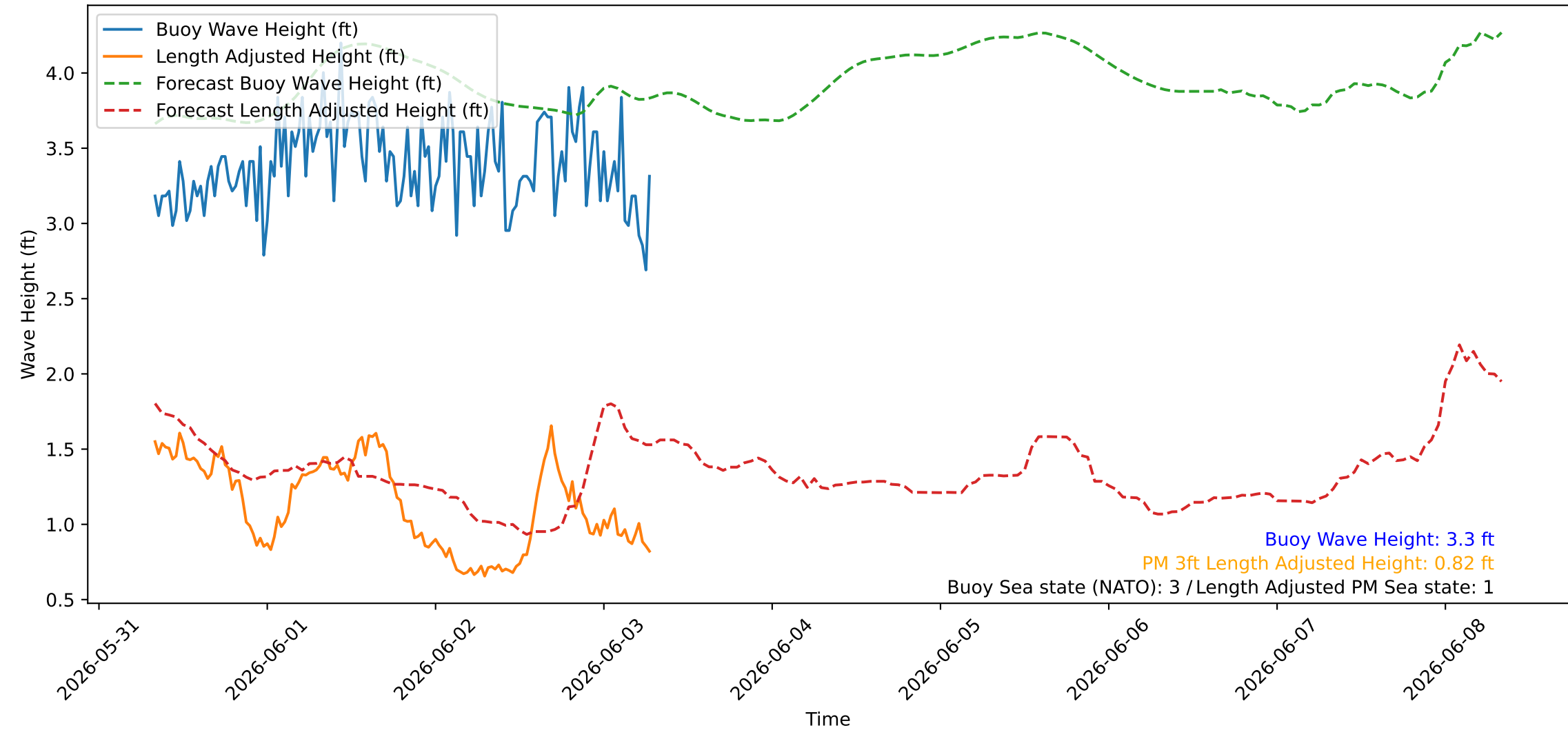
Wave Heights over Time for Red Beach at 2026-06-03 07:30:45
