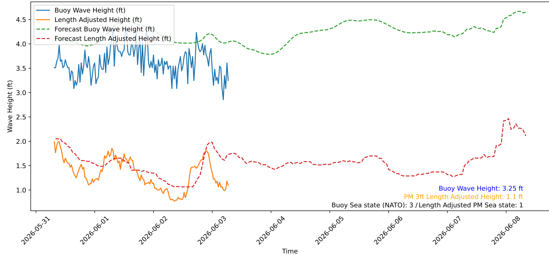
Wave Heights over Time for Green Beach at 2026-06-03 07:31:08
