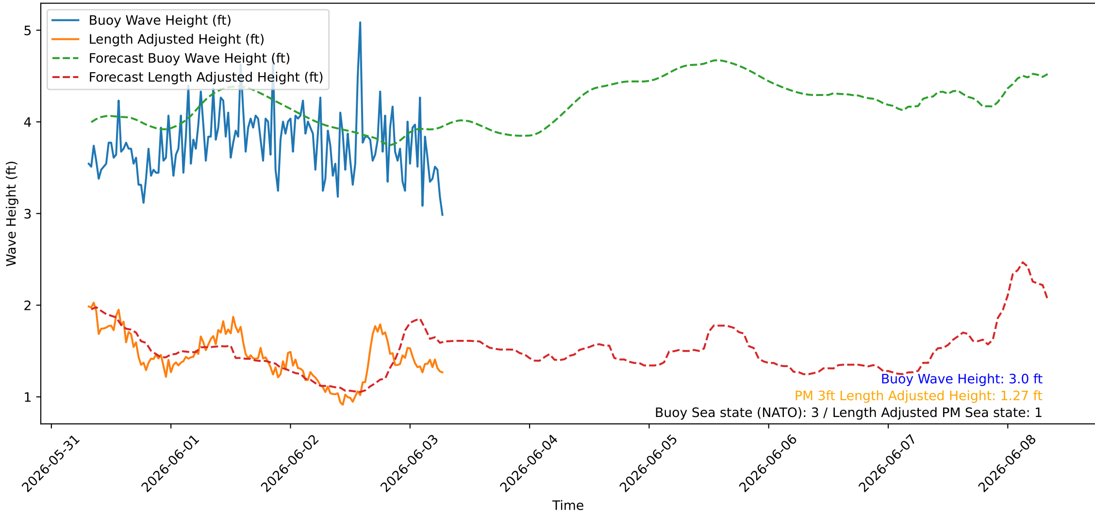
Wave Heights over Time for Oceanside Harbor at 2026-06-03 07:30:26
