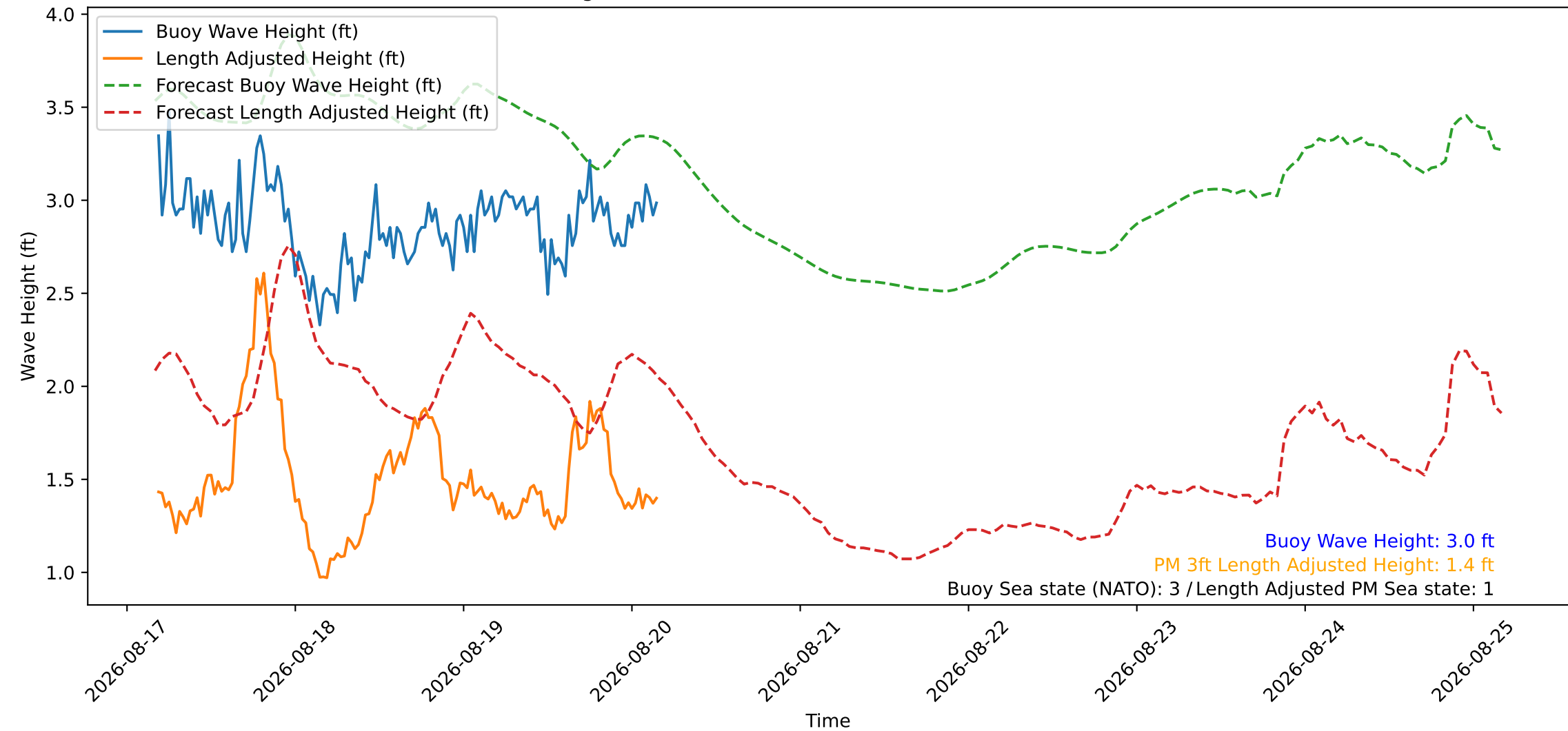
Wave Heights over Time for Red Beach at 2026-08-20 04:10:46
