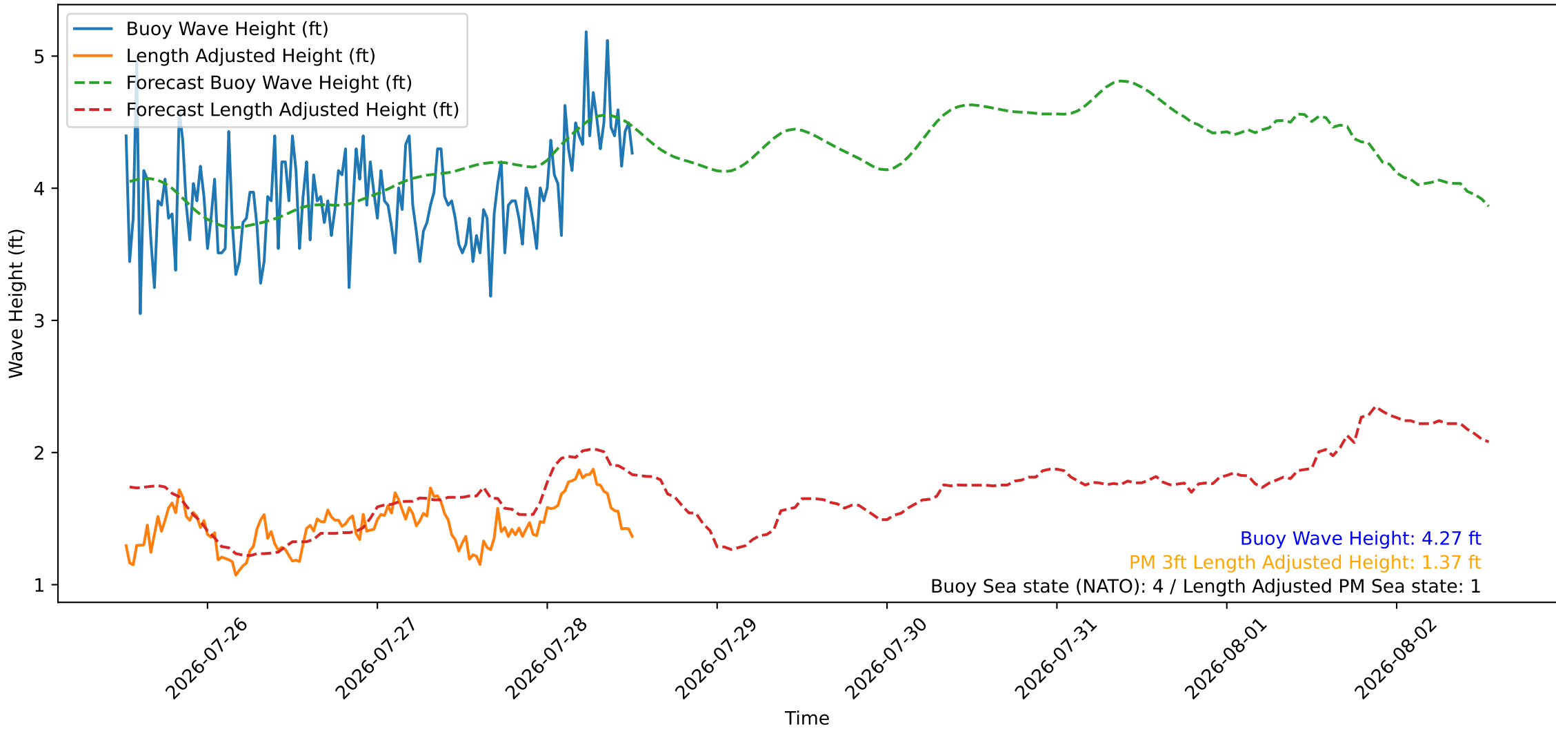
Wave Heights over Time for Oceanside Harbor at 2026-07-28 12:40:26
