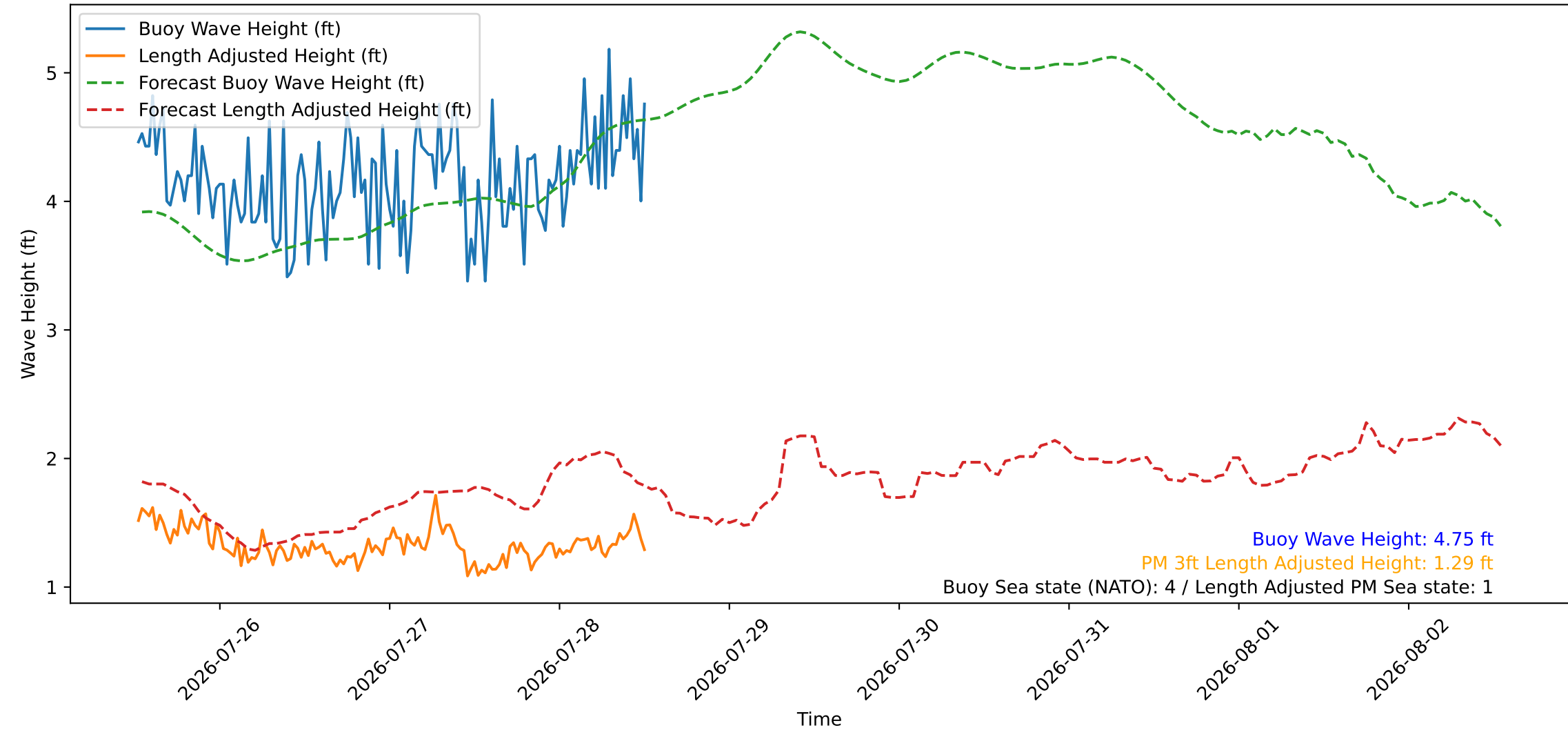
Wave Heights over Time for Green Beach at 2026-07-28 12:41:08
