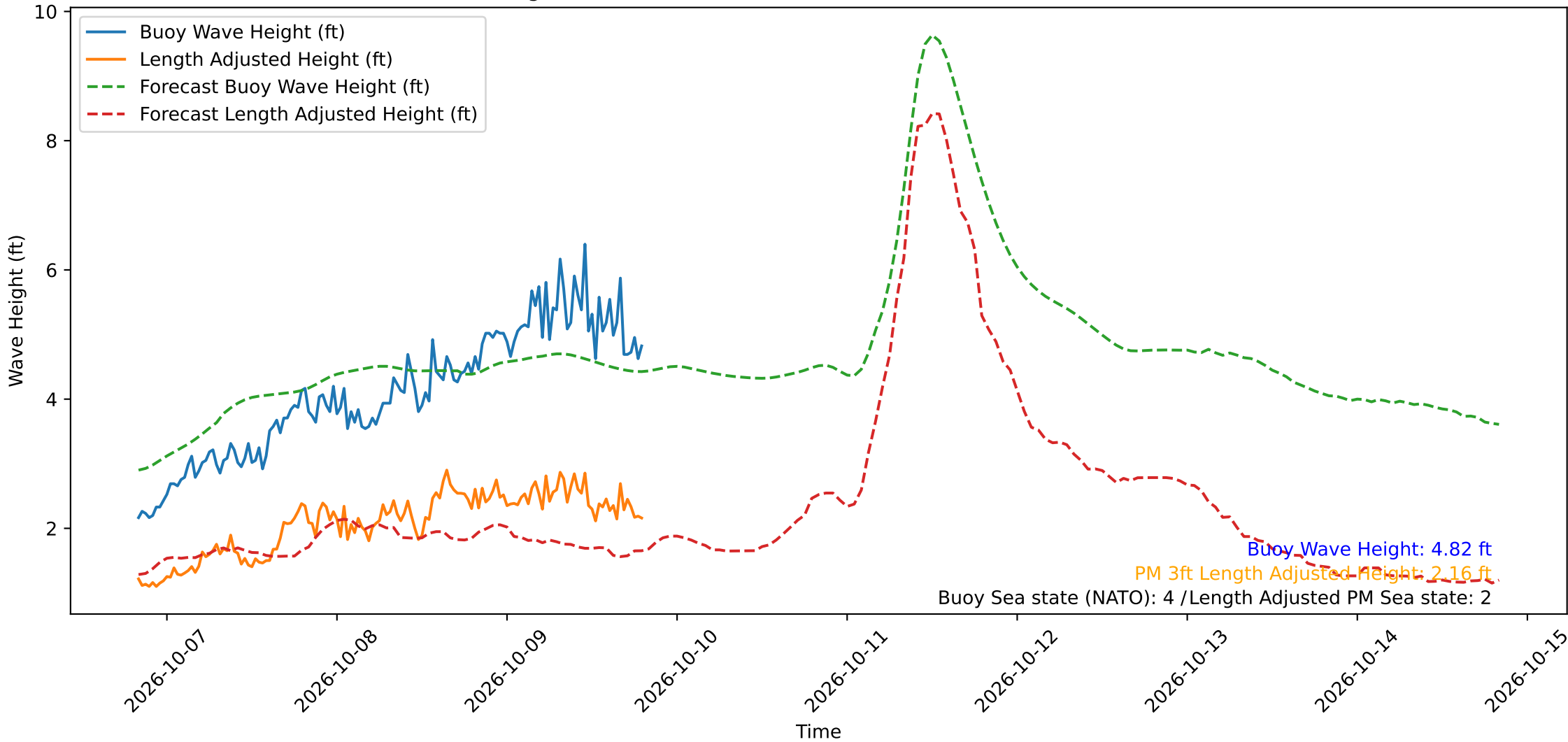
Wave Heights over Time for Oceanside Harbor at 2026-10-09 19:50:29
