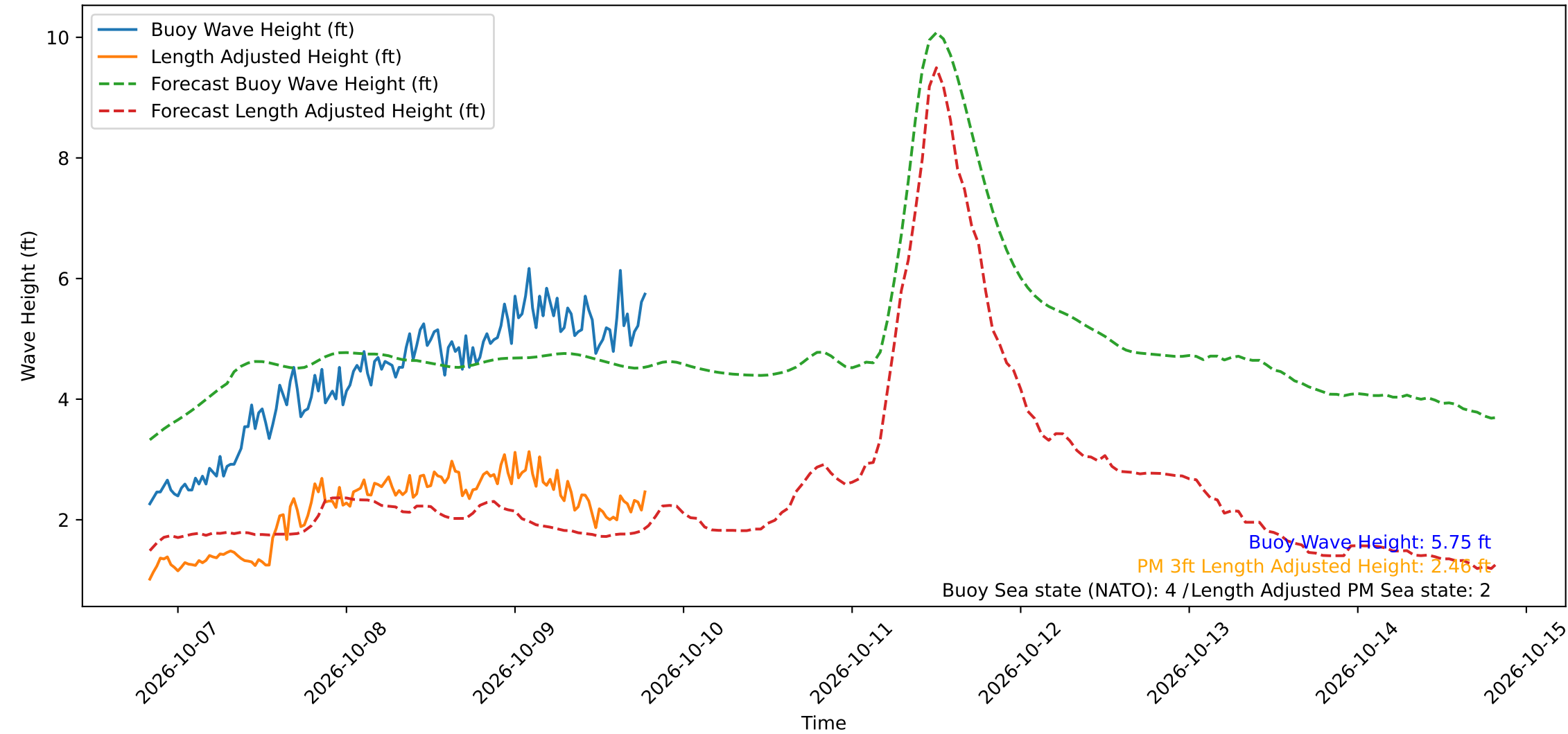
Wave Heights over Time for Green Beach at 2026-10-09 19:51:14
