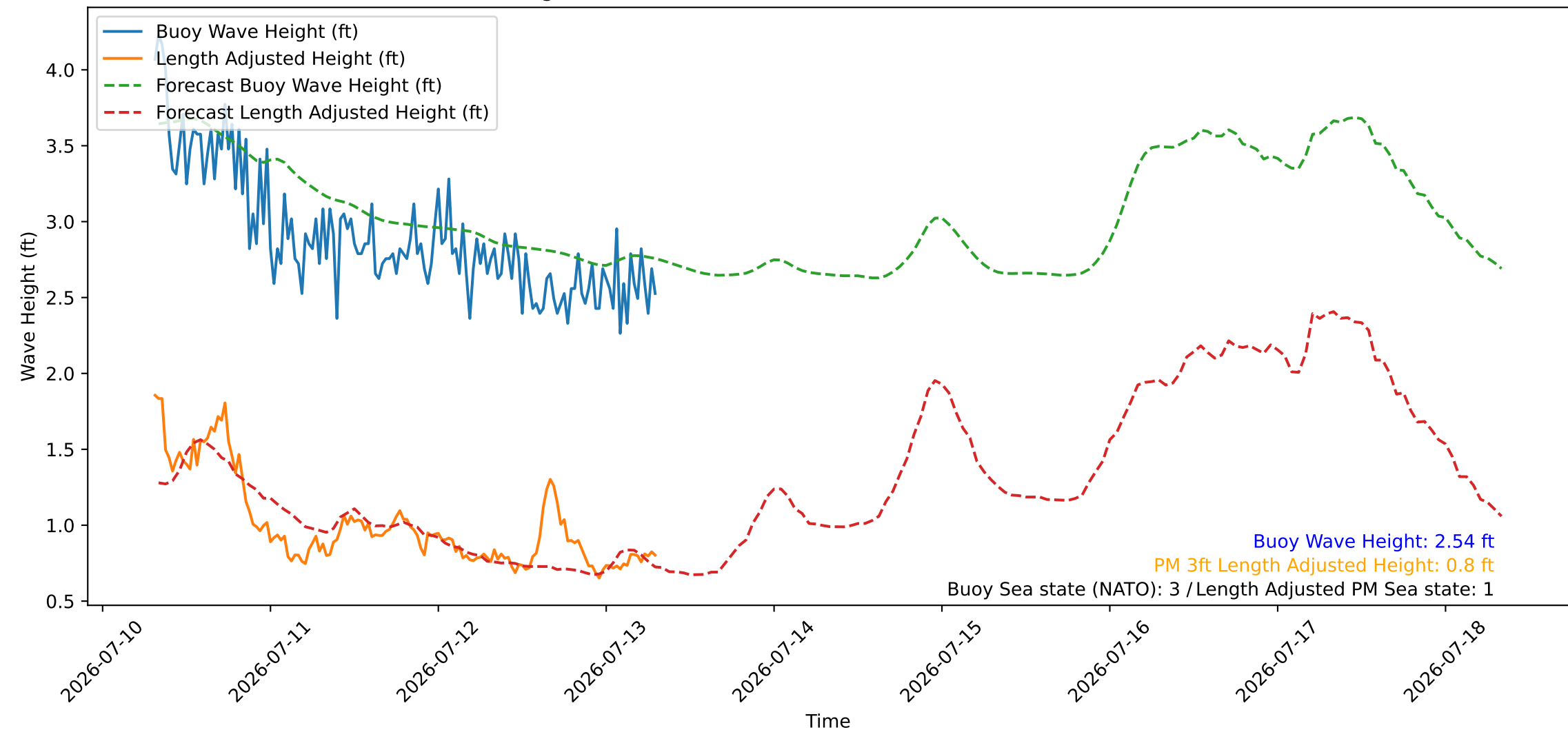
Wave Heights over Time for Oceanside Harbor at 2026-07-13 07:40:27
