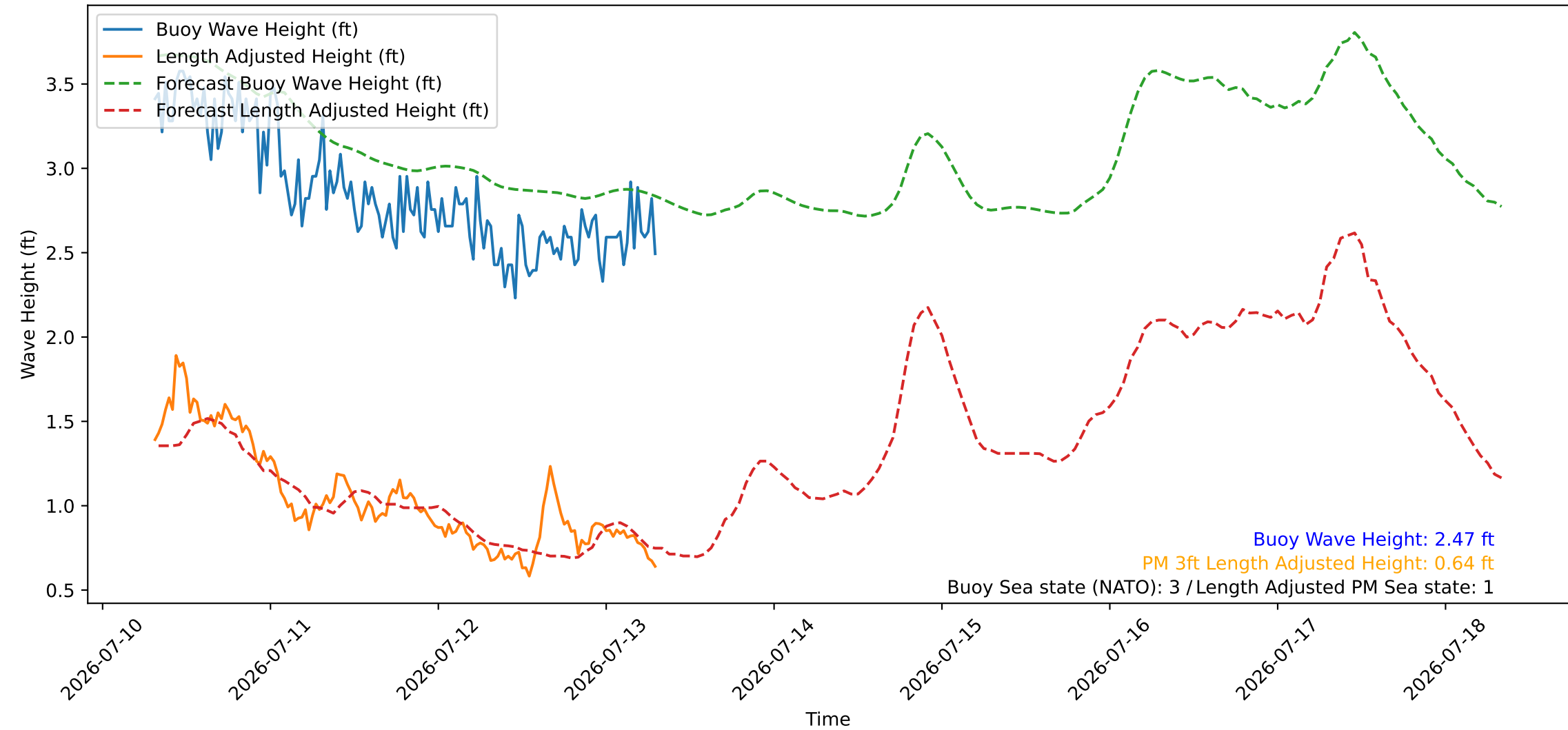
Wave Heights over Time for Green Beach at 2026-07-13 07:41:09
