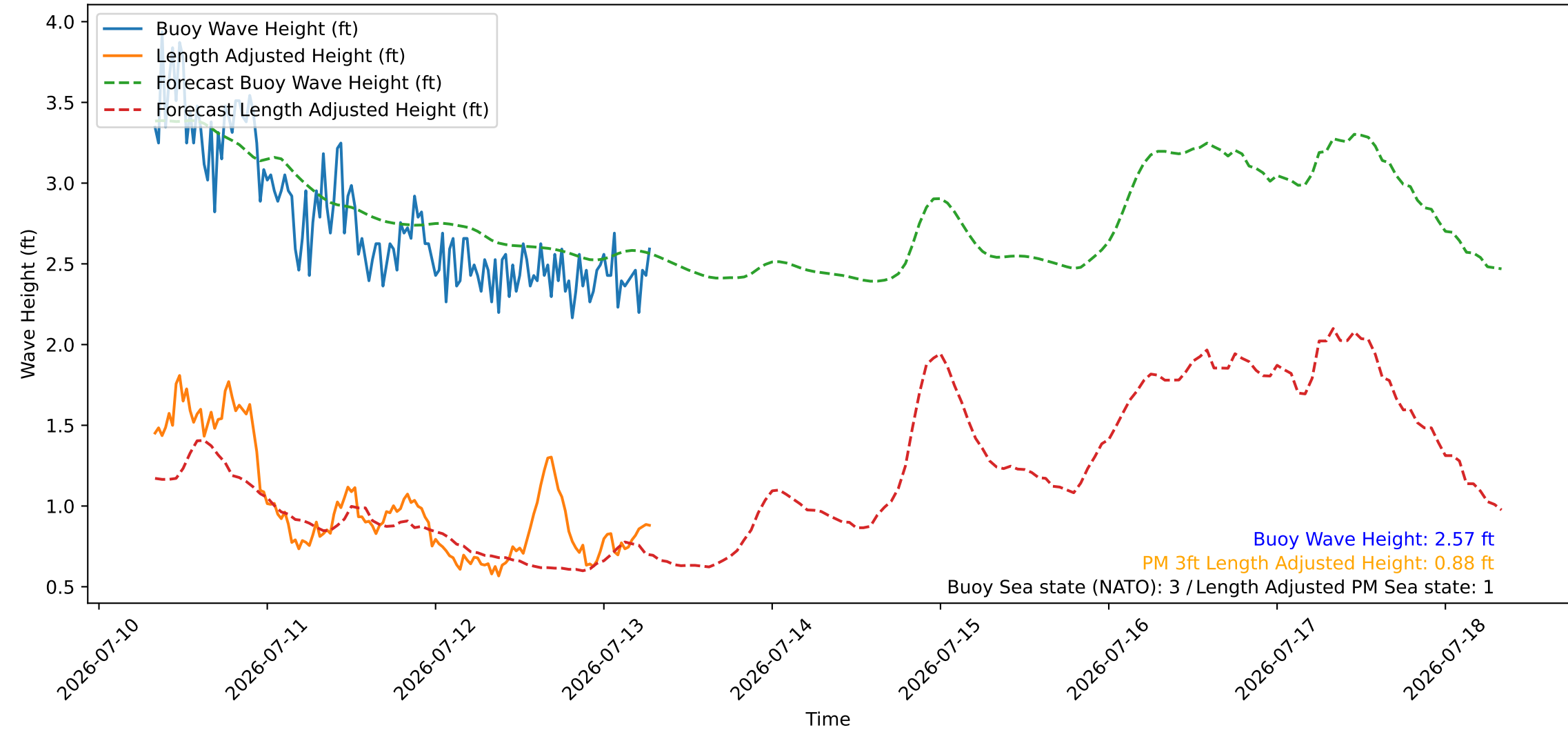
Wave Heights over Time for Red Beach at 2026-07-13 07:40:46
