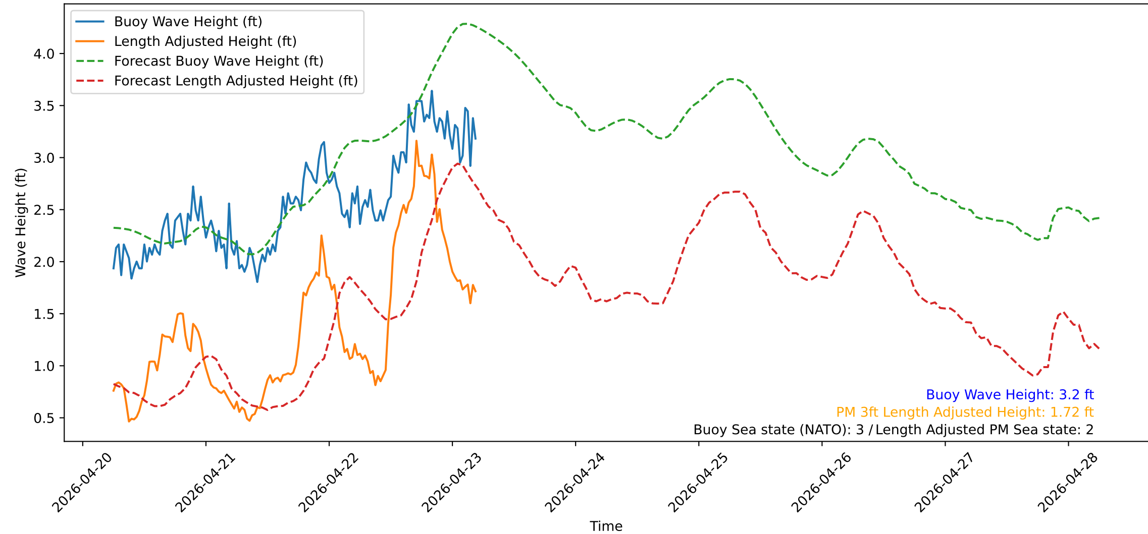
Wave Heights over Time for Red Beach at 2026-04-23 05:40:50
