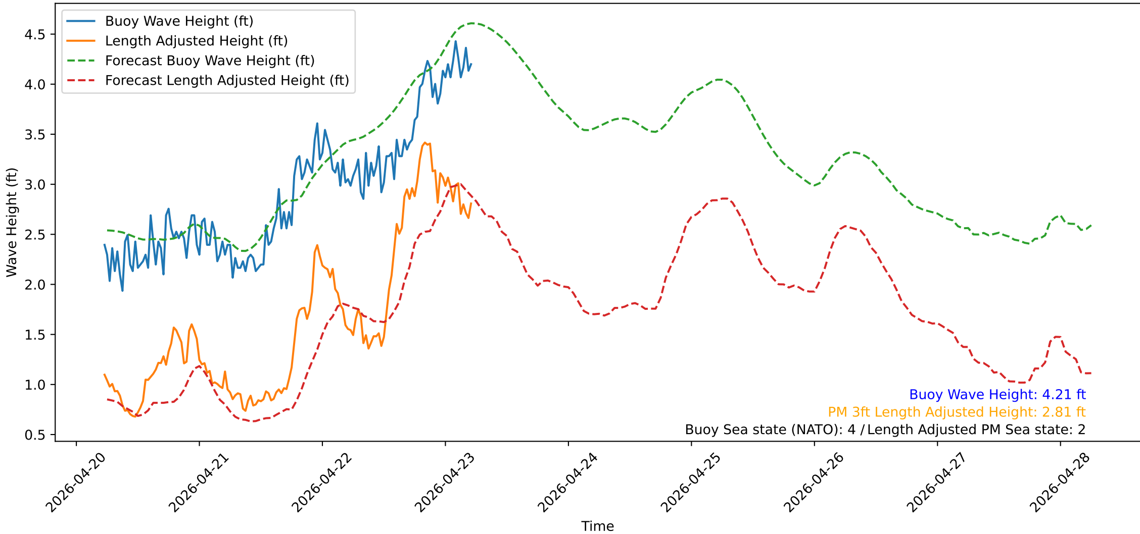
Wave Heights over Time for Oceanside Harbor at 2026-04-23 05:40:31
