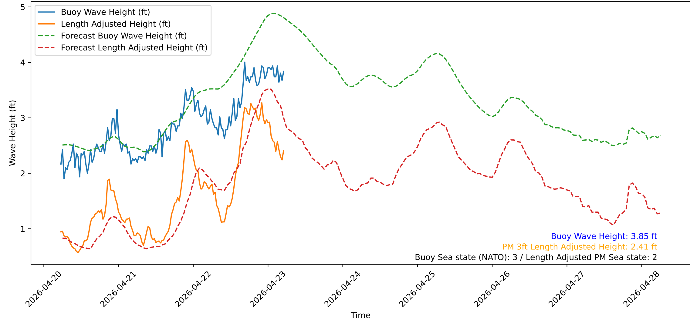
Wave Heights over Time for Green Beach at 2026-04-23 05:41:13
