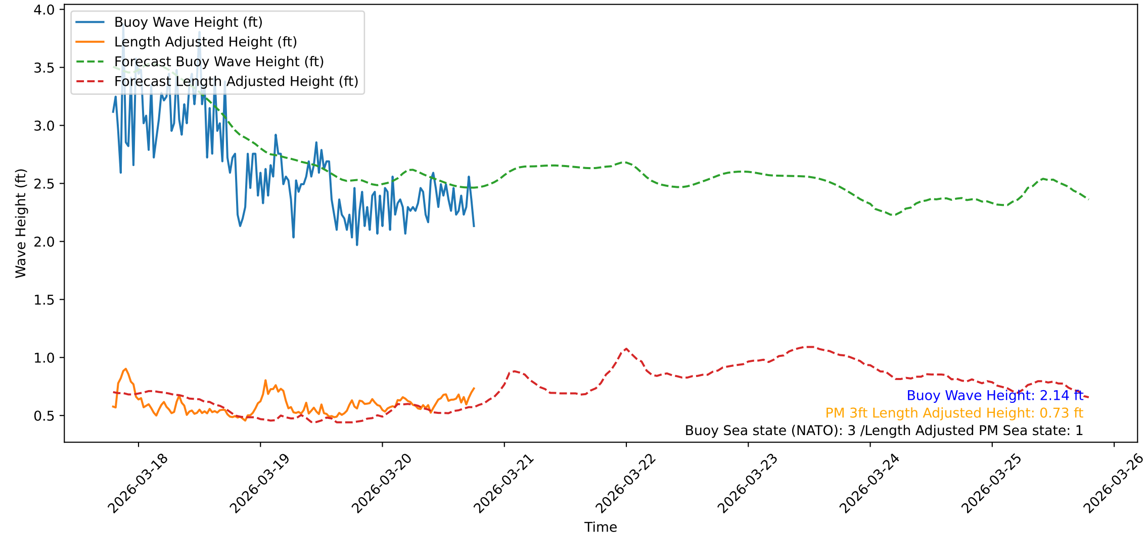
Wave Heights over Time for Oceanside Harbor at 2026-03-20 18:50:31
