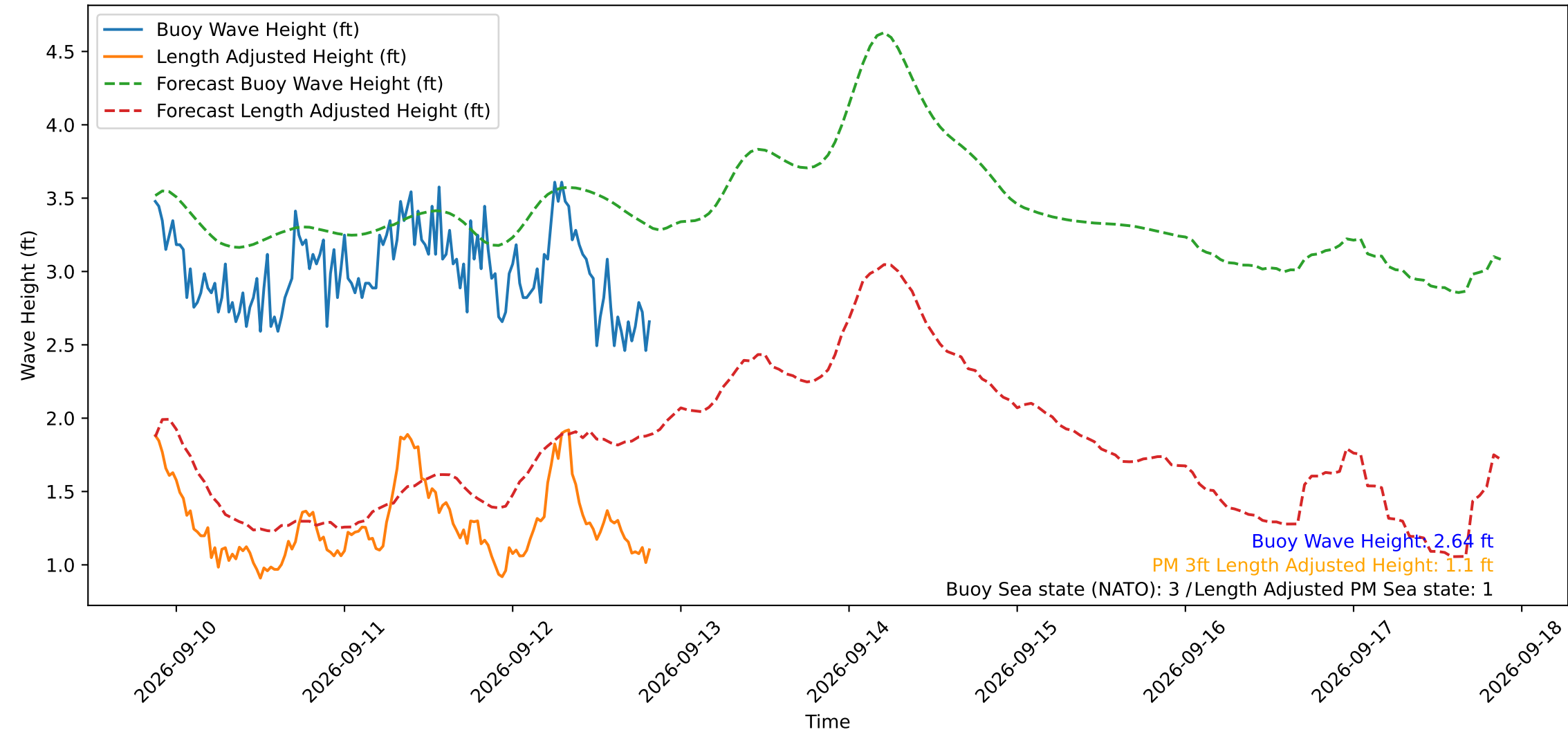
Wave Heights over Time for Green Beach at 2026-09-12 20:51:14
