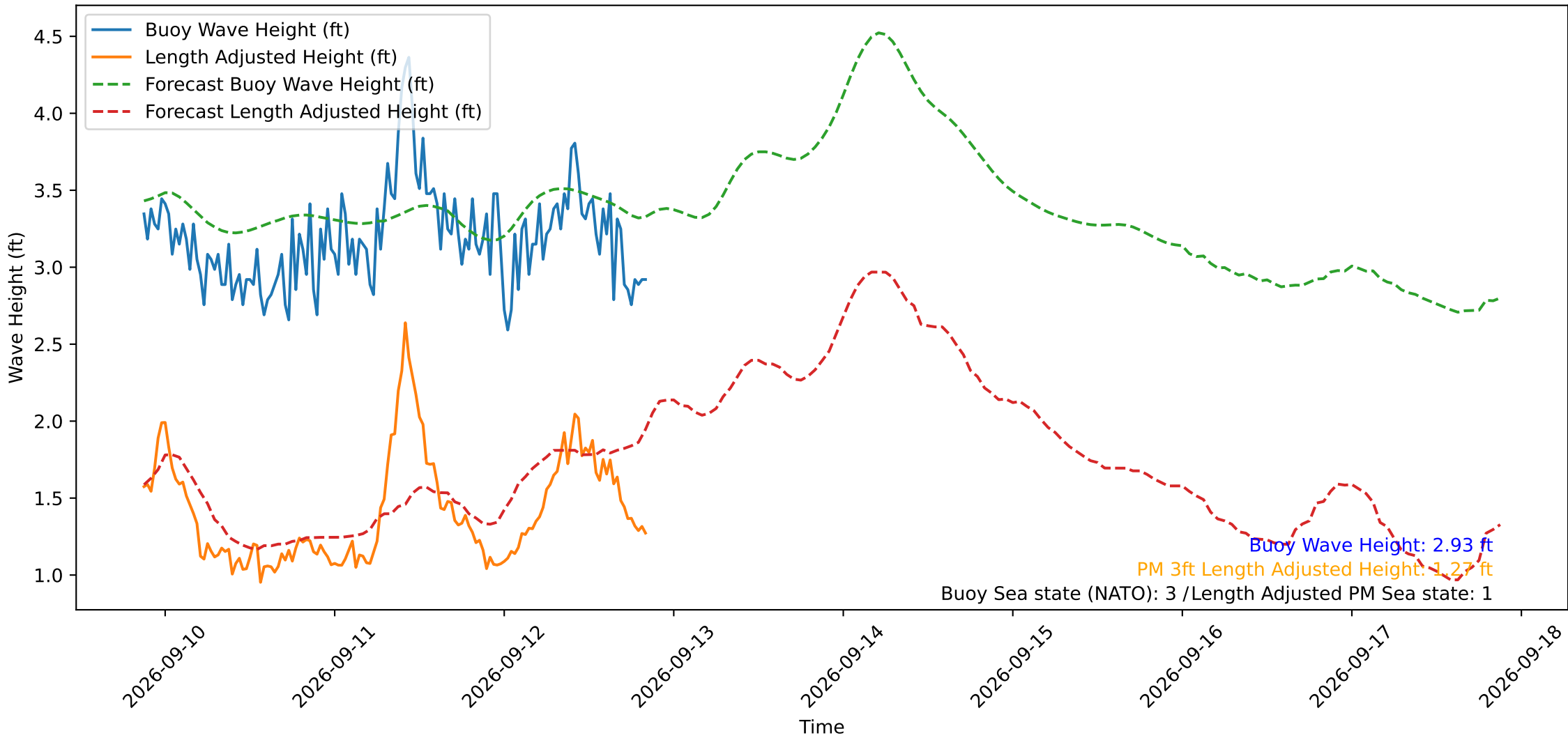
Wave Heights over Time for Oceanside Harbor at 2026-09-12 20:50:29
