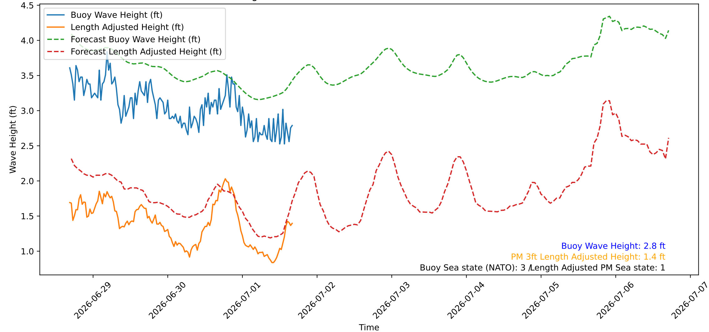
Wave Heights over Time for Green Beach at 2026-07-01 16:41:09
