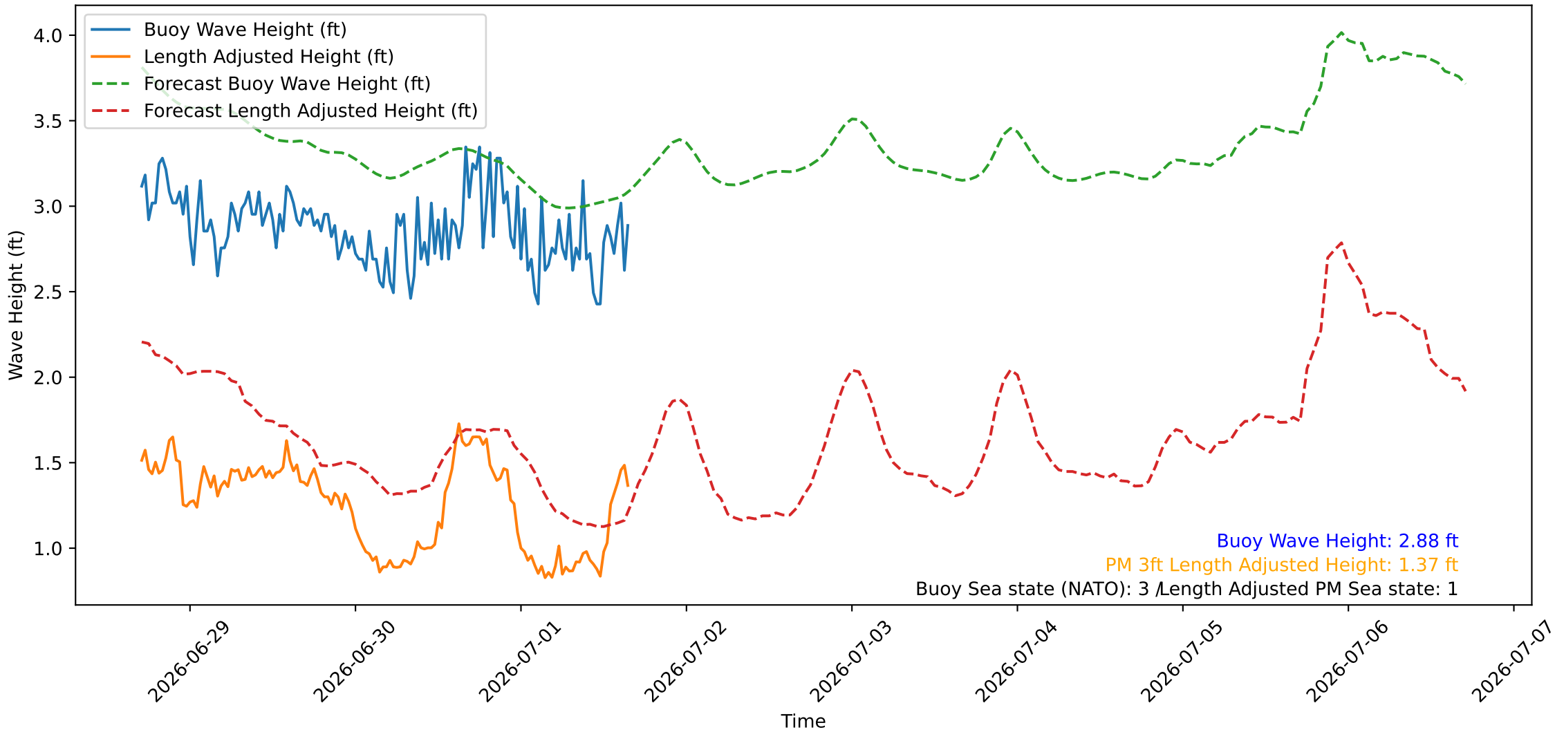
Wave Heights over Time for Red Beach at 2026-07-01 16:40:46
