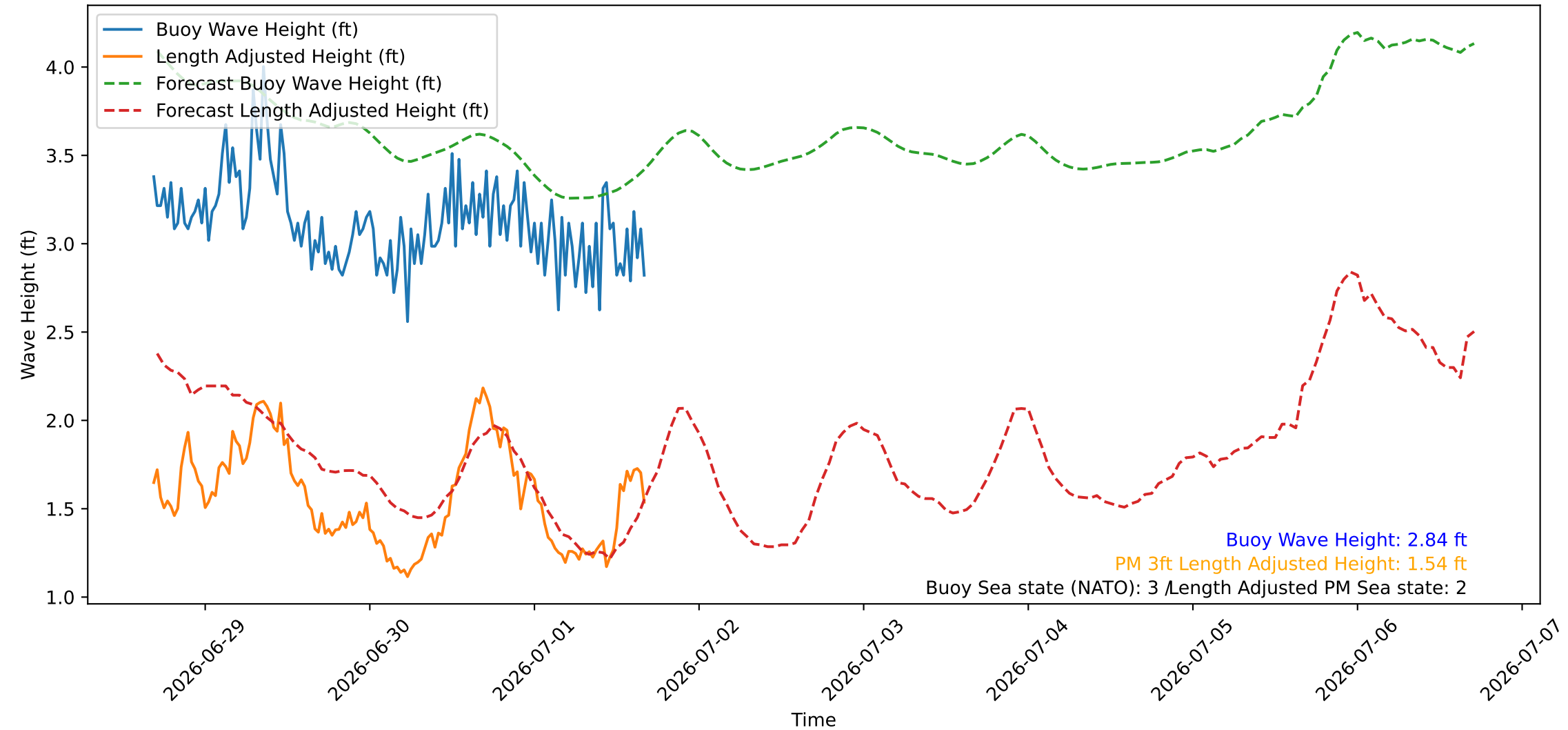
Wave Heights over Time for Oceanside Harbor at 2026-07-01 16:40:27
