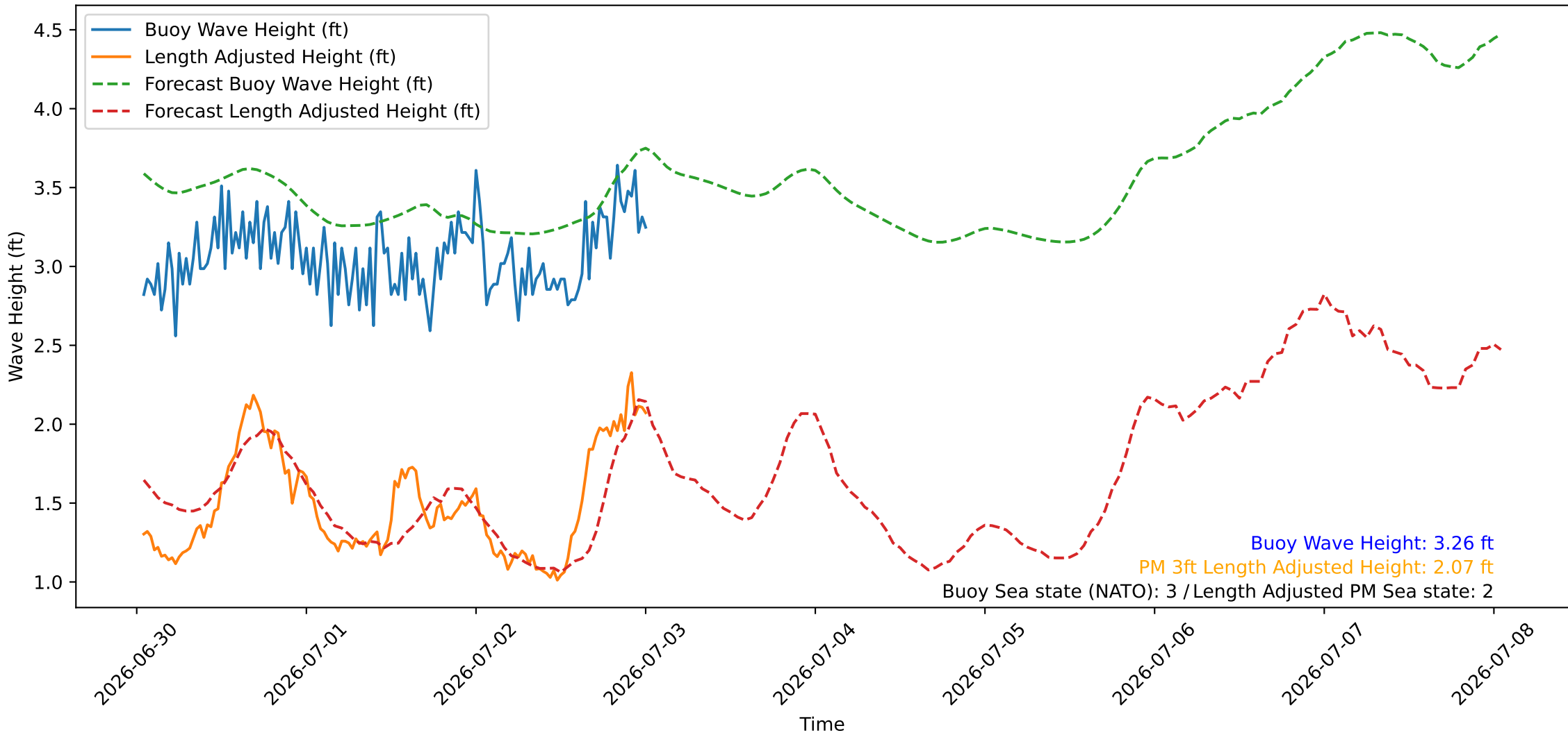
Wave Heights over Time for Oceanside Harbor at 2026-07-03 00:50:26
