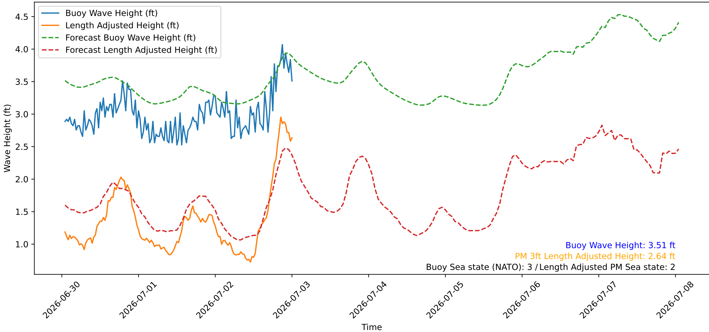
Wave Heights over Time for Green Beach at 2026-07-03 00:51:09
