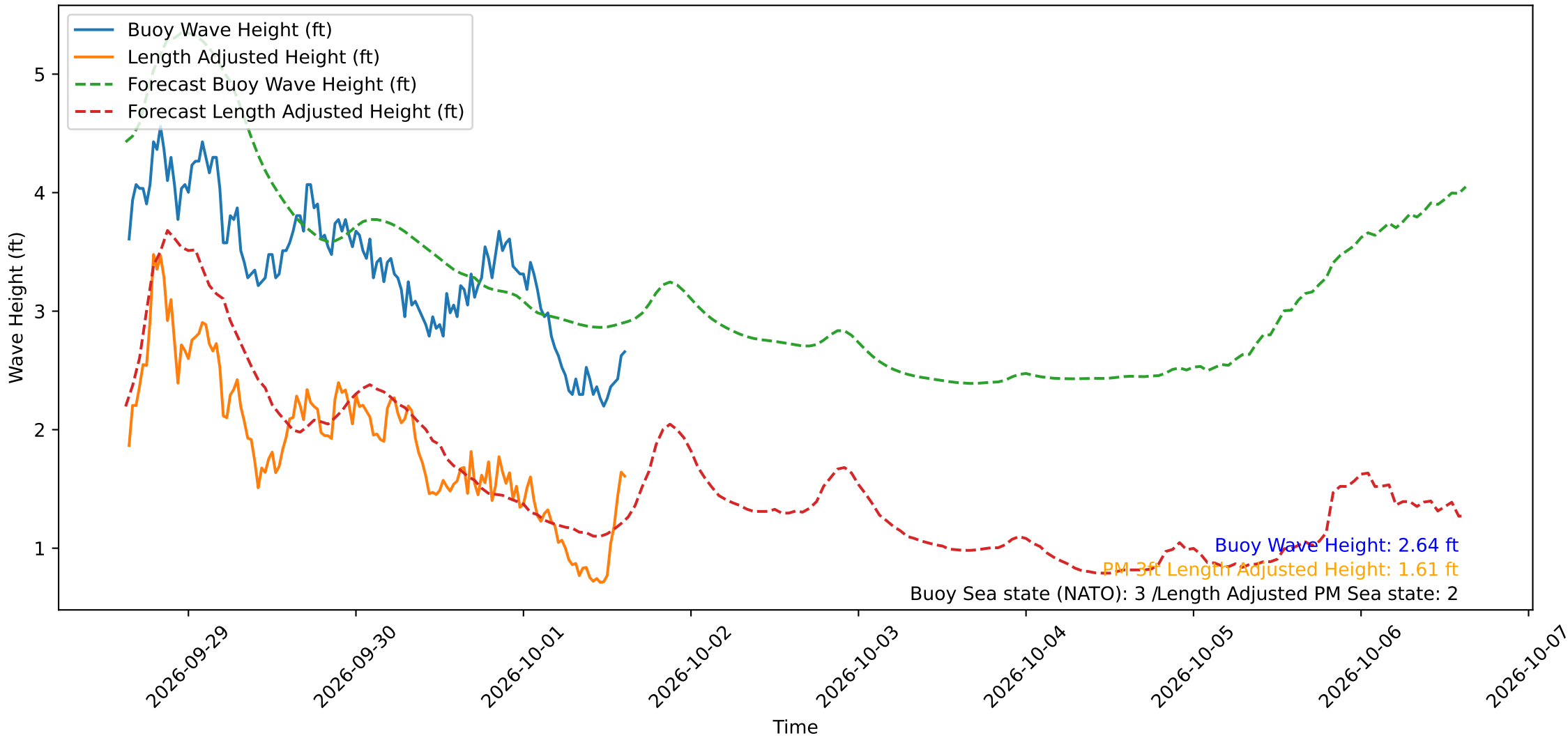
Wave Heights over Time for Green Beach at 2026-10-01 15:11:12
