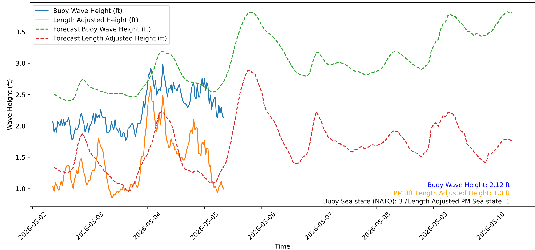
Wave Heights over Time for Green Beach at 2026-05-05 08:41:13
