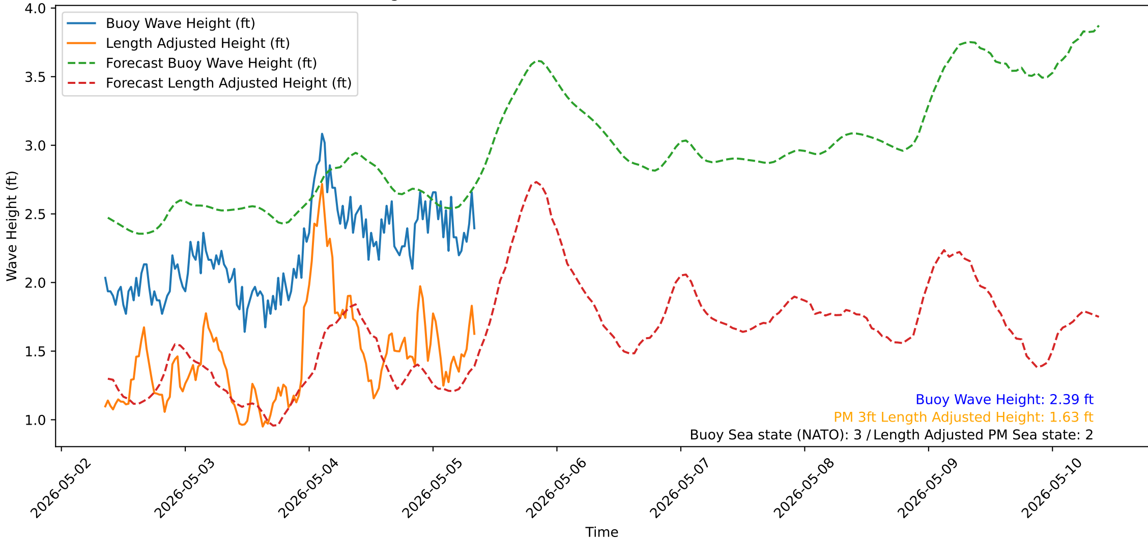
Wave Heights over Time for Oceanside Harbor at 2026-05-05 08:40:31
