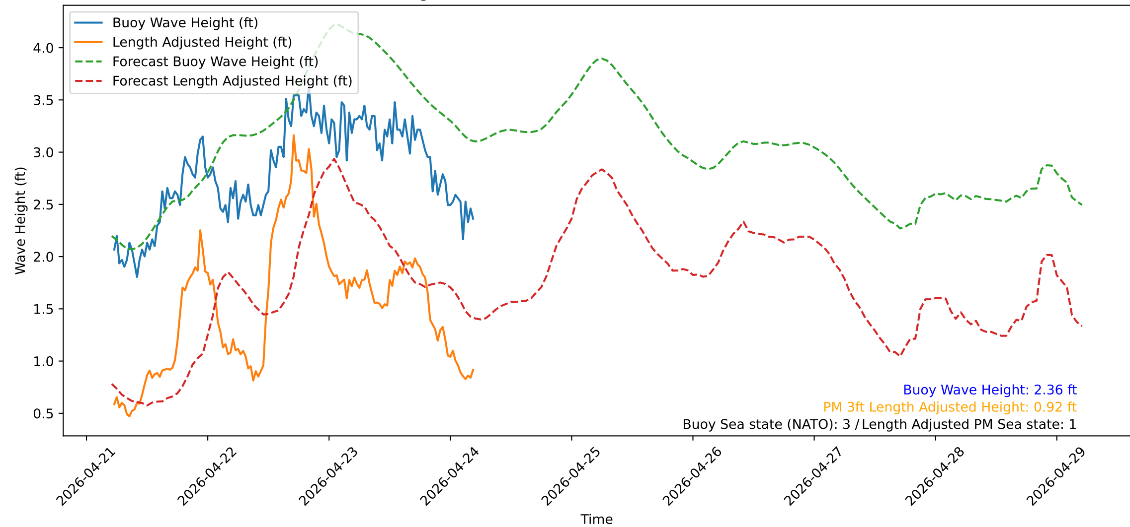
Wave Heights over Time for Red Beach at 2026-04-24 05:10:51
