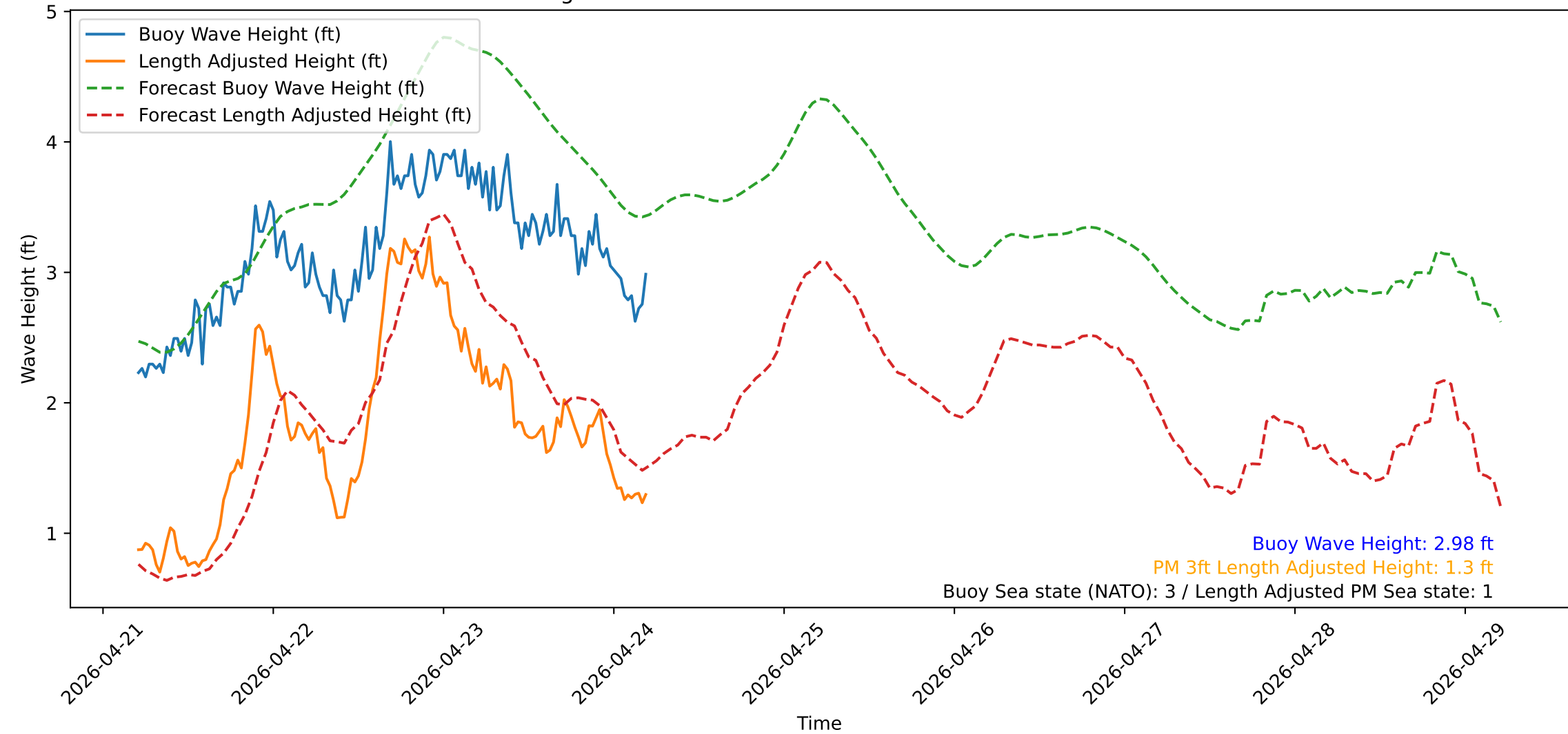
Wave Heights over Time for Green Beach at 2026-04-24 05:11:13
