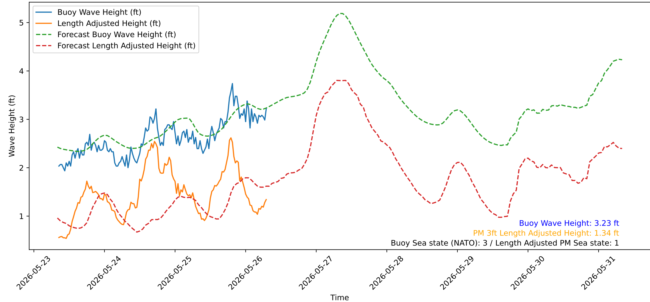
Wave Heights over Time for Red Beach at 2026-05-26 08:10:48
