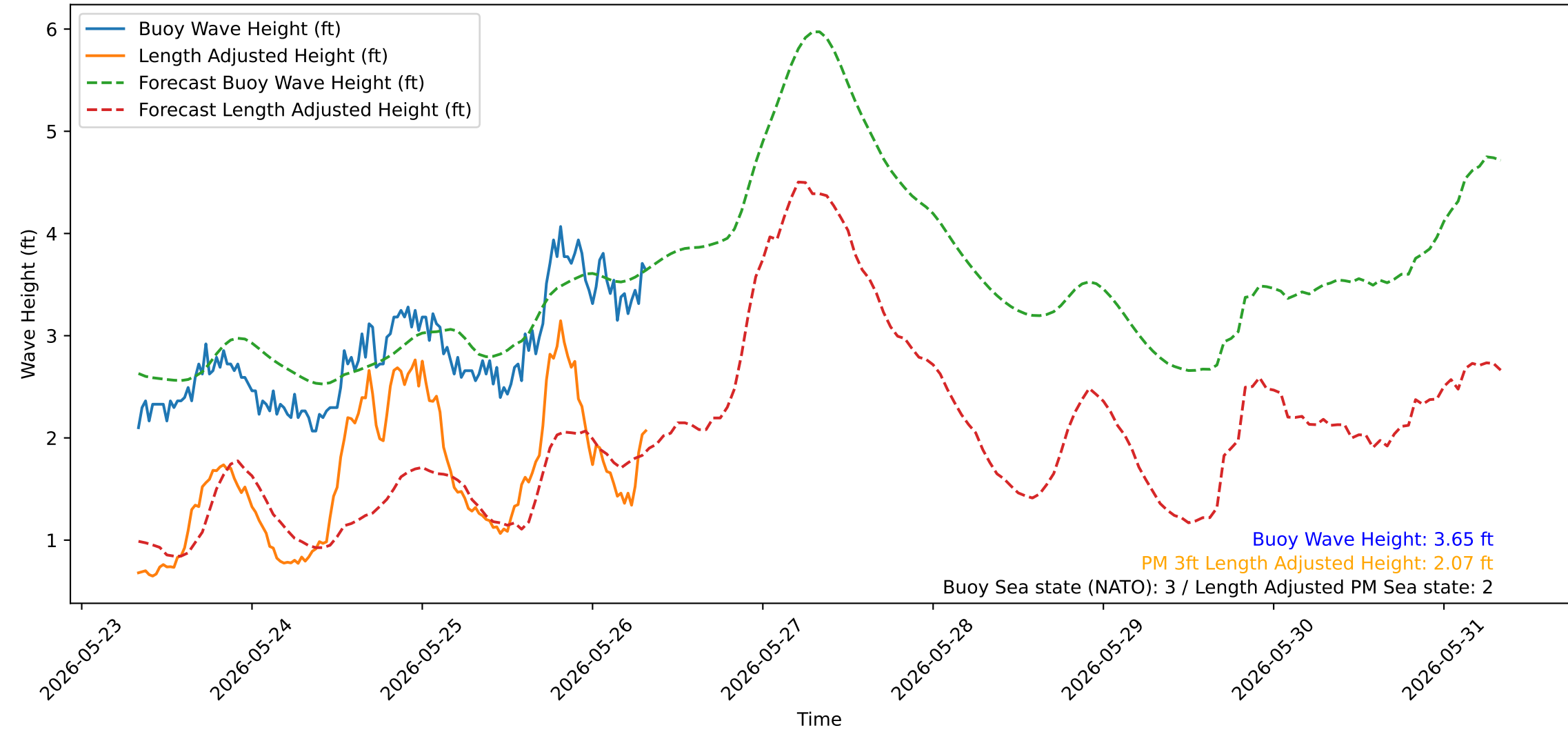
Wave Heights over Time for Green Beach at 2026-05-26 08:11:10
