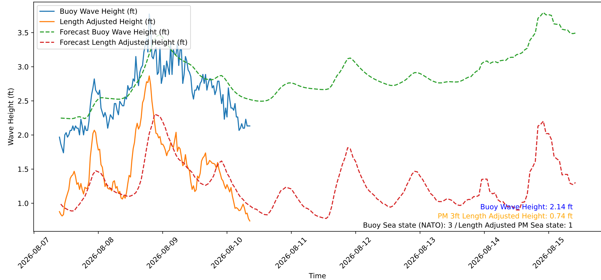
Wave Heights over Time for Green Beach at 2026-08-10 09:31:09
