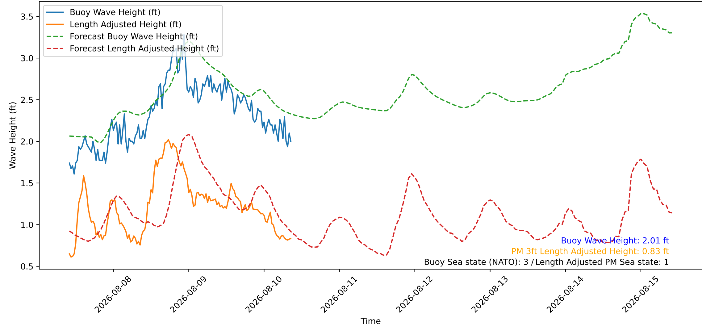
Wave Heights over Time for Red Beach at 2026-08-10 09:30:47
