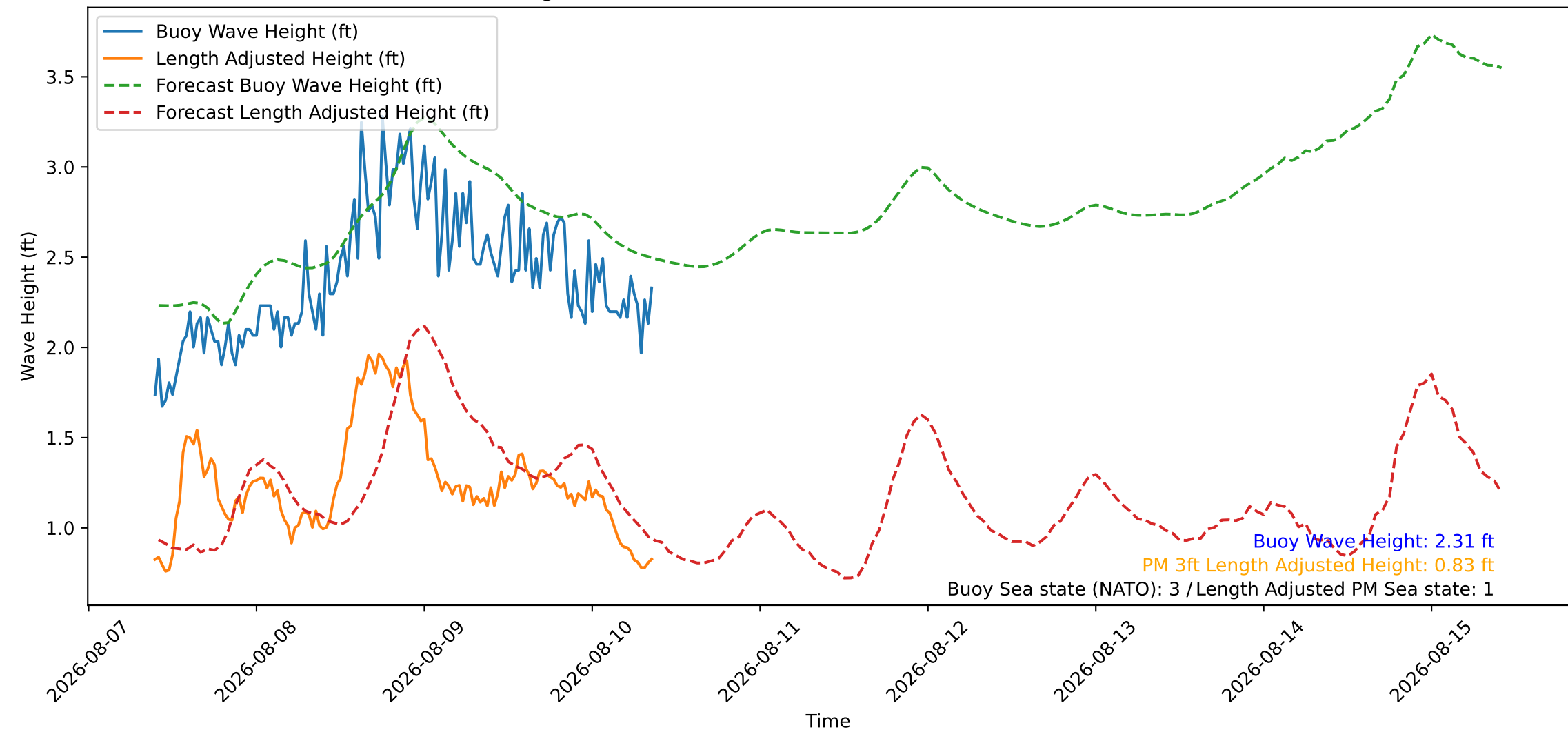
Wave Heights over Time for Oceanside Harbor at 2026-08-10 09:30:27
