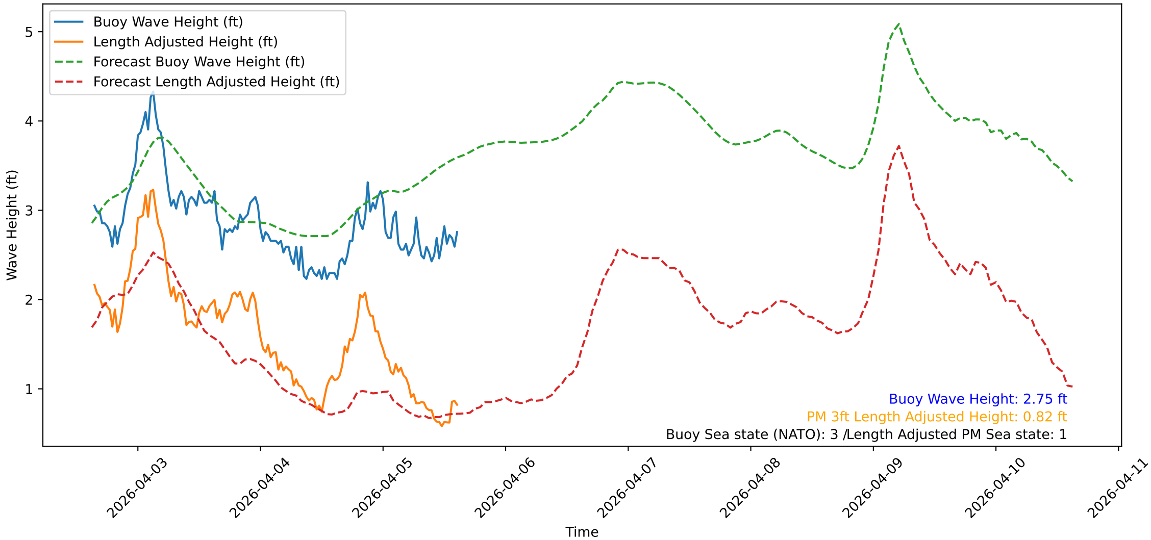
Wave Heights over Time for Green Beach at 2026-04-05 15:21:10
