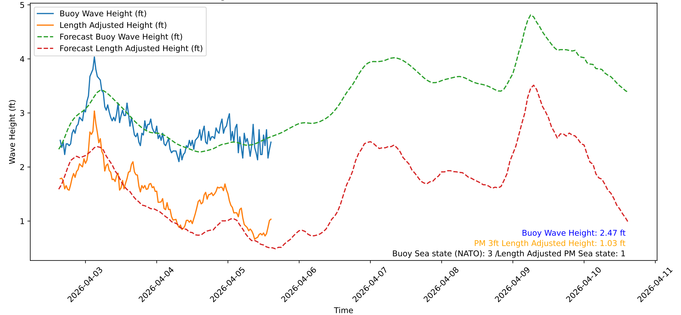
Wave Heights over Time for Oceanside Harbor at 2026-04-05 15:20:32
