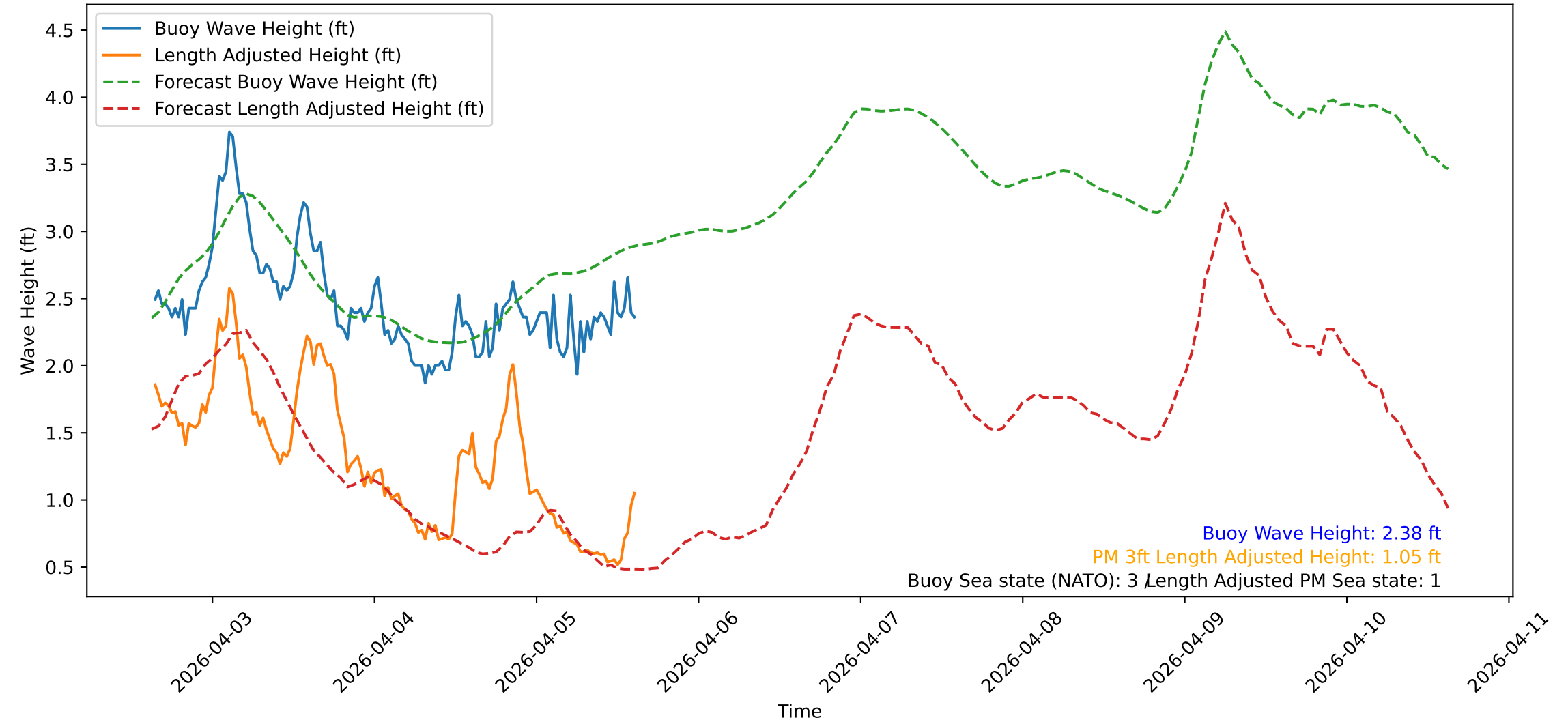
Wave Heights over Time for Red Beach at 2026-04-05 15:20:48
