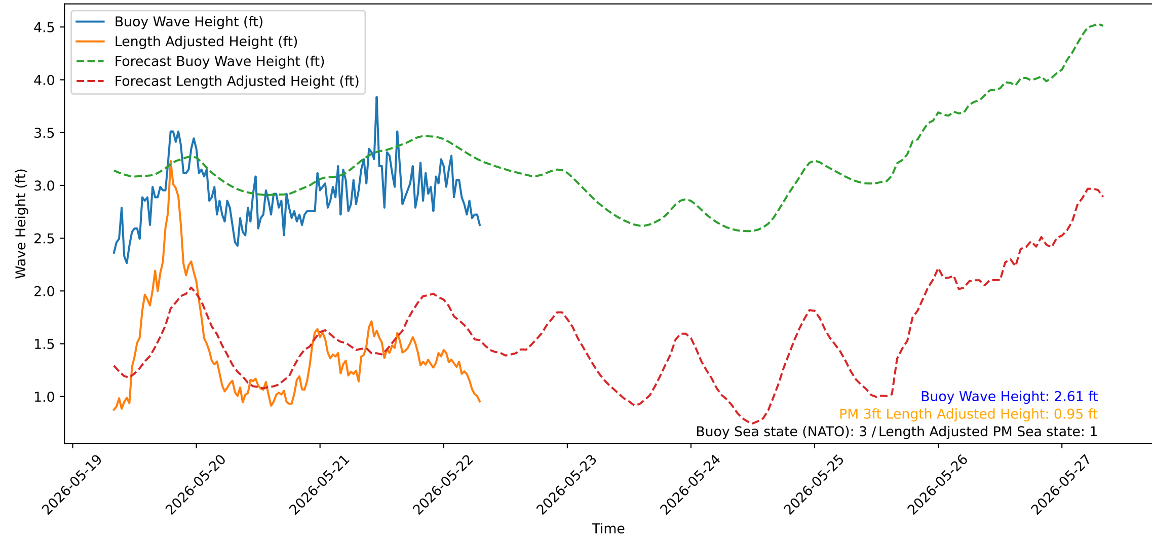
Wave Heights over Time for Oceanside Harbor at 2026-05-22 07:50:32
