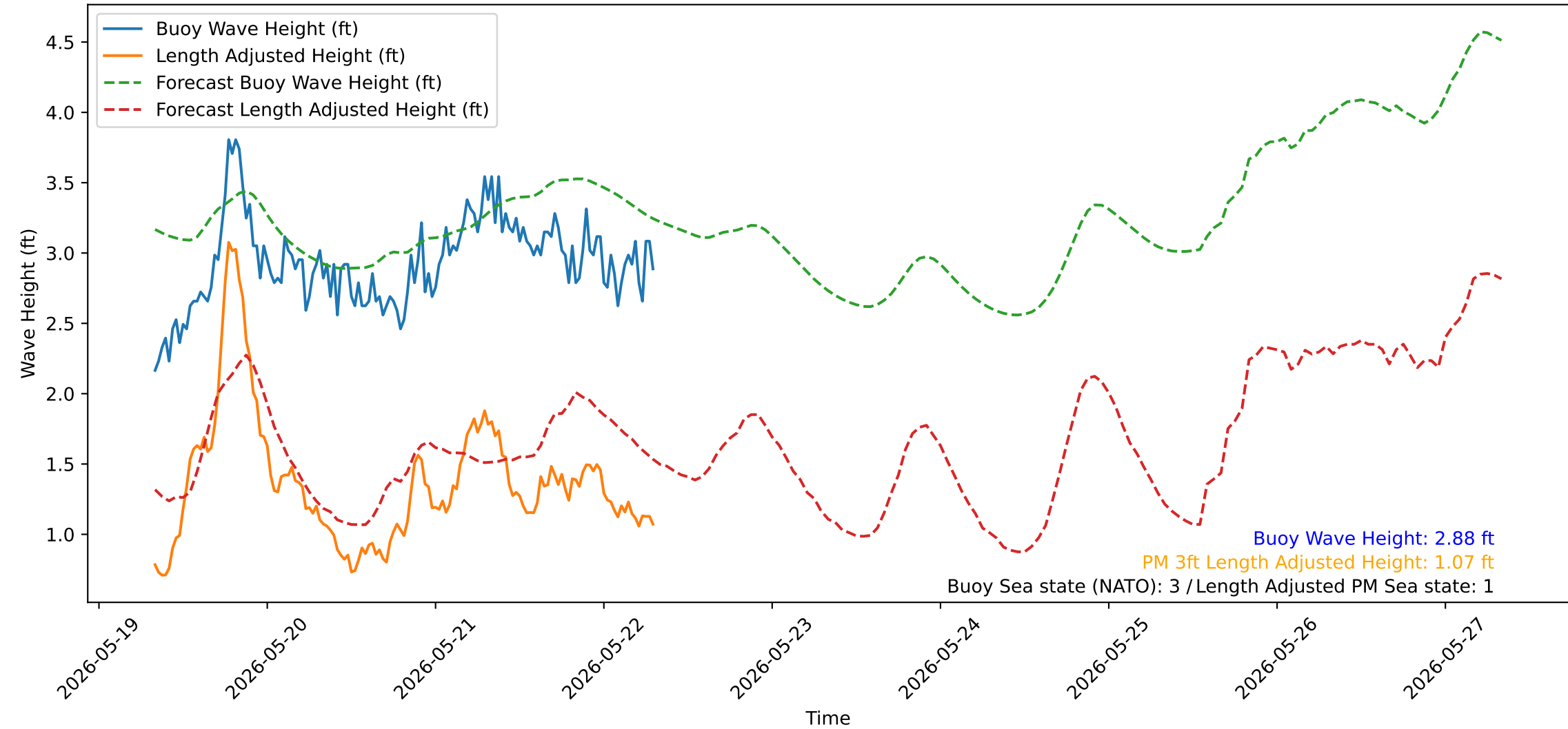
Wave Heights over Time for Green Beach at 2026-05-22 07:51:14
