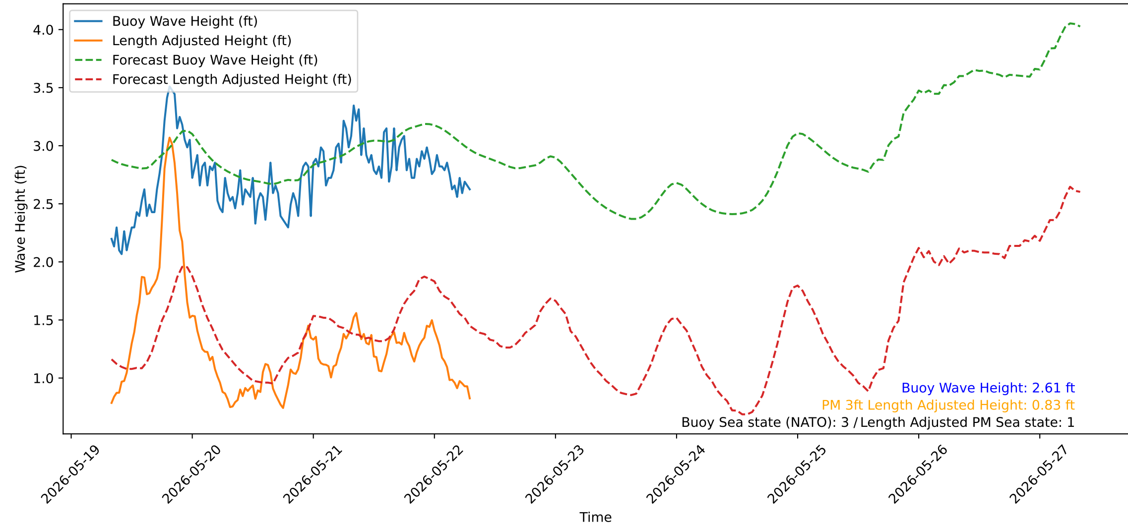
Wave Heights over Time for Red Beach at 2026-05-22 07:50:52
