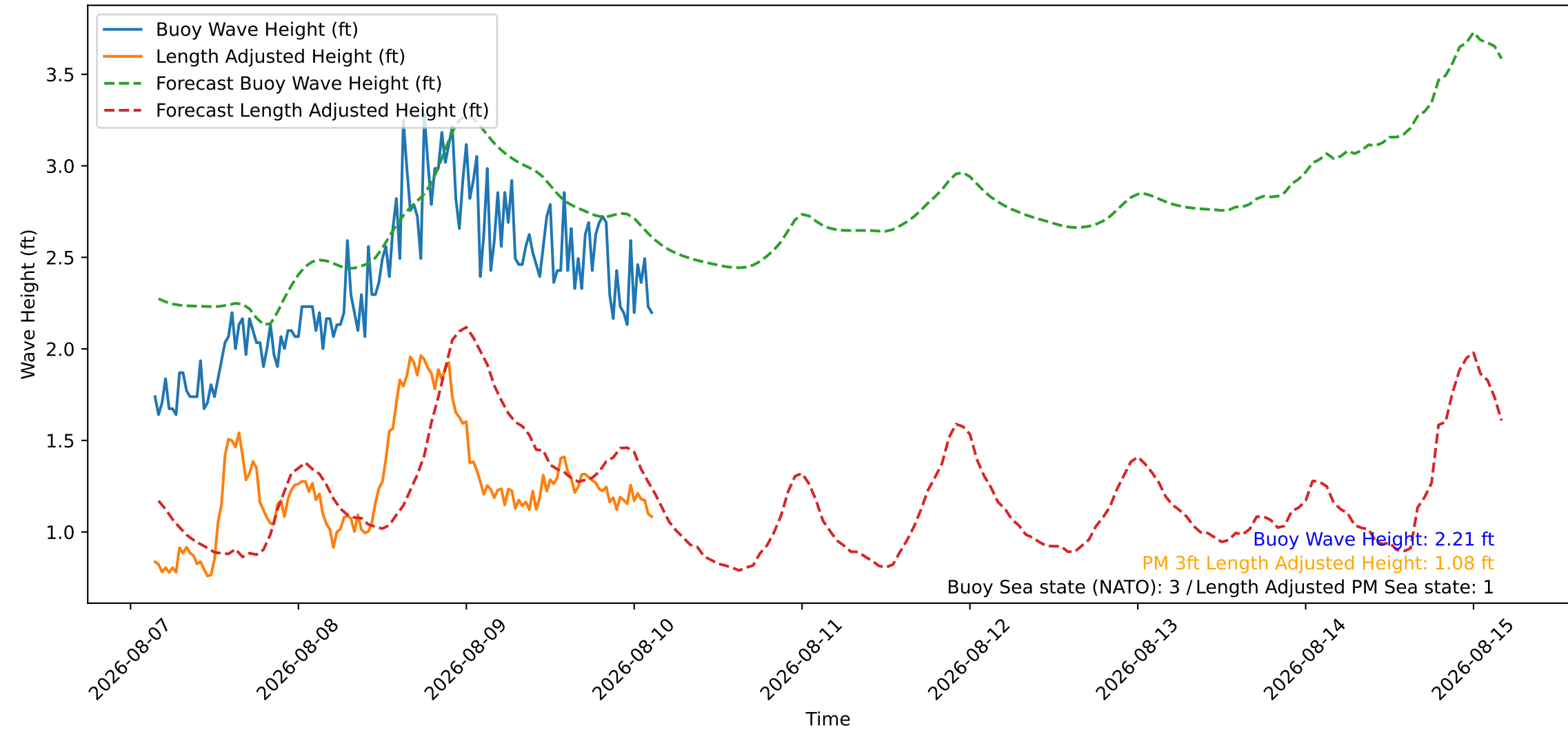
Wave Heights over Time for Oceanside Harbor at 2026-08-10 03:30:27
