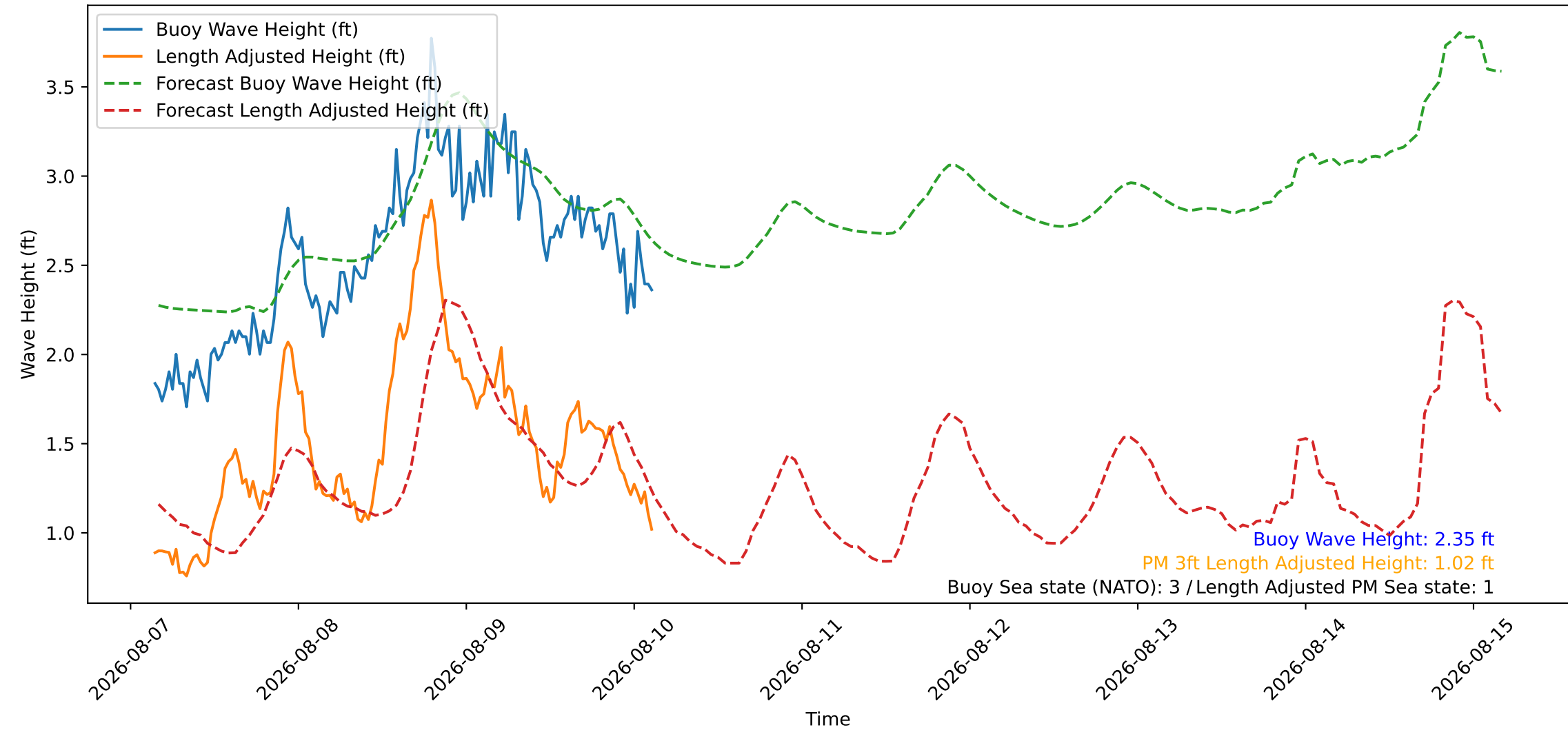
Wave Heights over Time for Green Beach at 2026-08-10 03:31:09
