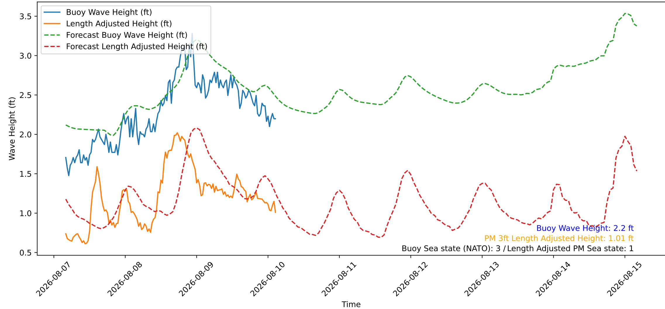
Wave Heights over Time for Red Beach at 2026-08-10 03:30:46
