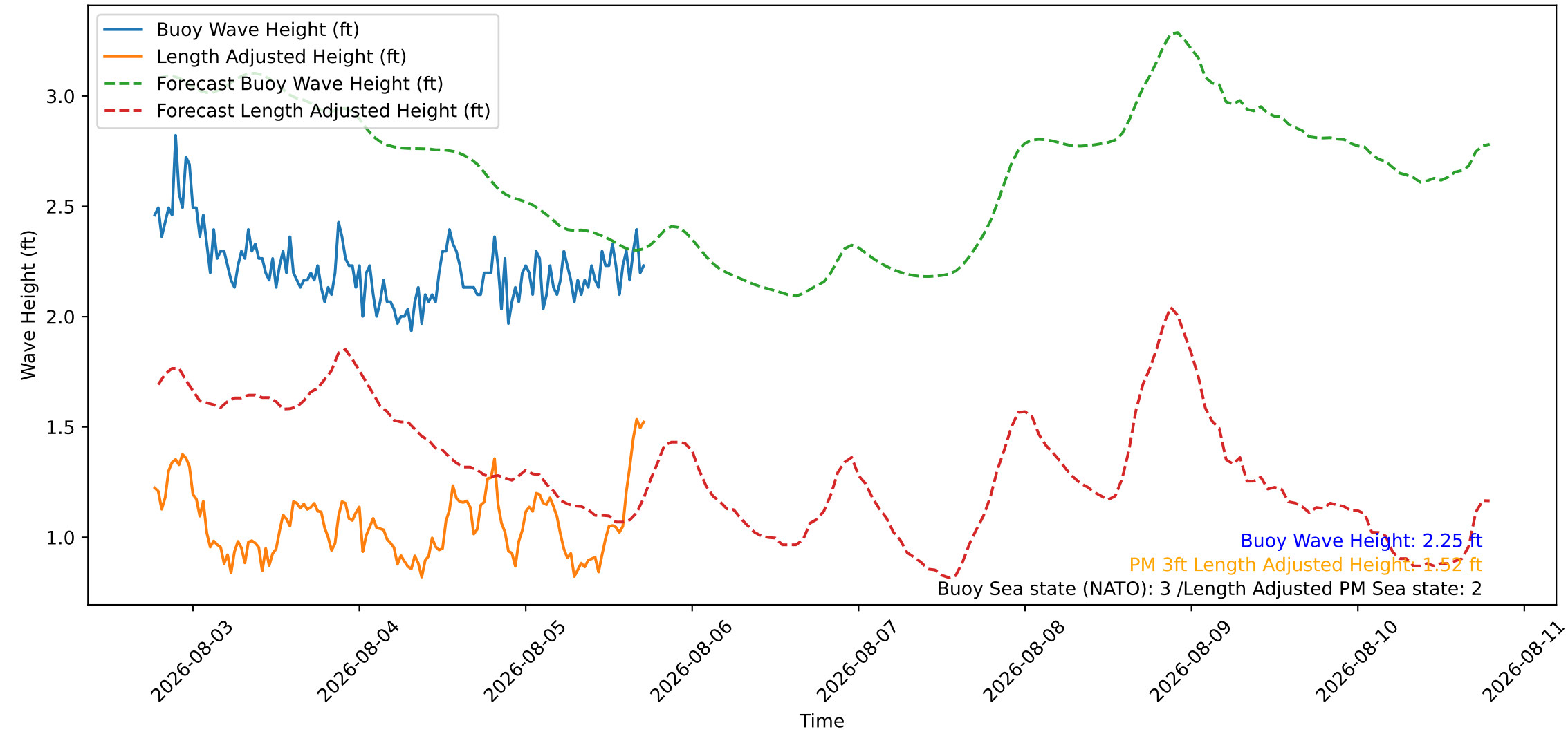
Wave Heights over Time for Green Beach at 2026-08-05 18:31:08
