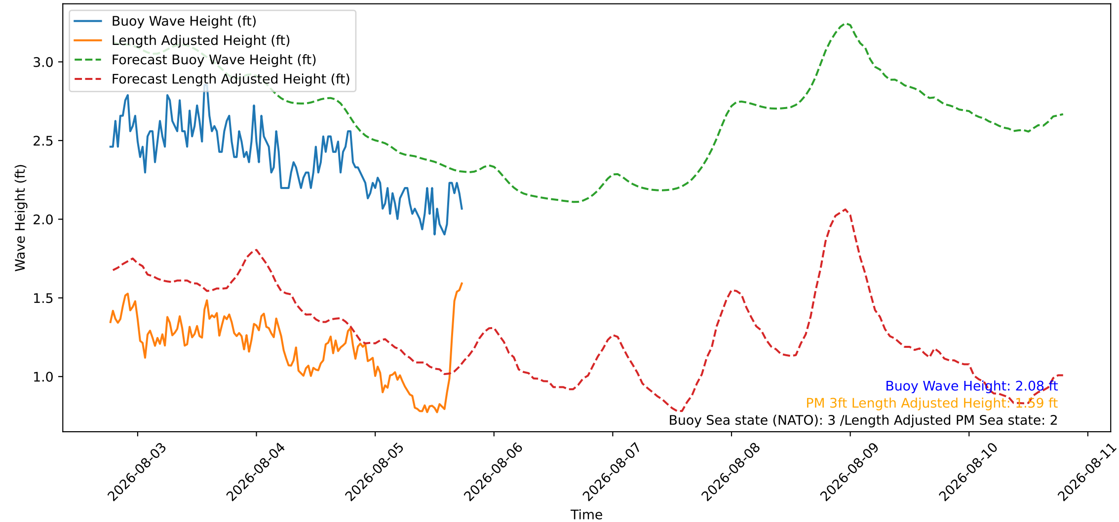
Wave Heights over Time for Oceanside Harbor at 2026-08-05 18:30:26
