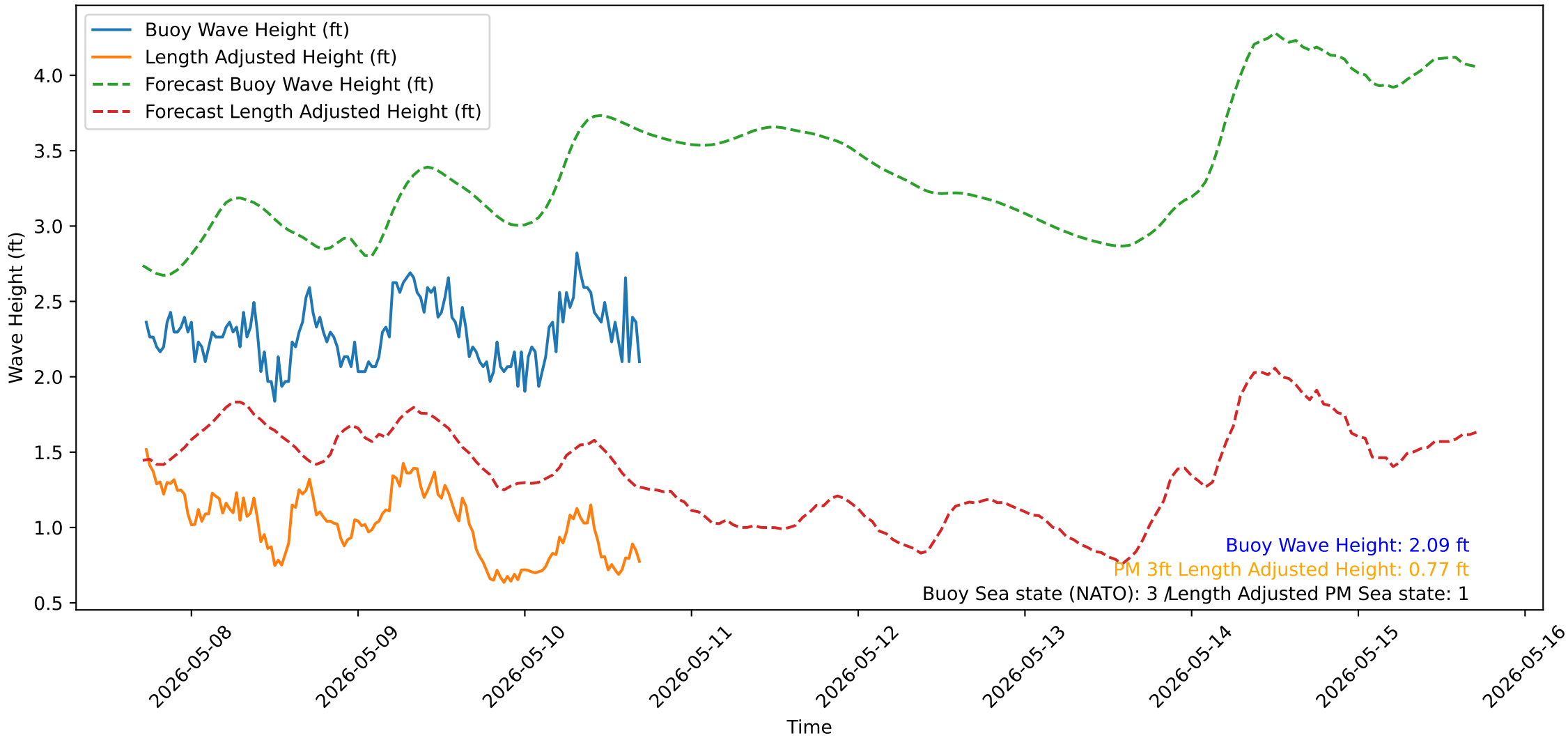
Wave Heights over Time for Green Beach at 2026-05-10 17:21:17
