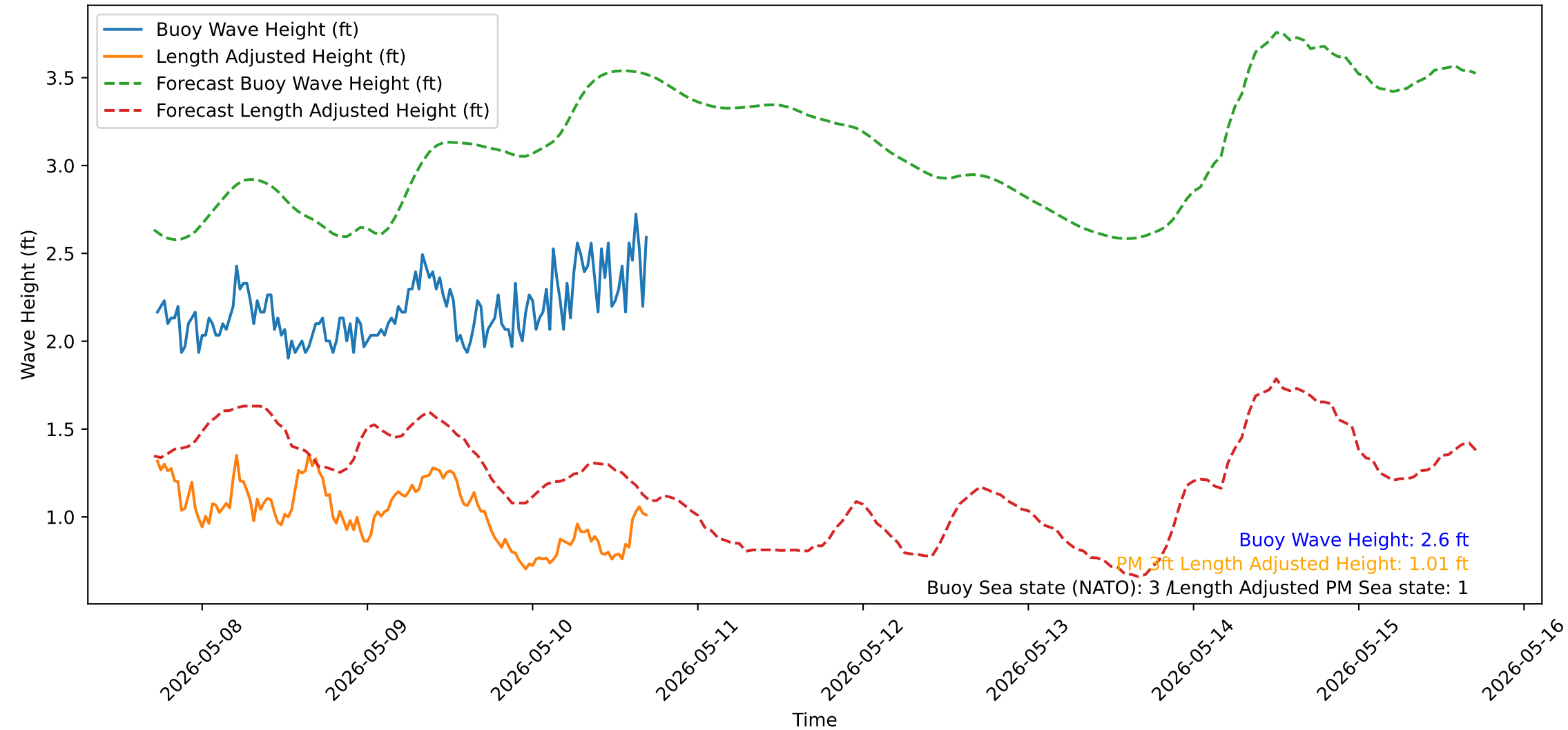
Wave Heights over Time for Red Beach at 2026-05-10 17:20:53
