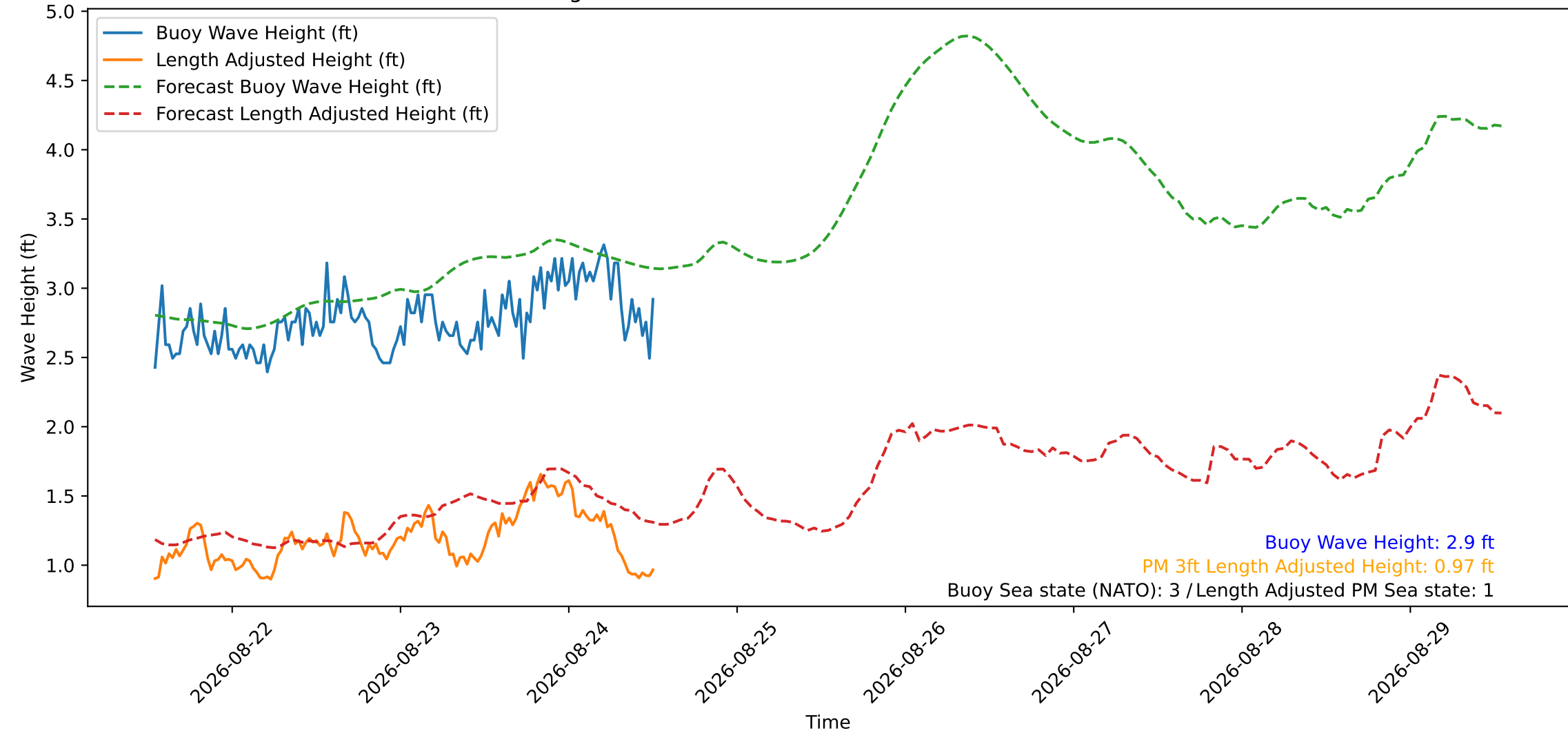
Wave Heights over Time for Green Beach at 2026-08-24 12:51:13
