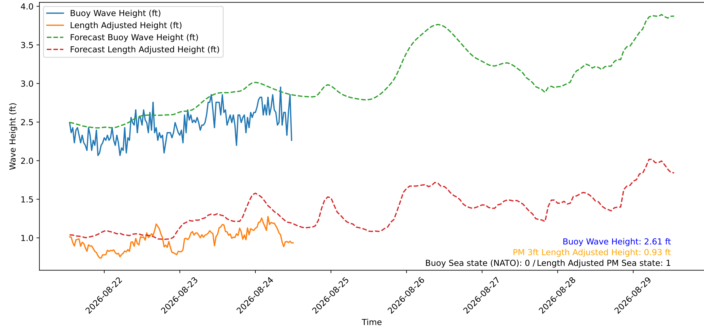
Wave Heights over Time for Red Beach at 2026-08-24 12:50:50
