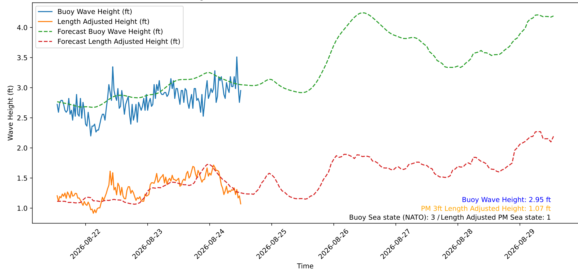
Wave Heights over Time for Oceanside Harbor at 2026-08-24 12:50:29
