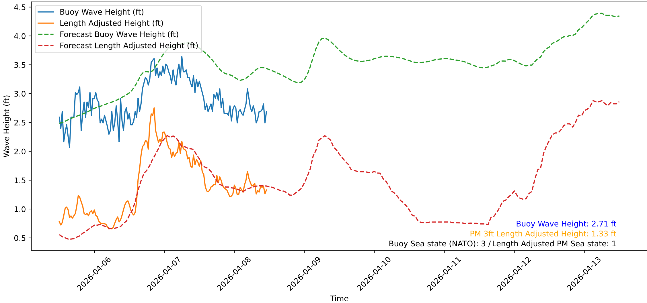
Wave Heights over Time for Oceanside Harbor at 2026-04-08 12:00:31
