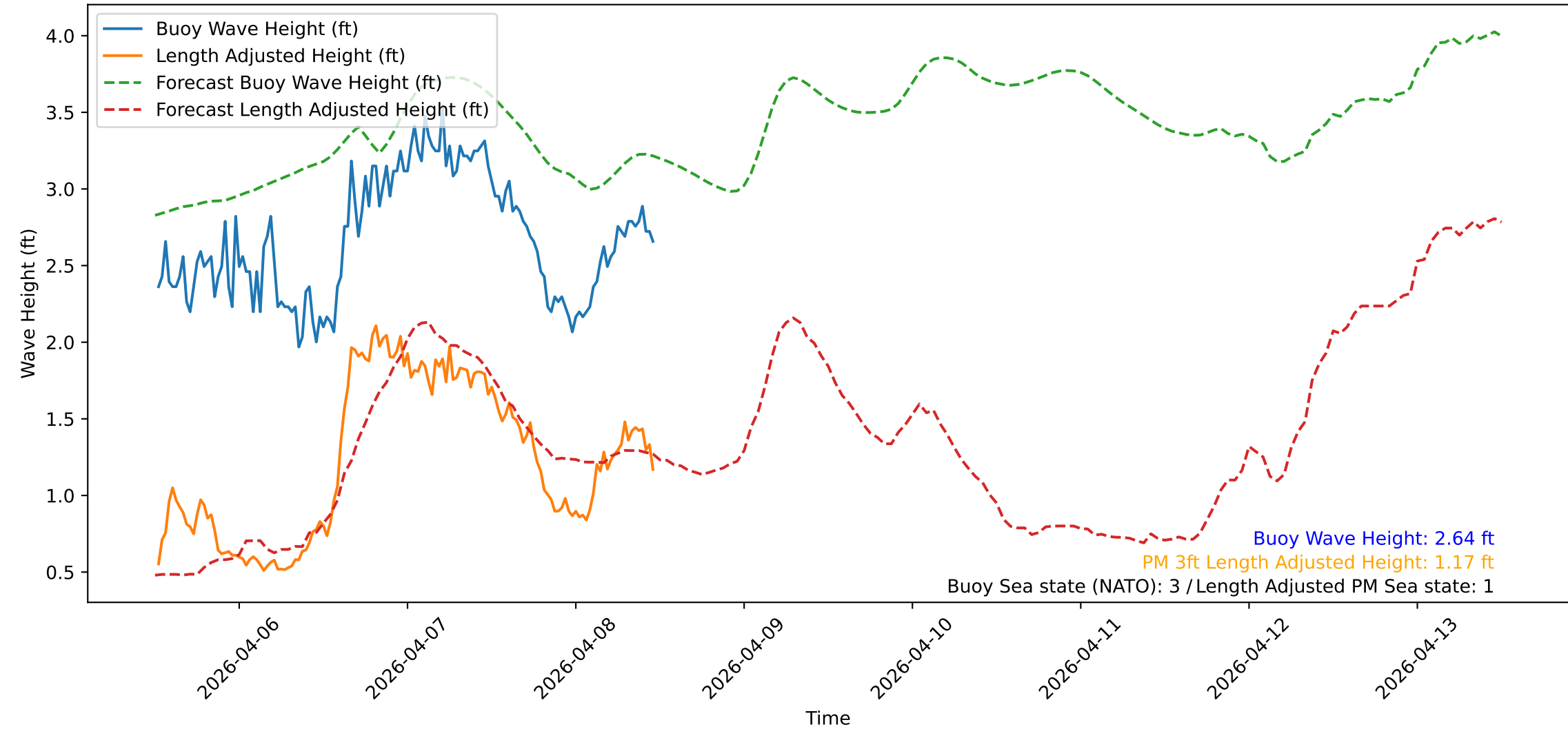
Wave Heights over Time for Red Beach at 2026-04-08 12:00:47
