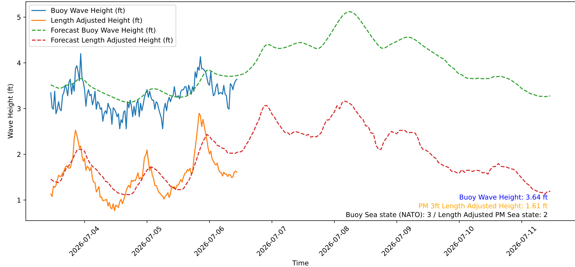
Wave Heights over Time for Green Beach at 2026-07-06 11:11:09
