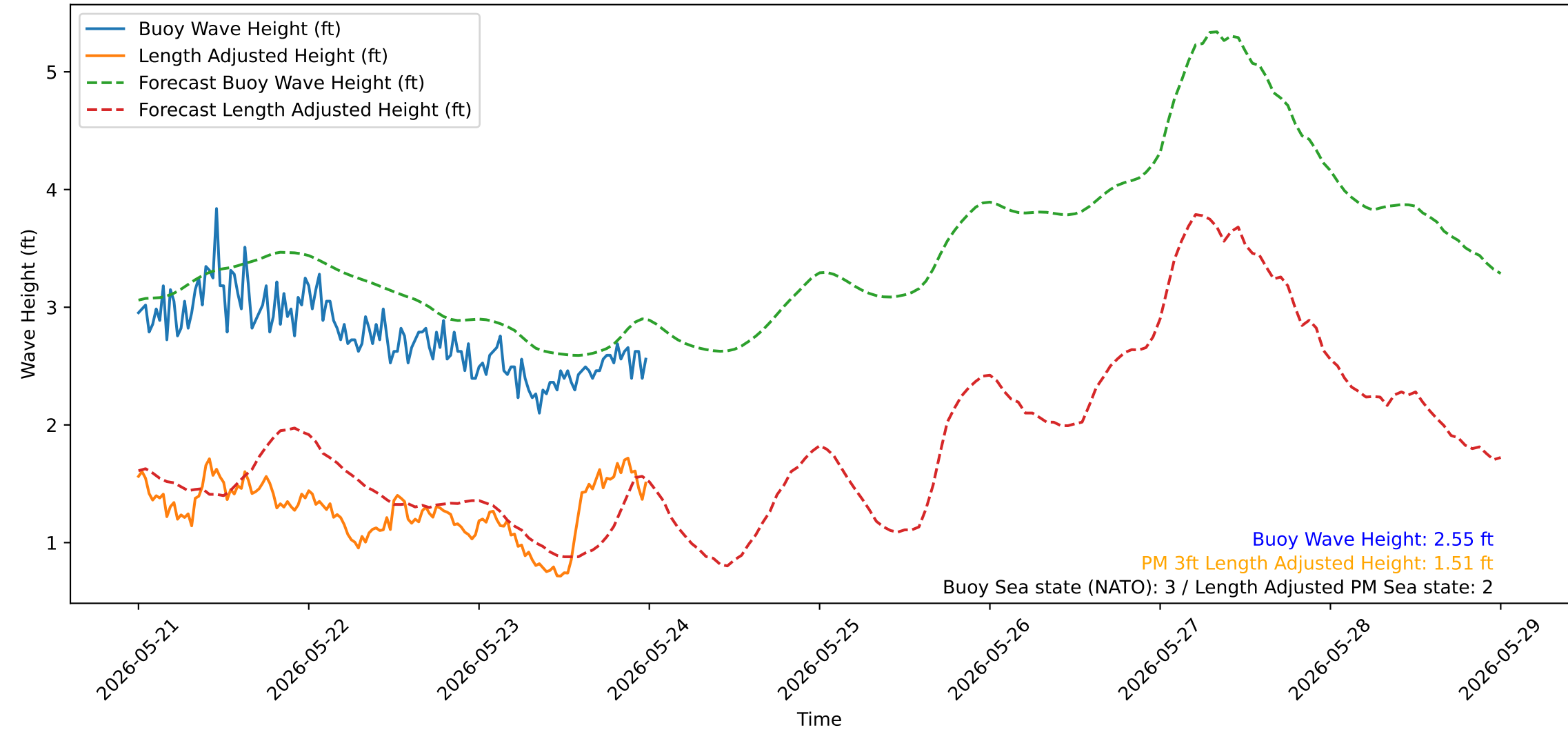
Wave Heights over Time for Oceanside Harbor at 2026-05-24 00:10:31
