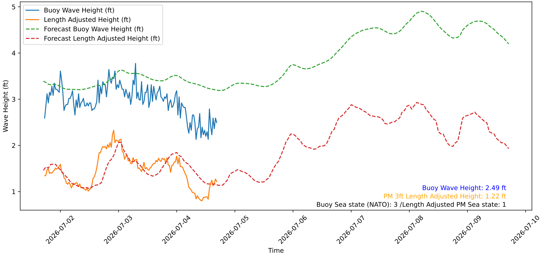
Wave Heights over Time for Oceanside Harbor at 2026-07-04 17:20:27
