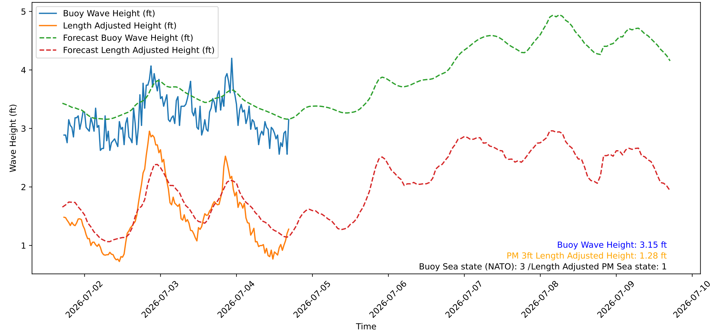
Wave Heights over Time for Green Beach at 2026-07-04 17:21:09
