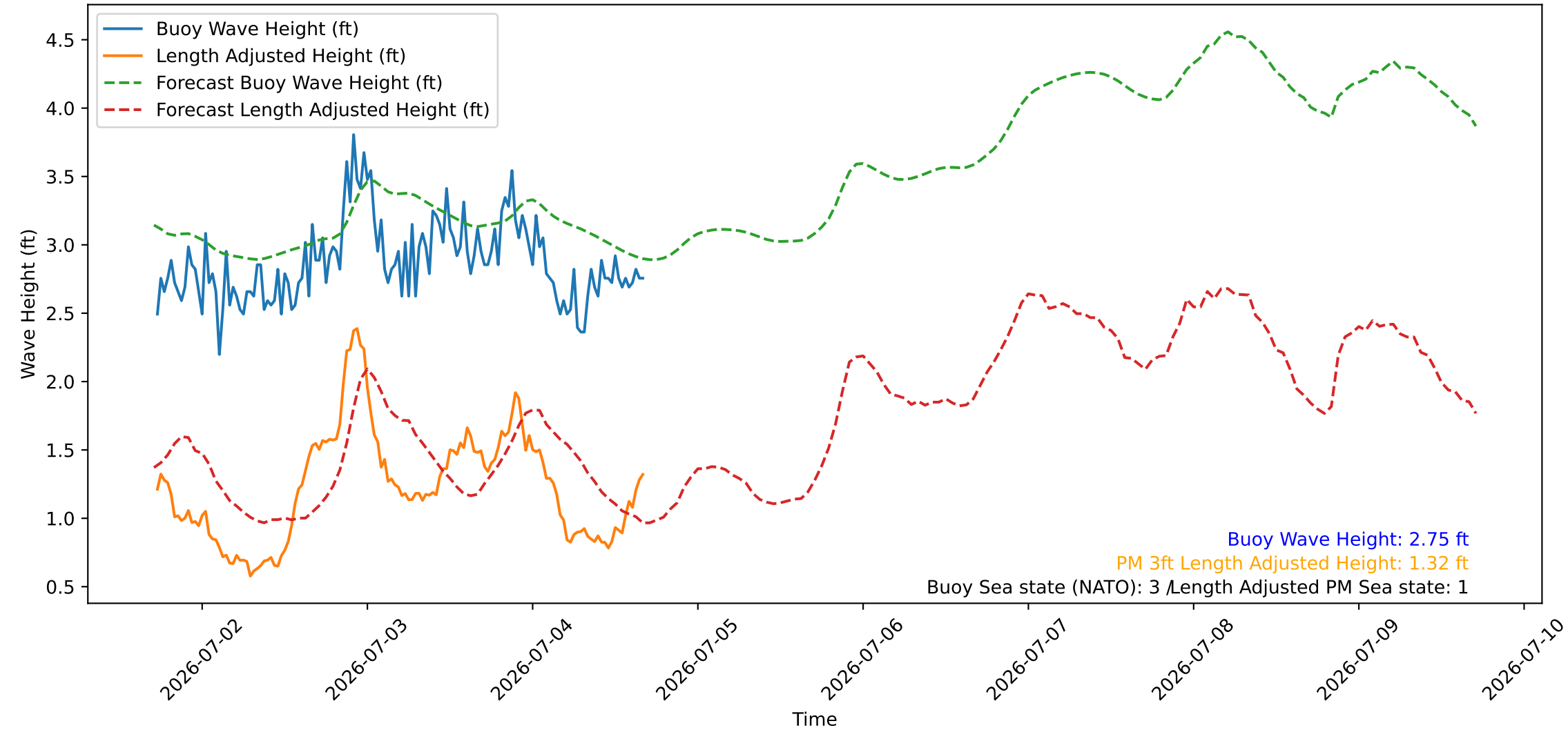
Wave Heights over Time for Red Beach at 2026-07-04 17:20:47
