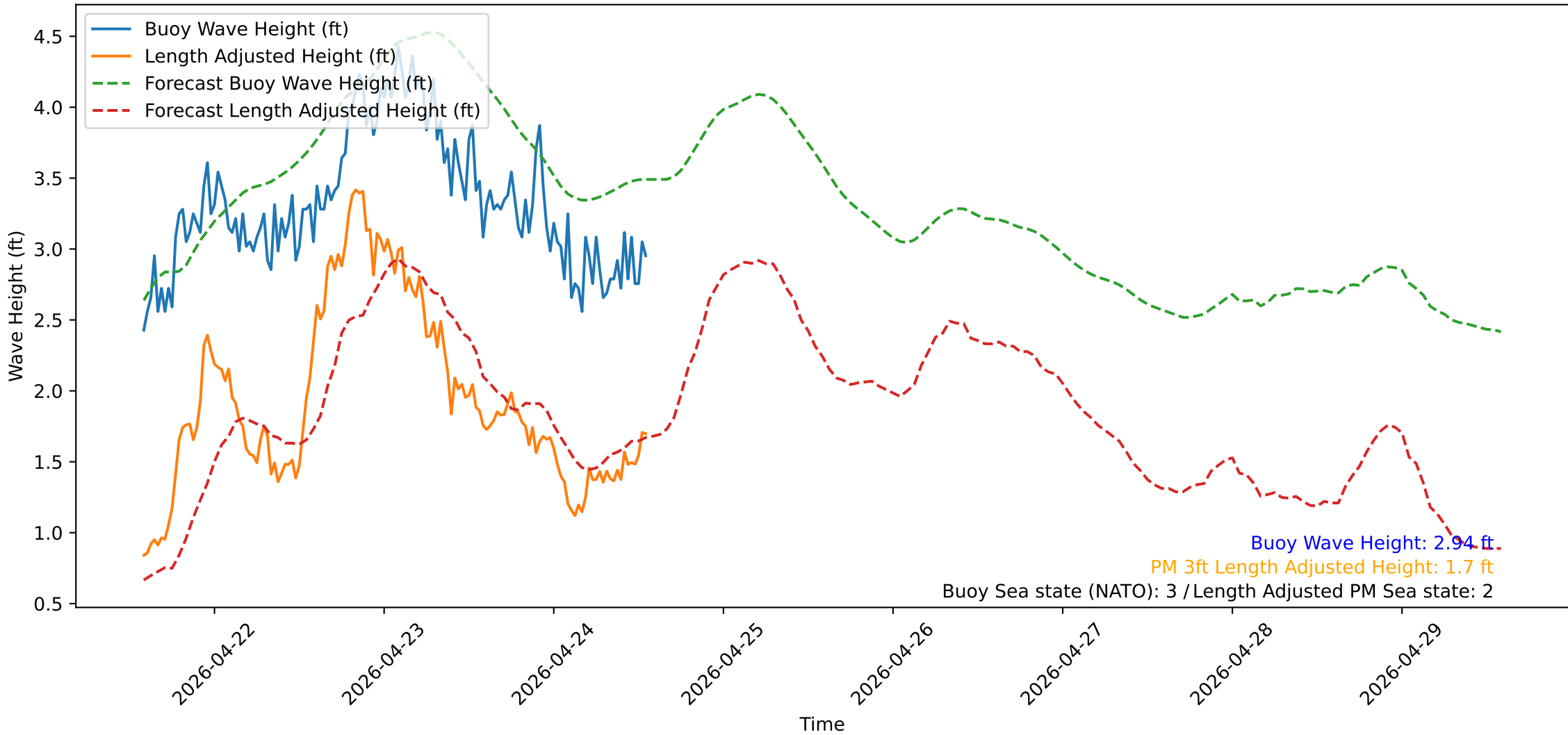
Wave Heights over Time for Oceanside Harbor at 2026-04-24 13:50:31
