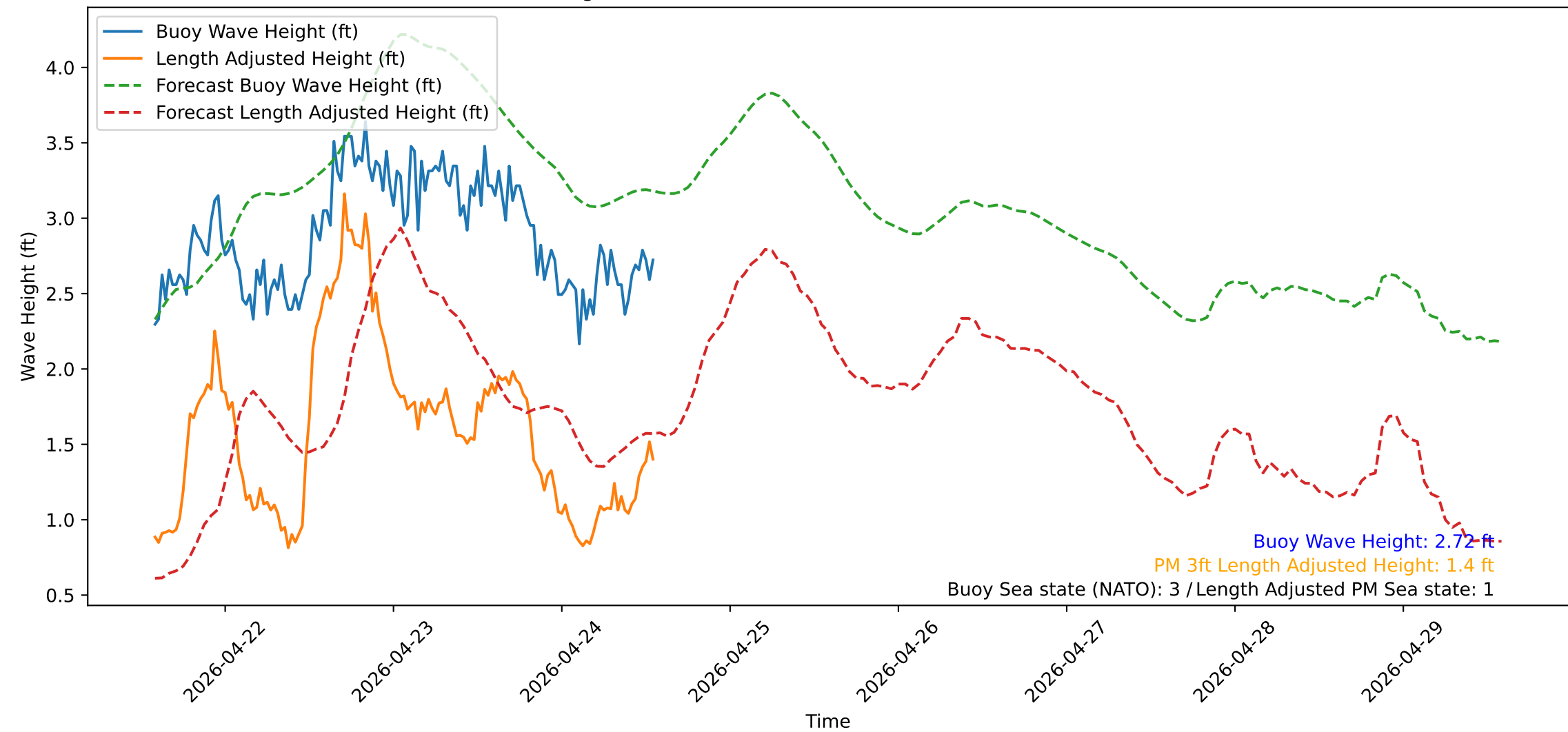
Wave Heights over Time for Red Beach at 2026-04-24 13:50:51
