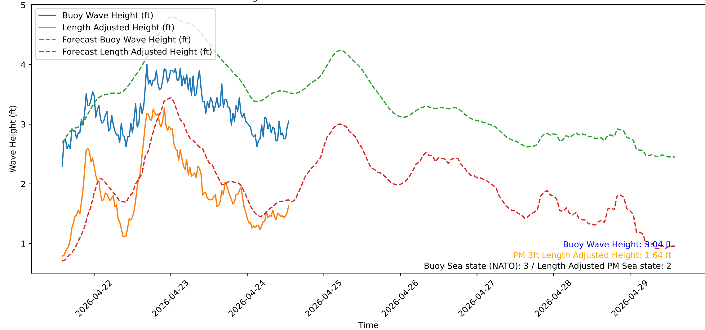
Wave Heights over Time for Green Beach at 2026-04-24 13:51:14
