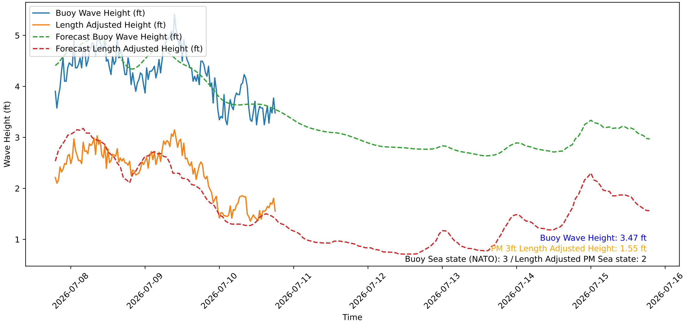
Wave Heights over Time for Oceanside Harbor at 2026-07-10 18:50:26
