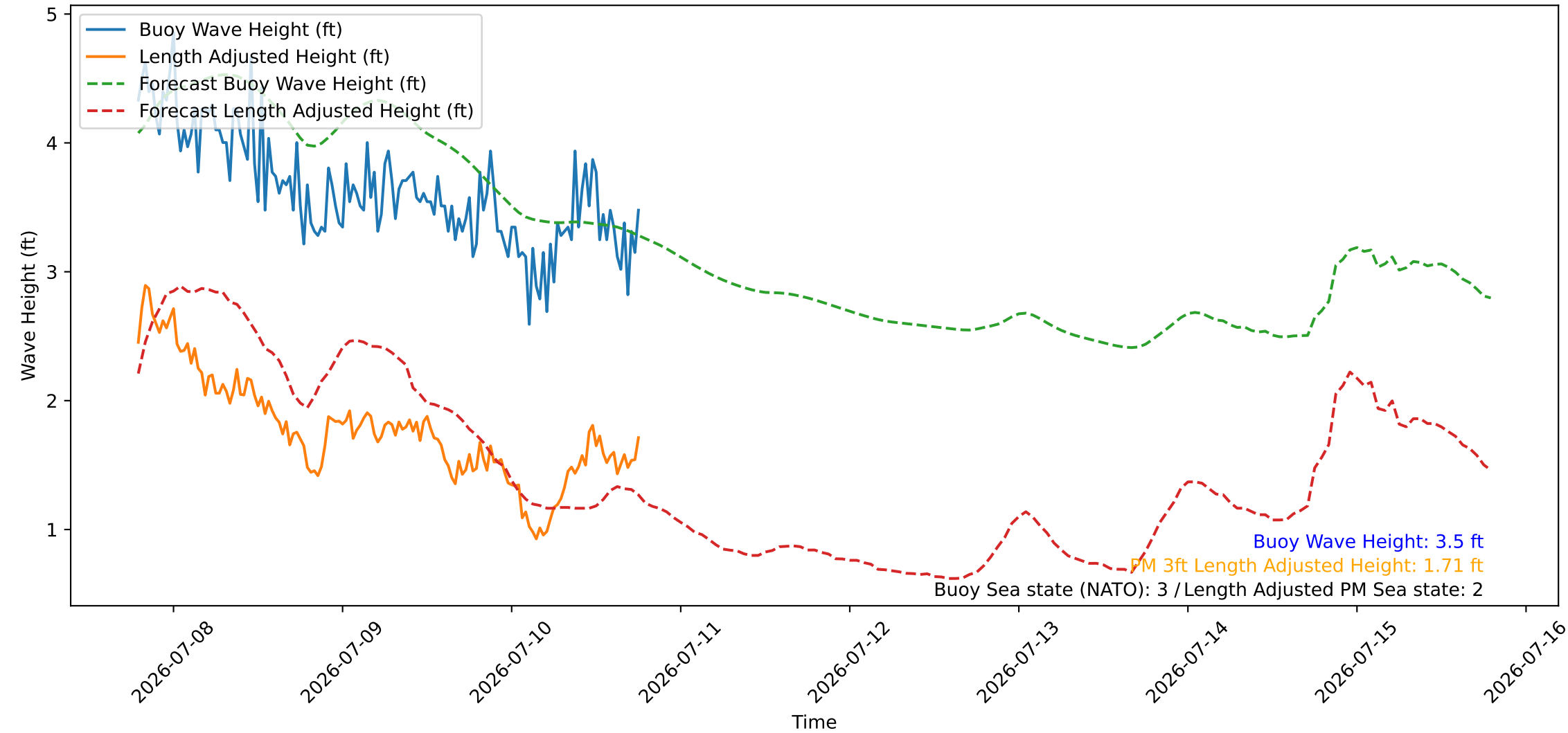
Wave Heights over Time for Red Beach at 2026-07-10 18:50:47
