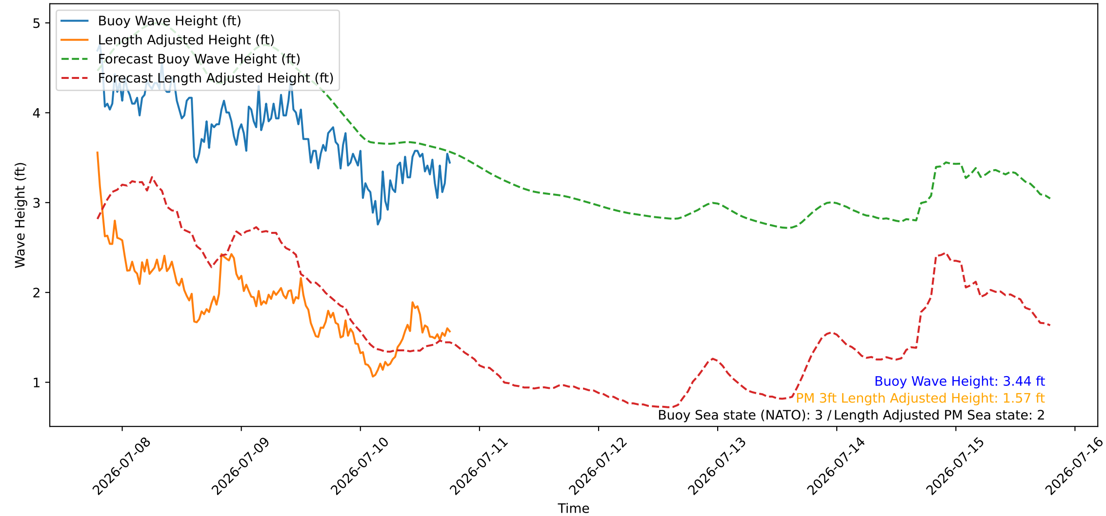
Wave Heights over Time for Green Beach at 2026-07-10 18:51:10
