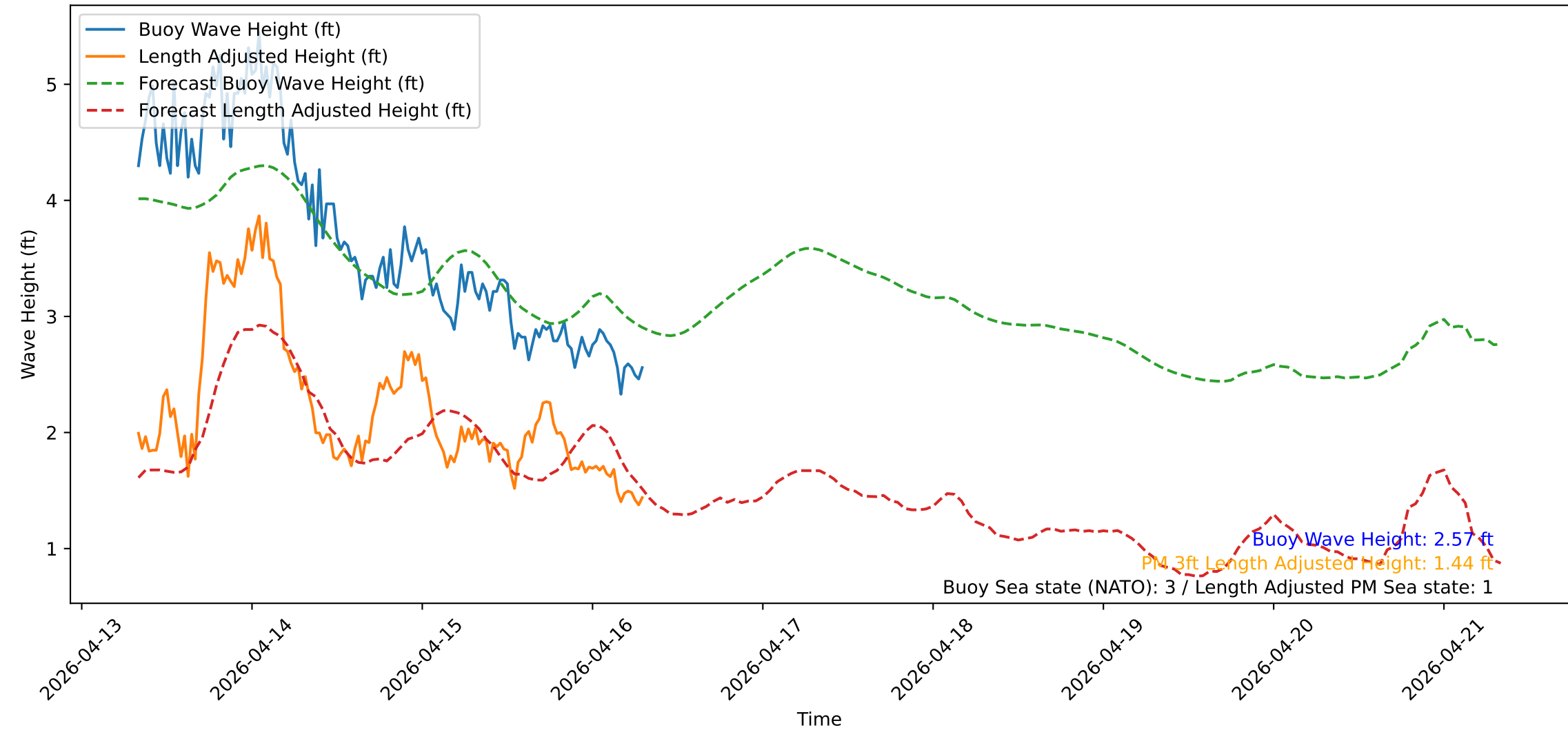
Wave Heights over Time for Oceanside Harbor at 2026-04-16 08:10:31
