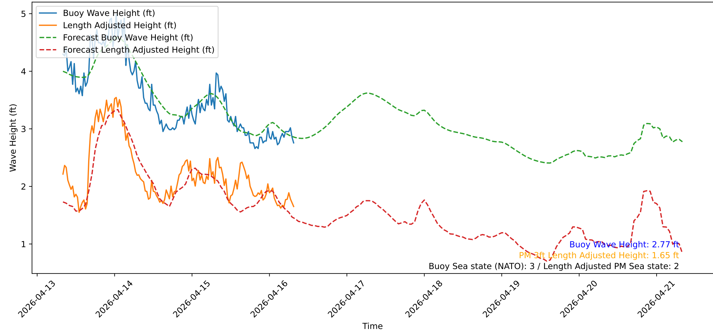
Wave Heights over Time for Green Beach at 2026-04-16 08:11:13
