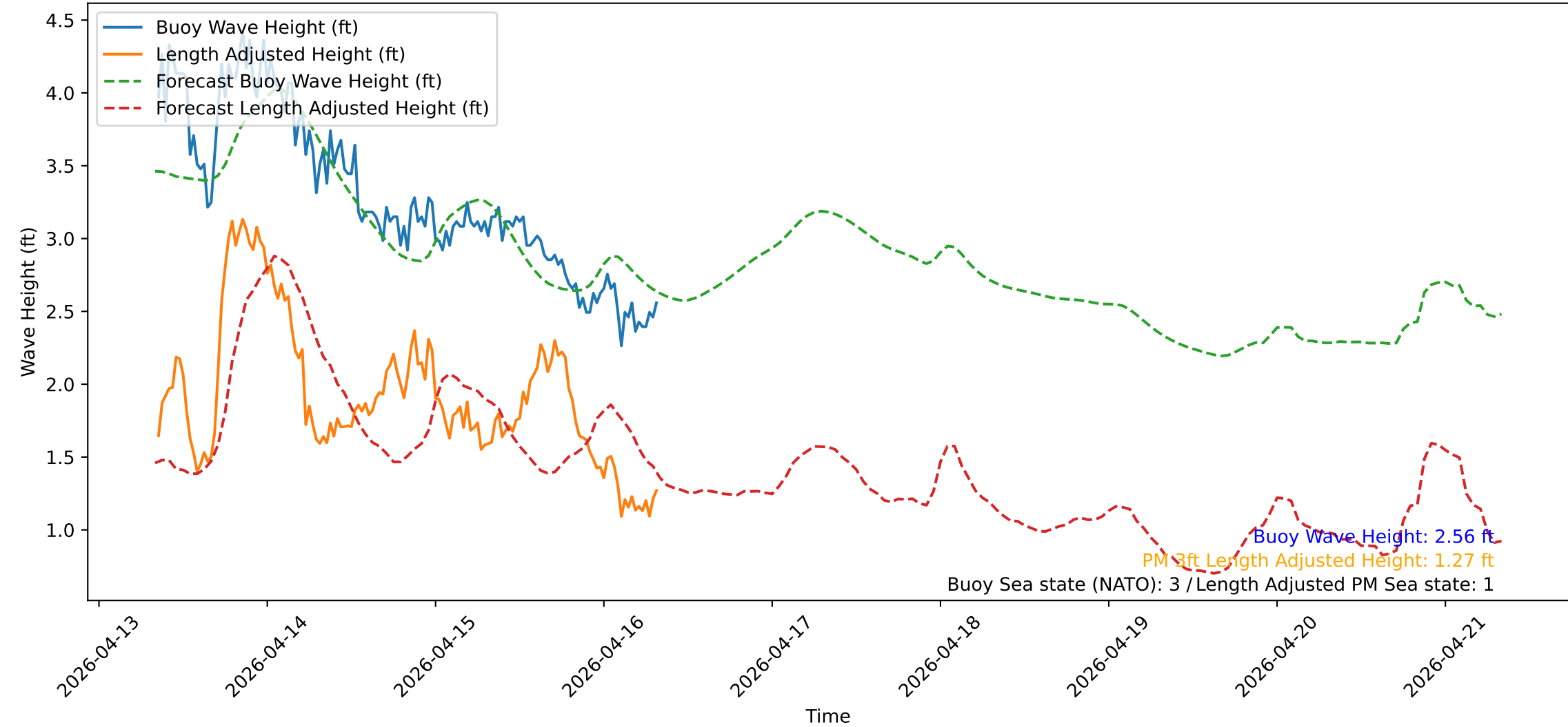
Wave Heights over Time for Red Beach at 2026-04-16 08:10:50
