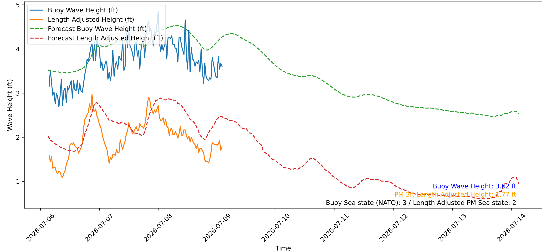
Wave Heights over Time for Red Beach at 2026-07-09 03:00:45
