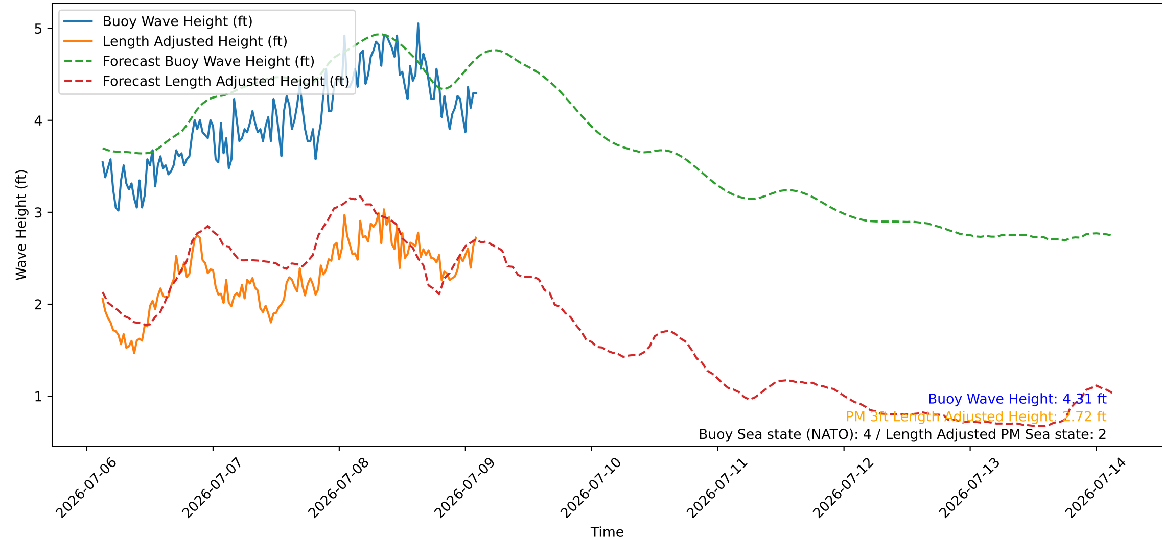
Wave Heights over Time for Oceanside Harbor at 2026-07-09 03:00:26
