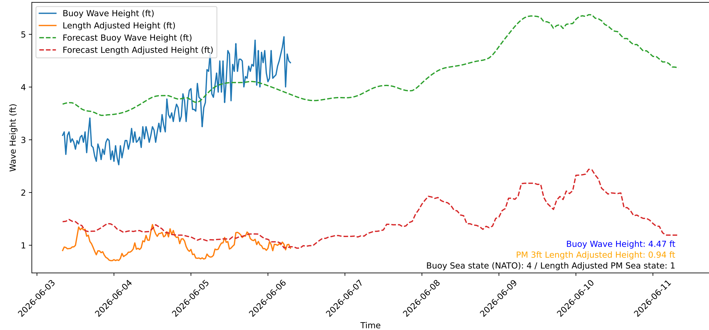
Wave Heights over Time for Red Beach at 2026-06-06 07:50:46
