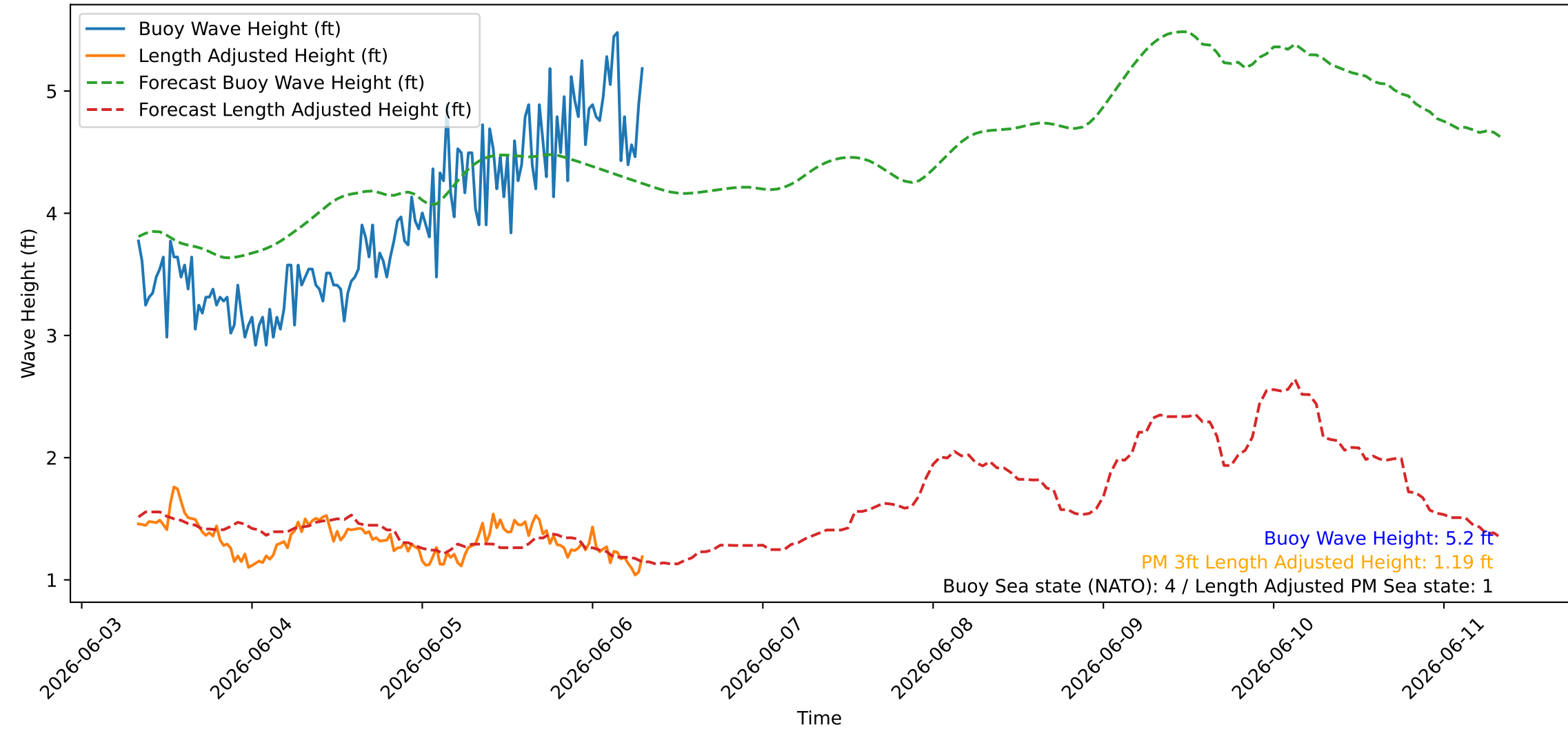
Wave Heights over Time for Oceanside Harbor at 2026-06-06 07:50:26
