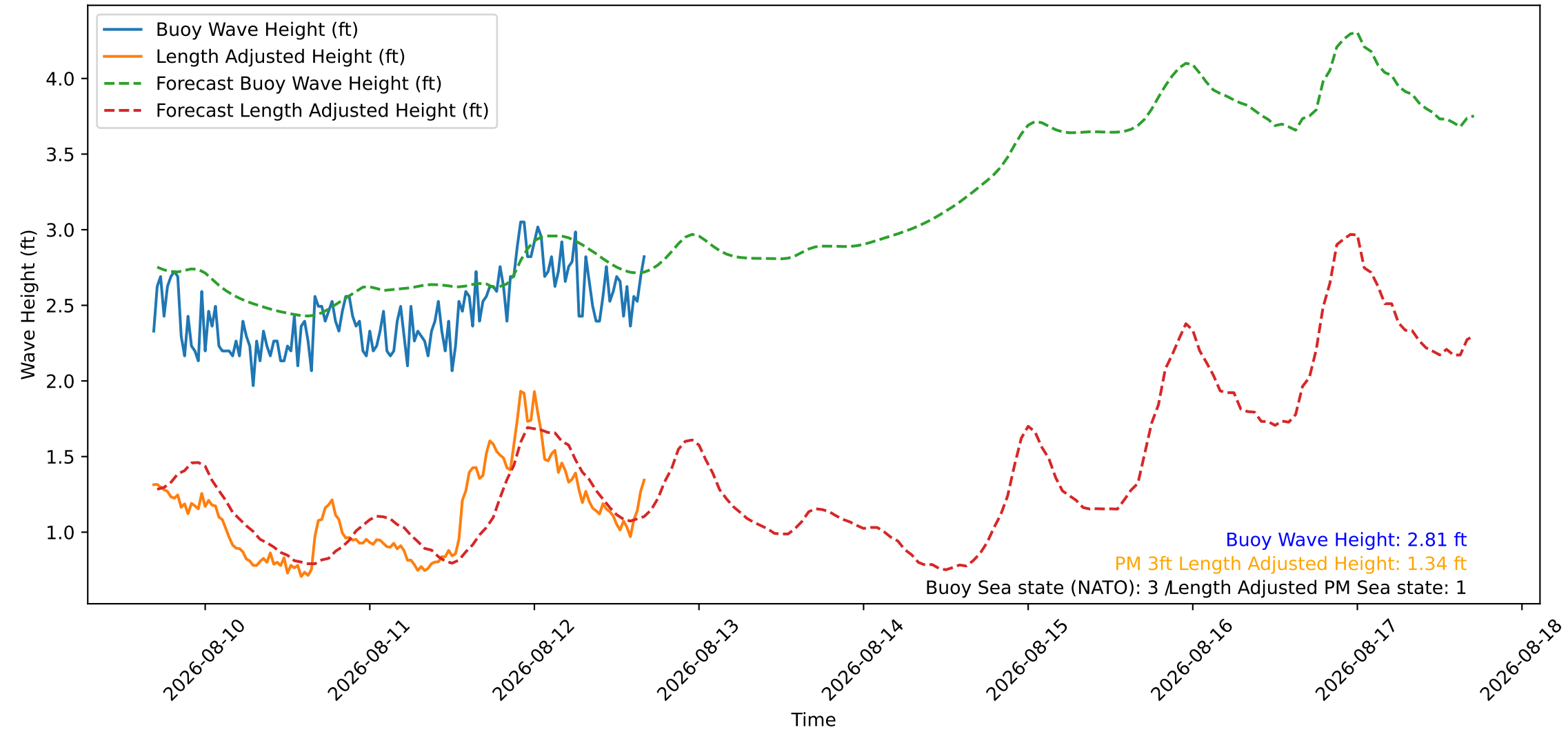
Wave Heights over Time for Oceanside Harbor at 2026-08-12 16:40:27
