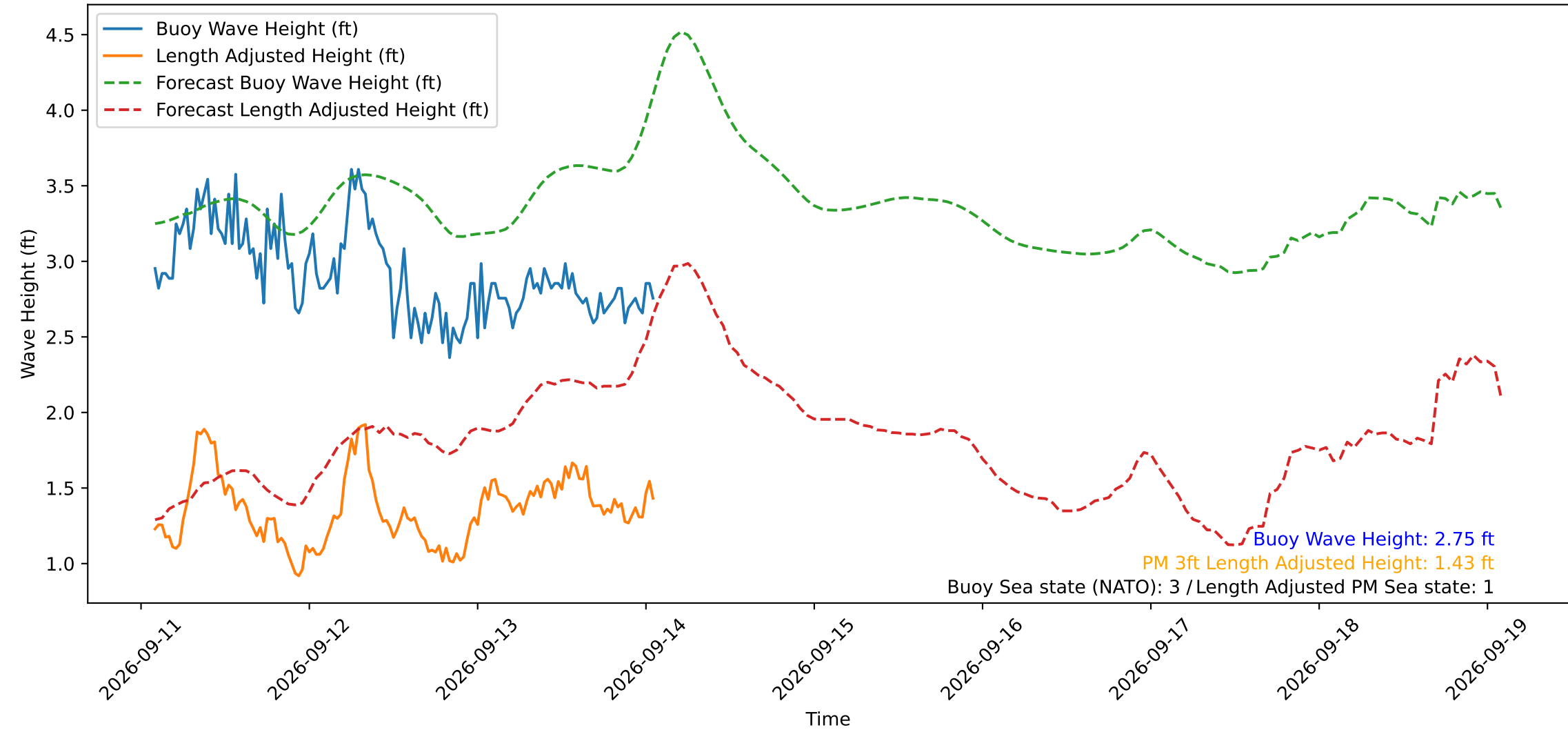
Wave Heights over Time for Green Beach at 2026-09-14 01:51:14
