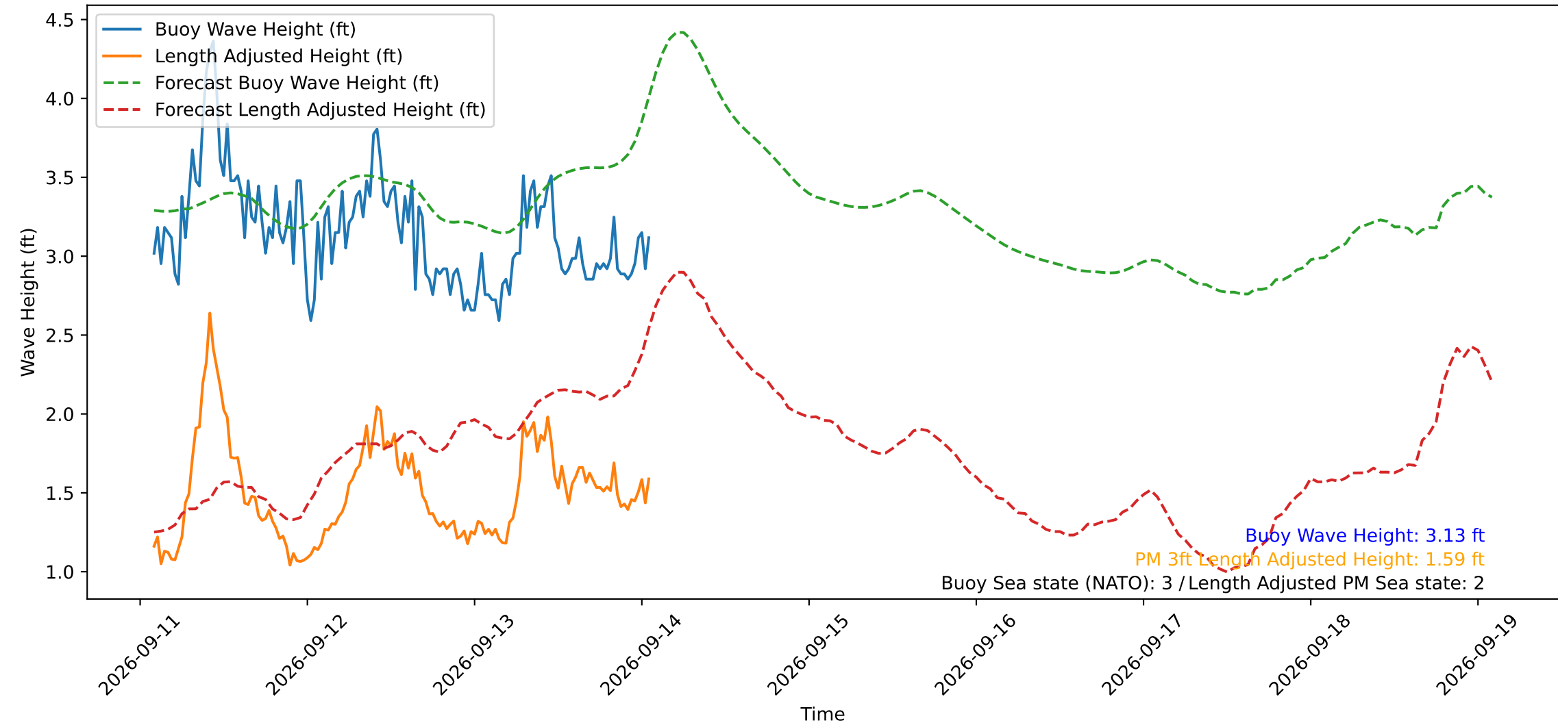
Wave Heights over Time for Oceanside Harbor at 2026-09-14 01:50:29
