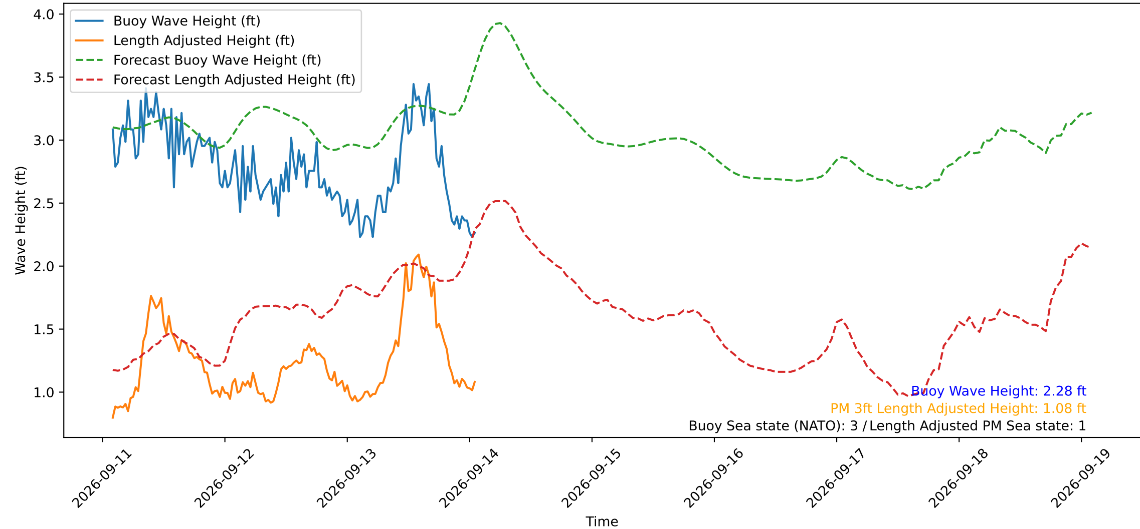
Wave Heights over Time for Red Beach at 2026-09-14 01:50:50
