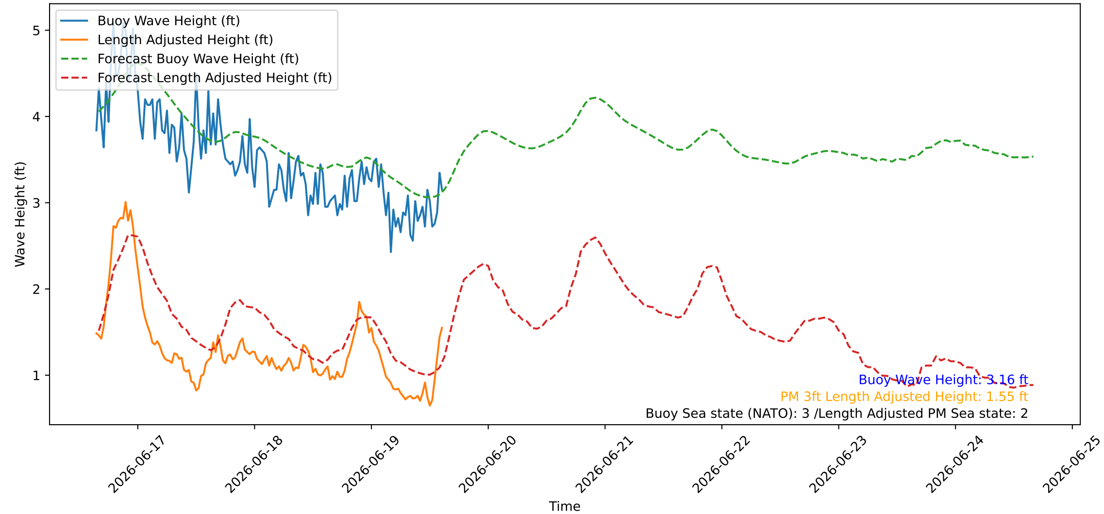
Wave Heights over Time for Green Beach at 2026-06-19 15:31:08
