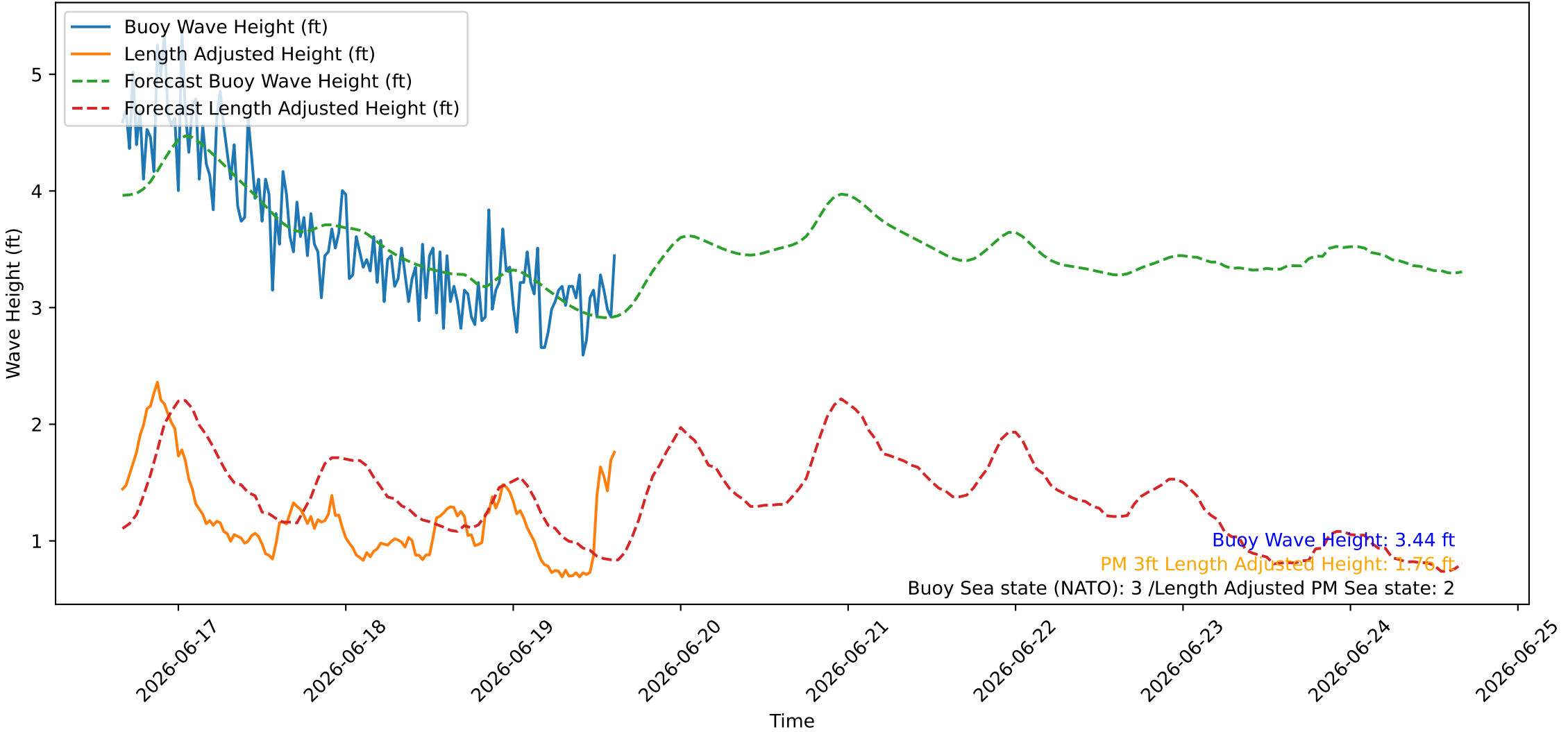
Wave Heights over Time for Red Beach at 2026-06-19 15:30:46
