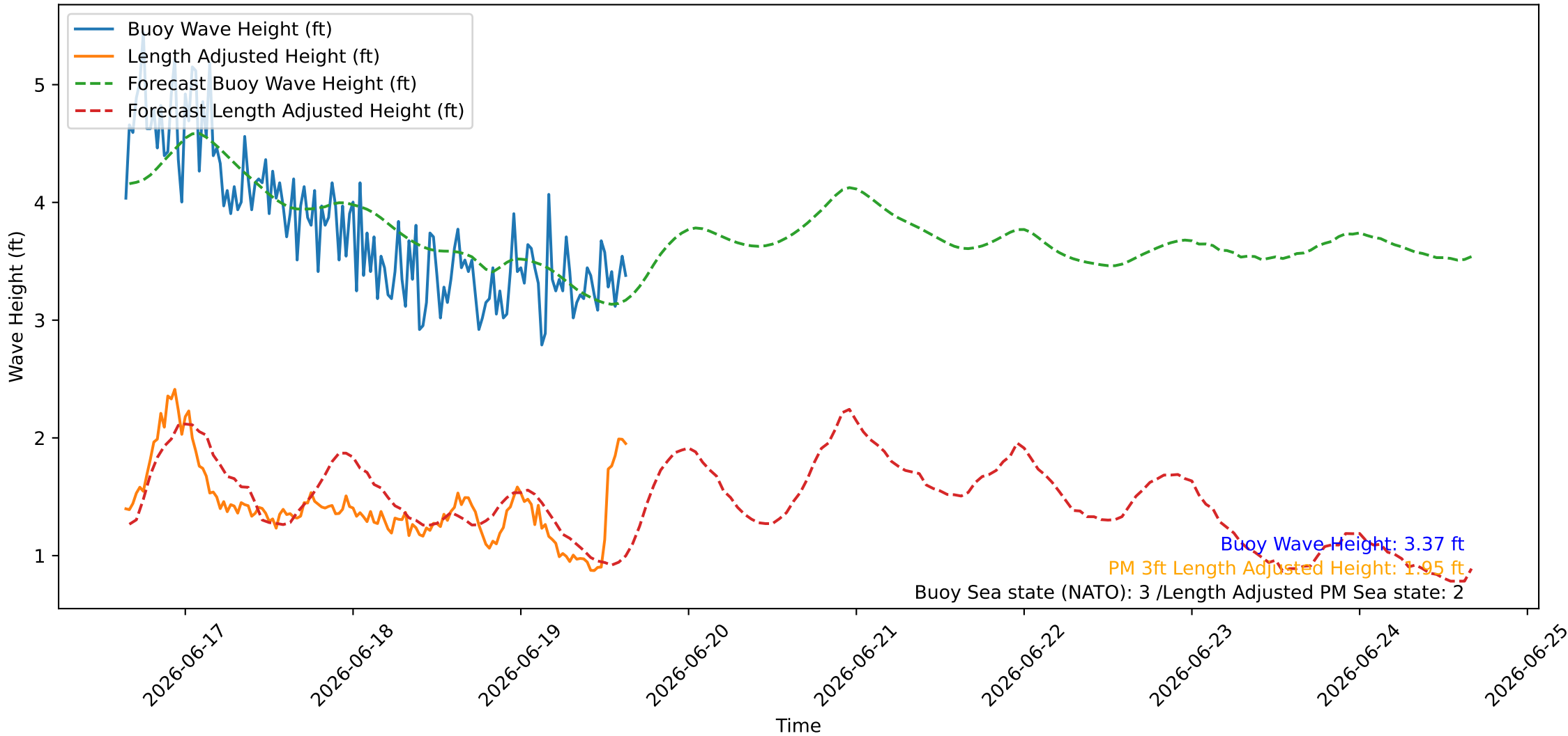
Wave Heights over Time for Oceanside Harbor at 2026-06-19 15:30:26
