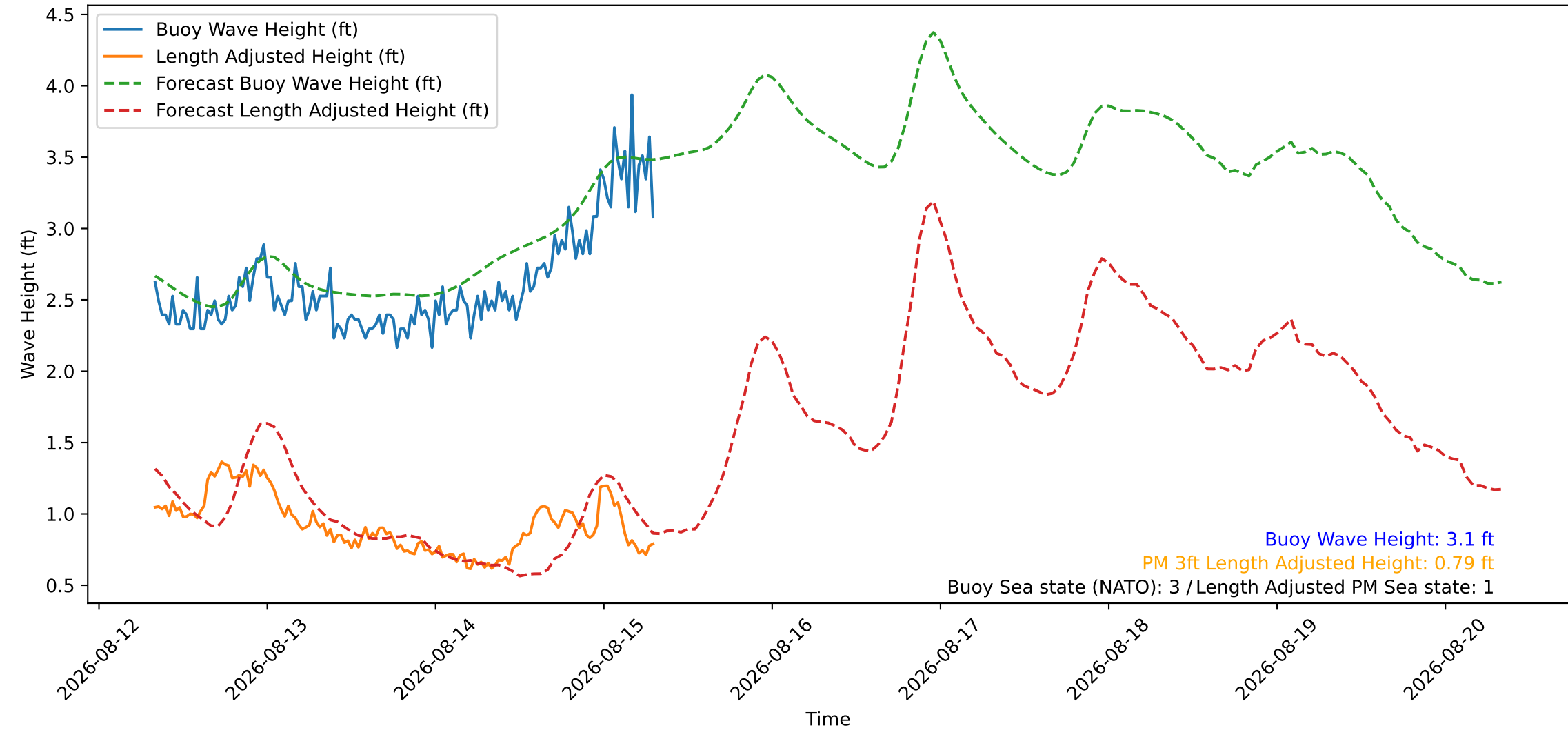
Wave Heights over Time for Red Beach at 2026-08-15 07:50:48
