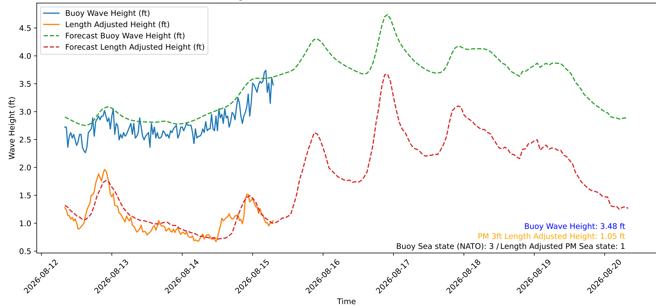
Wave Heights over Time for Green Beach at 2026-08-15 07:51:10
