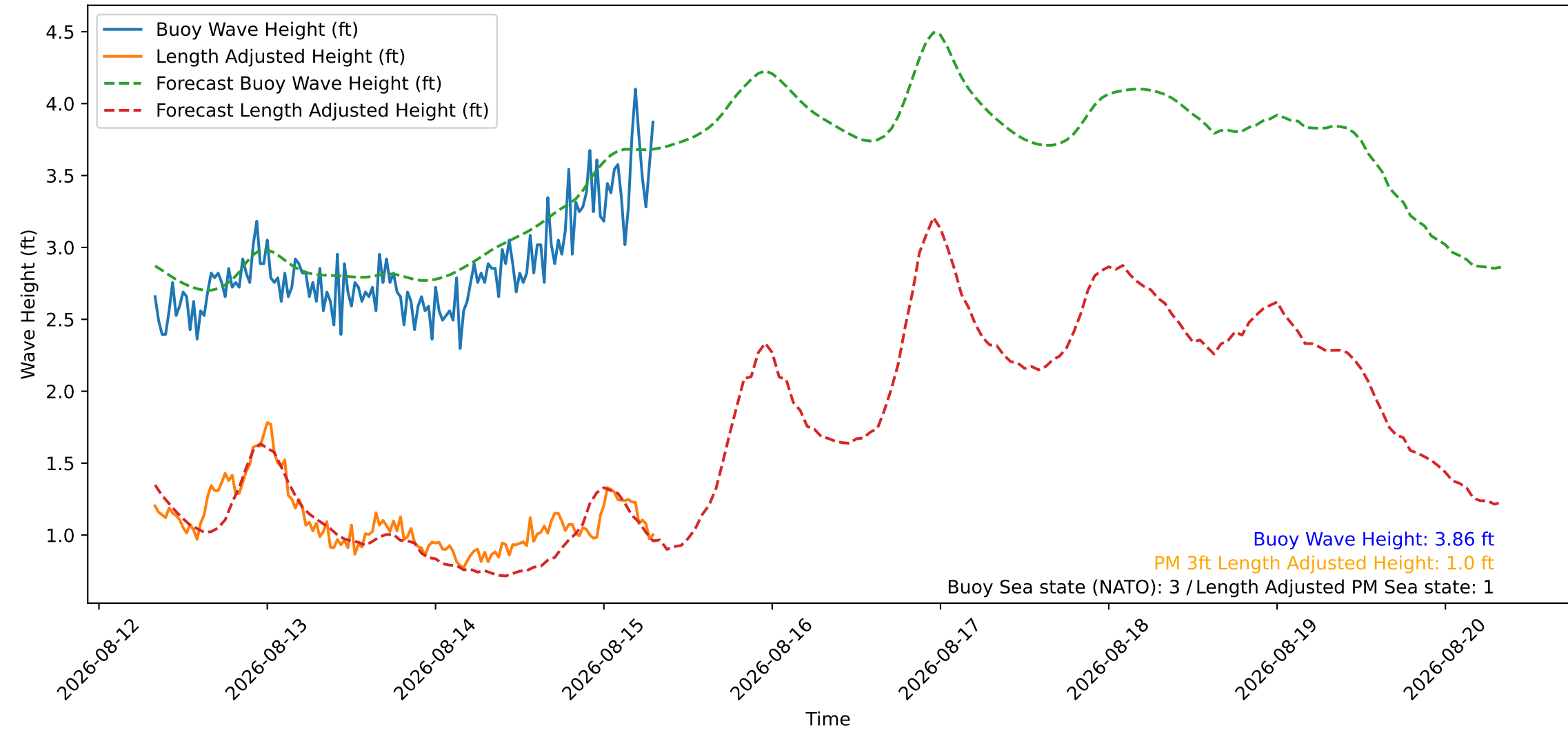
Wave Heights over Time for Oceanside Harbor at 2026-08-15 07:50:27
