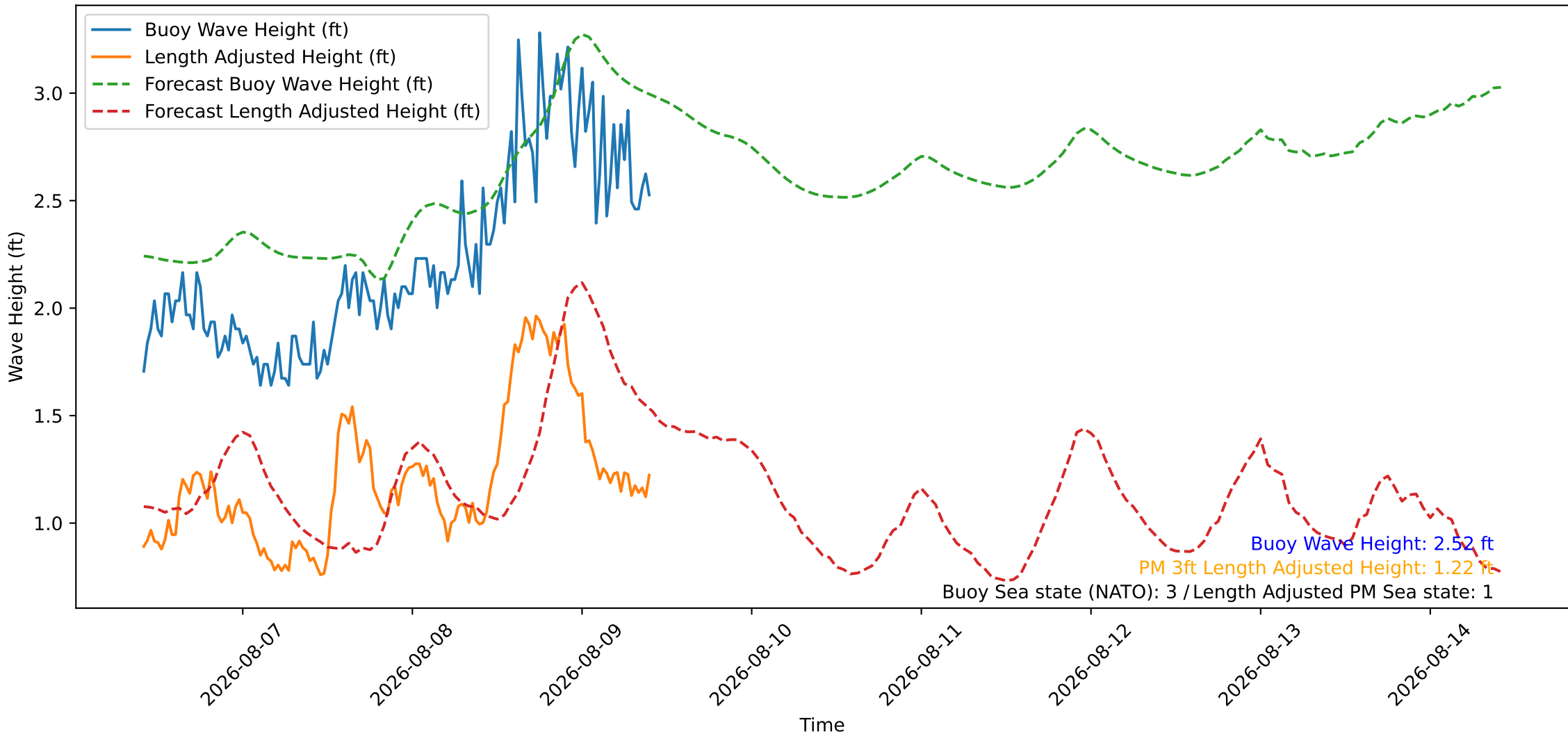
Wave Heights over Time for Oceanside Harbor at 2026-08-09 10:10:27
