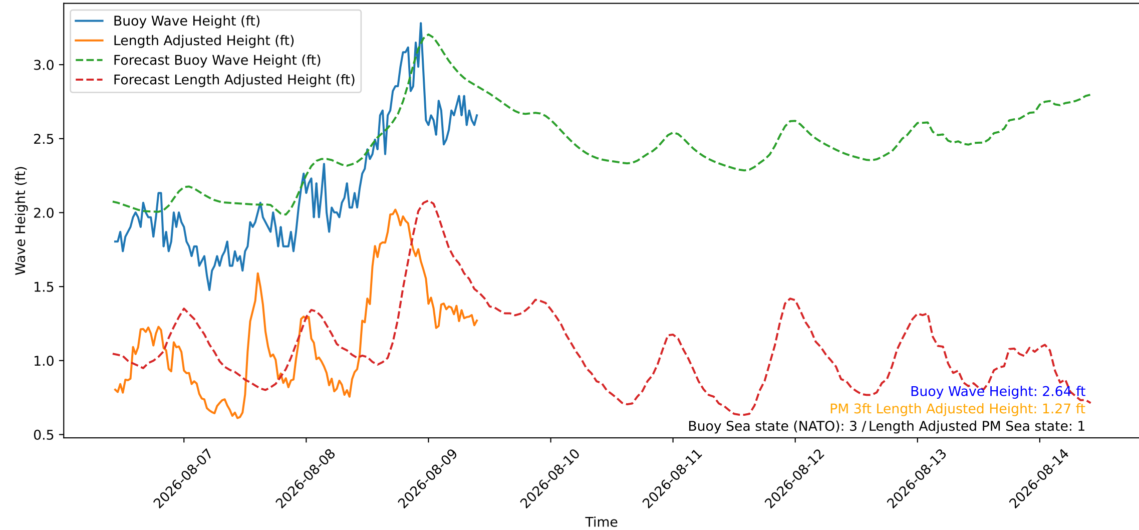
Wave Heights over Time for Red Beach at 2026-08-09 10:10:47
