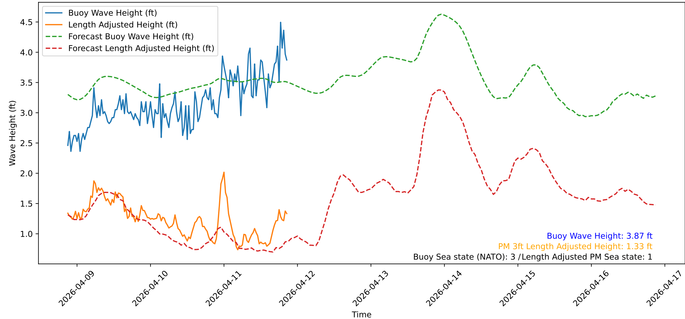
Wave Heights over Time for Green Beach at 2026-04-11 21:11:14
