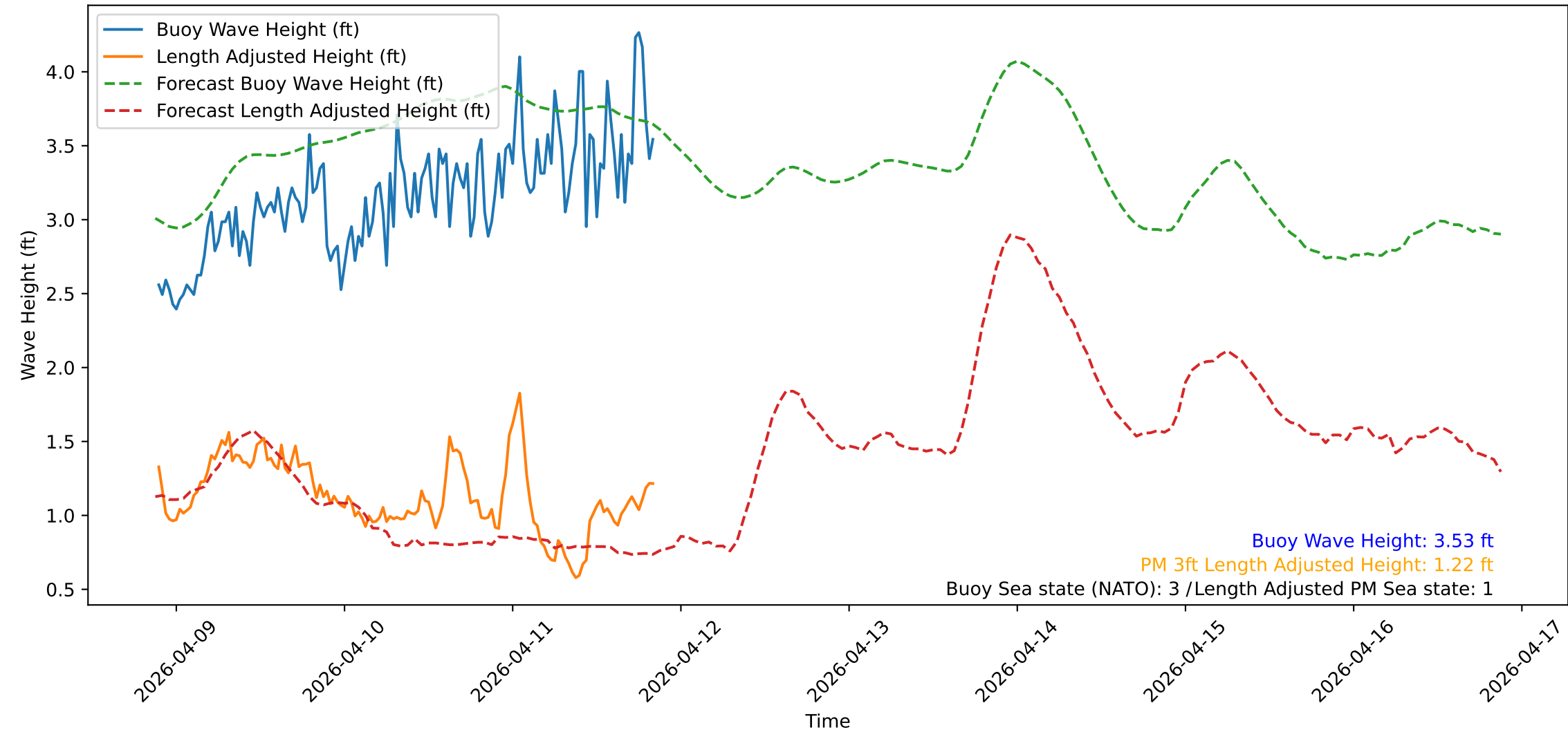
Wave Heights over Time for Red Beach at 2026-04-11 21:10:51
