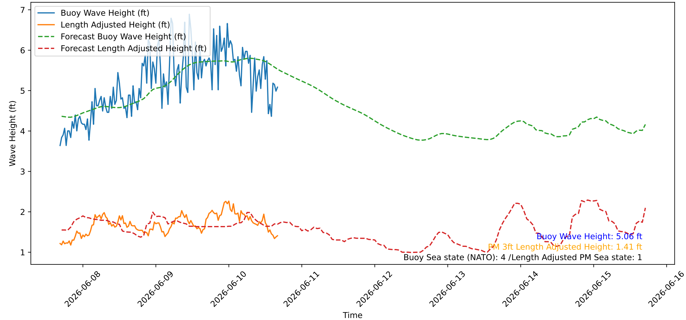
Wave Heights over Time for Green Beach at 2026-06-10 16:41:09
