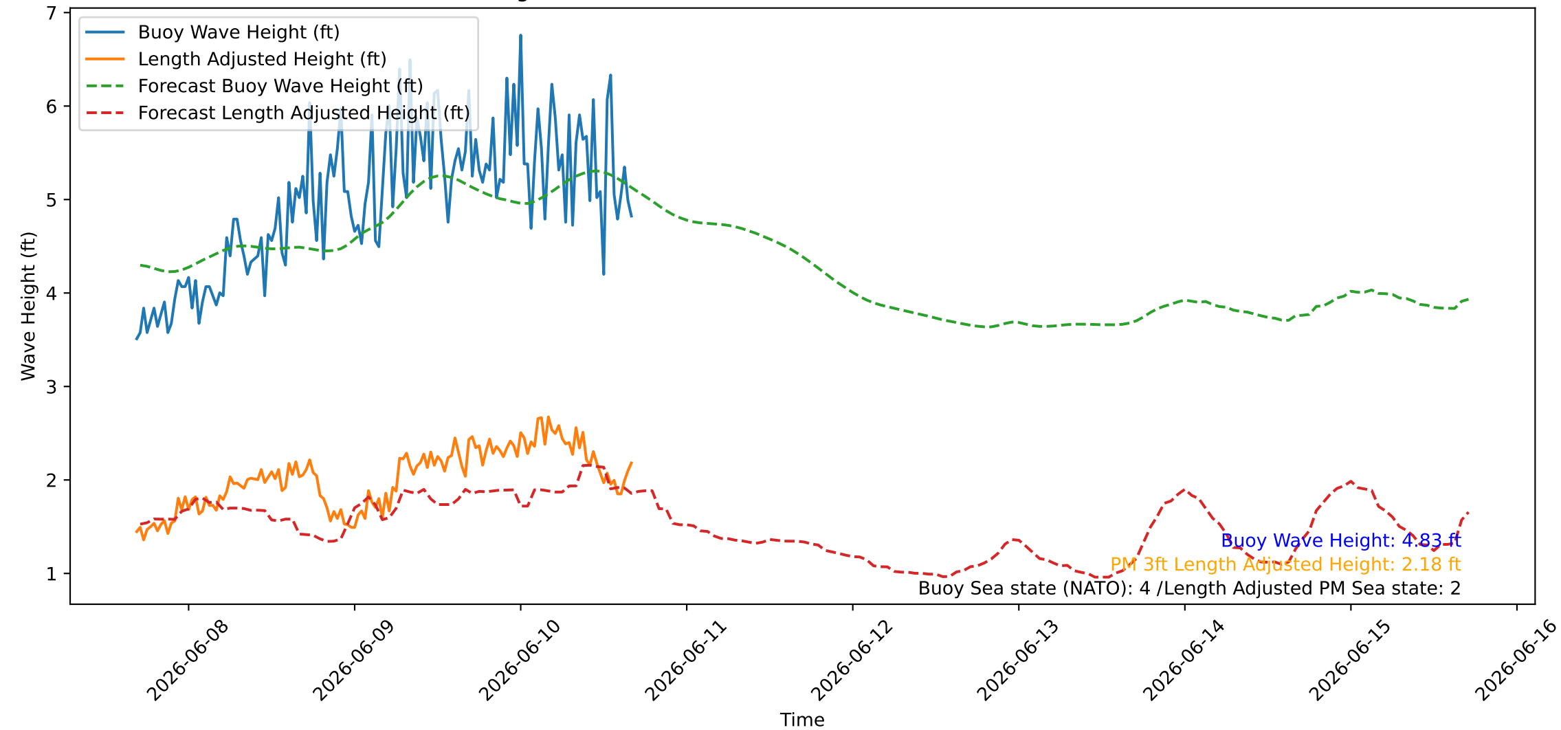
Wave Heights over Time for Oceanside Harbor at 2026-06-10 16:40:26
