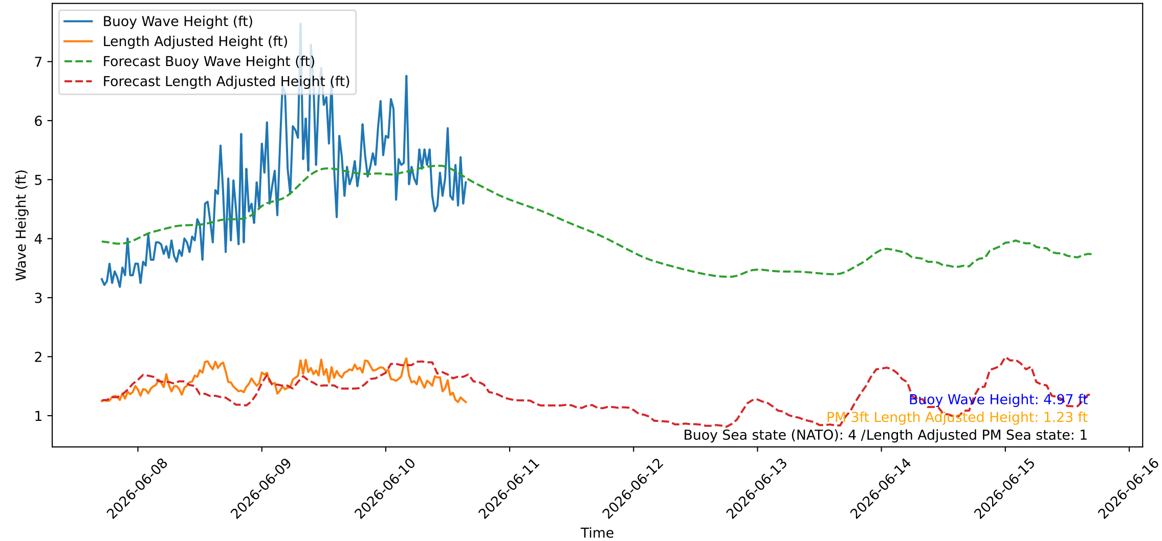
Wave Heights over Time for Red Beach at 2026-06-10 16:40:46
