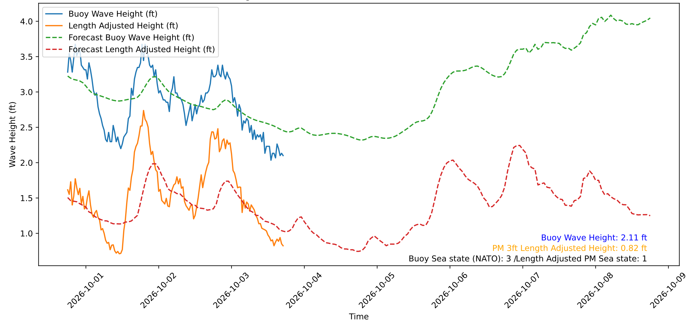
Wave Heights over Time for Green Beach at 2026-10-03 17:51:14
