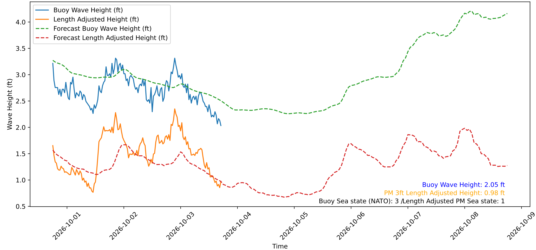
Wave Heights over Time for Oceanside Harbor at 2026-10-03 17:50:30
