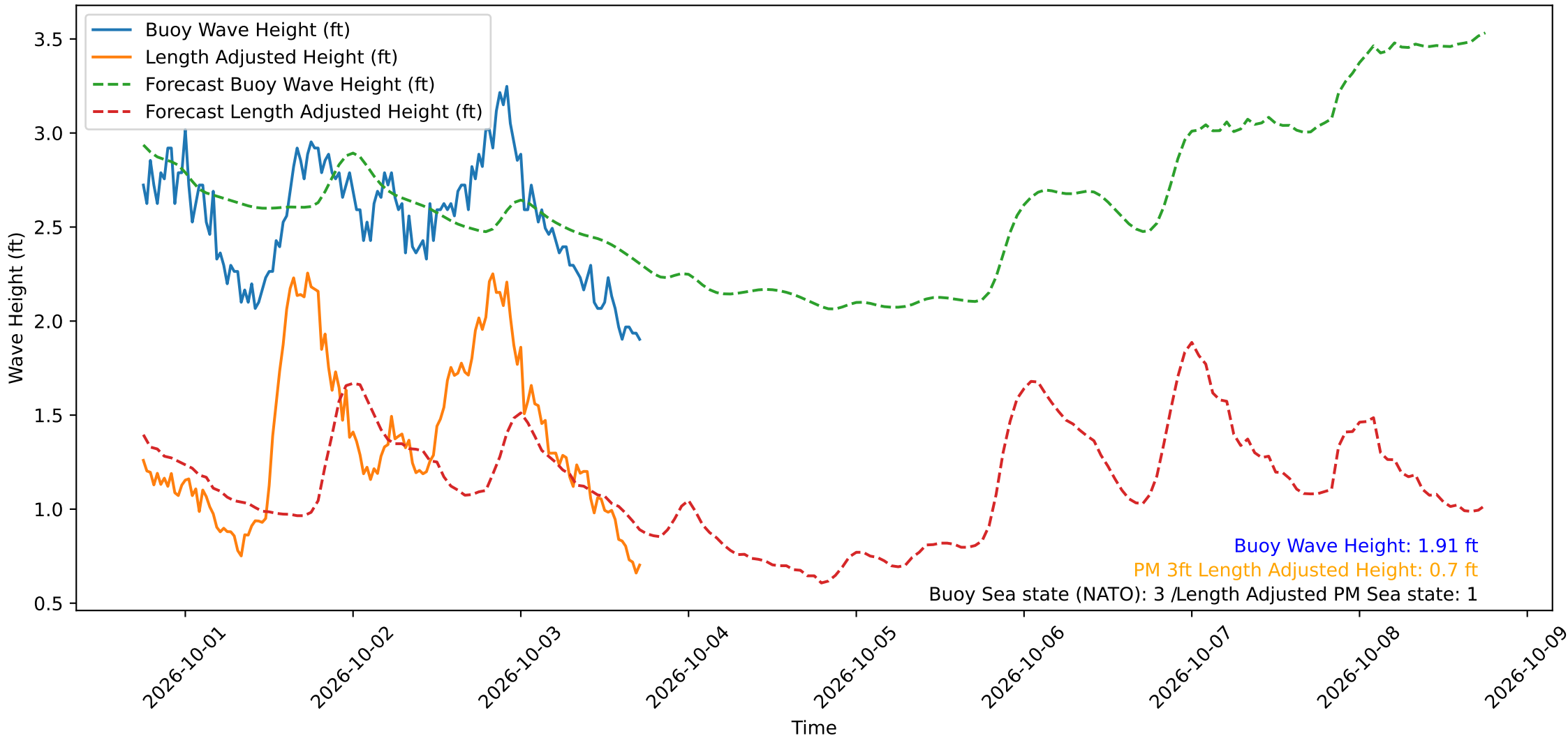
Wave Heights over Time for Red Beach at 2026-10-03 17:50:51
