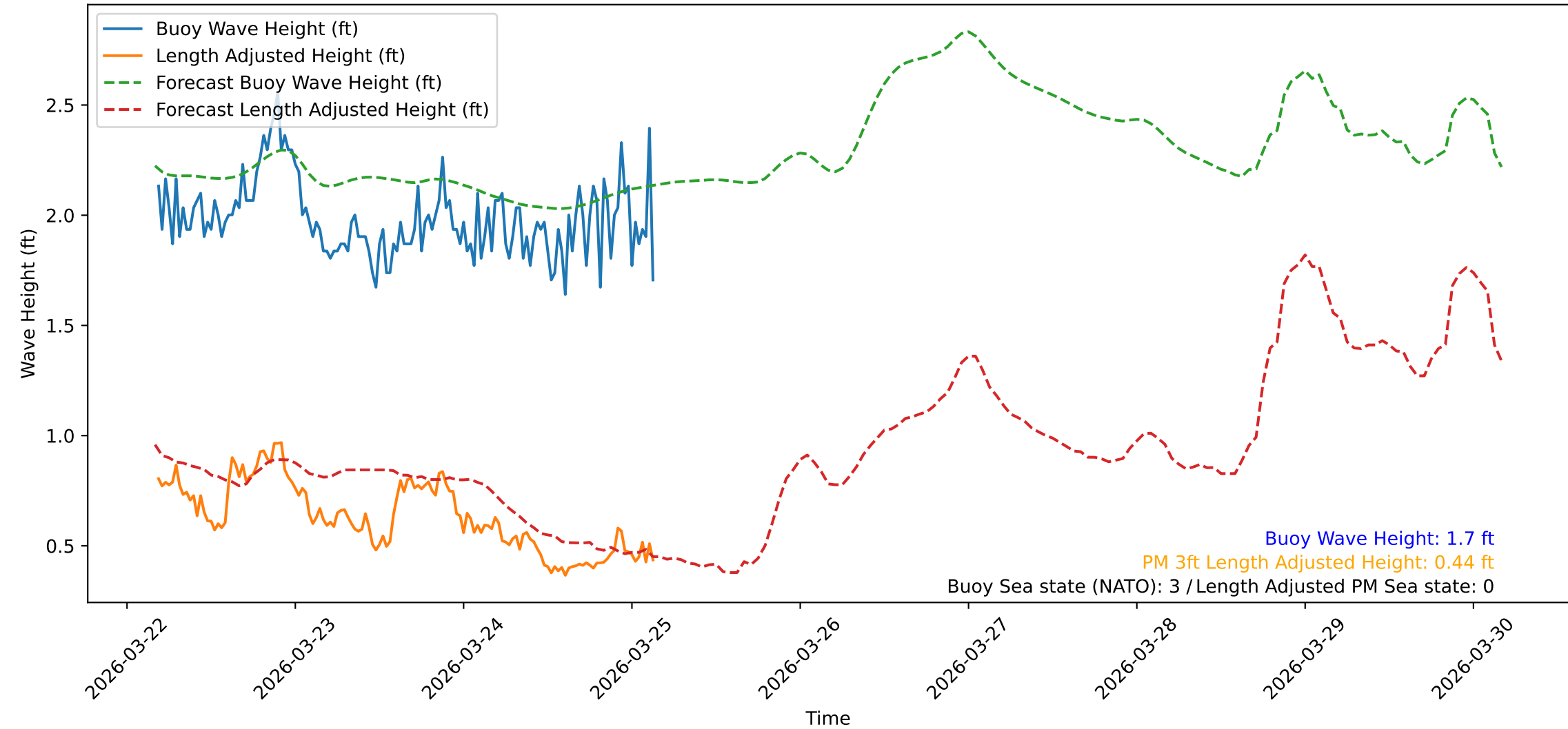
Wave Heights over Time for Red Beach at 2026-03-25 04:00:47
