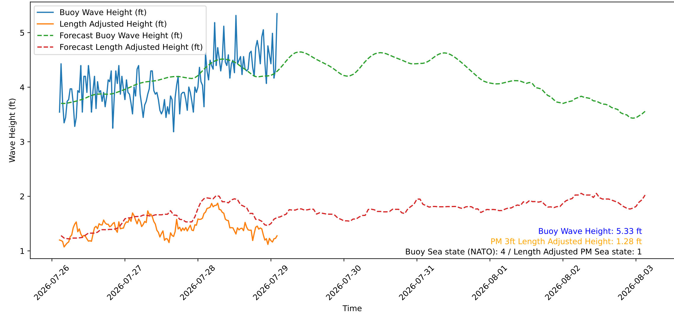
Wave Heights over Time for Oceanside Harbor at 2026-07-29 02:30:26
