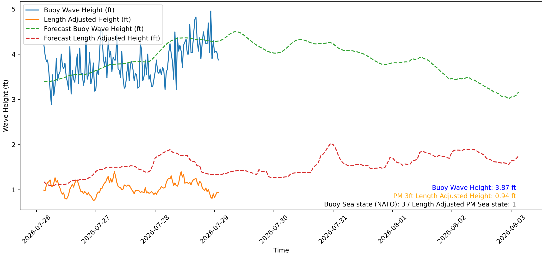
Wave Heights over Time for Red Beach at 2026-07-29 02:30:45
