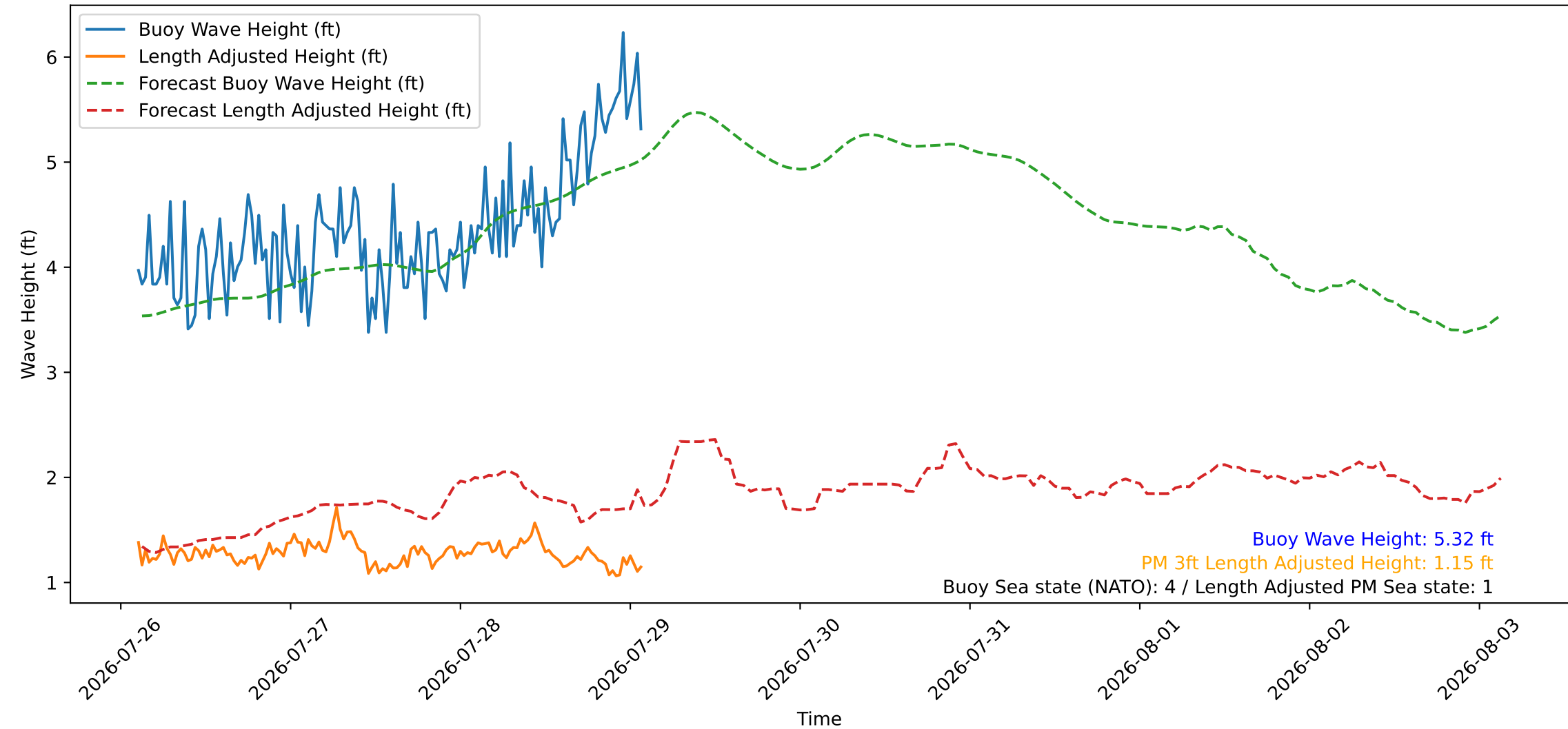
Wave Heights over Time for Green Beach at 2026-07-29 02:31:08
