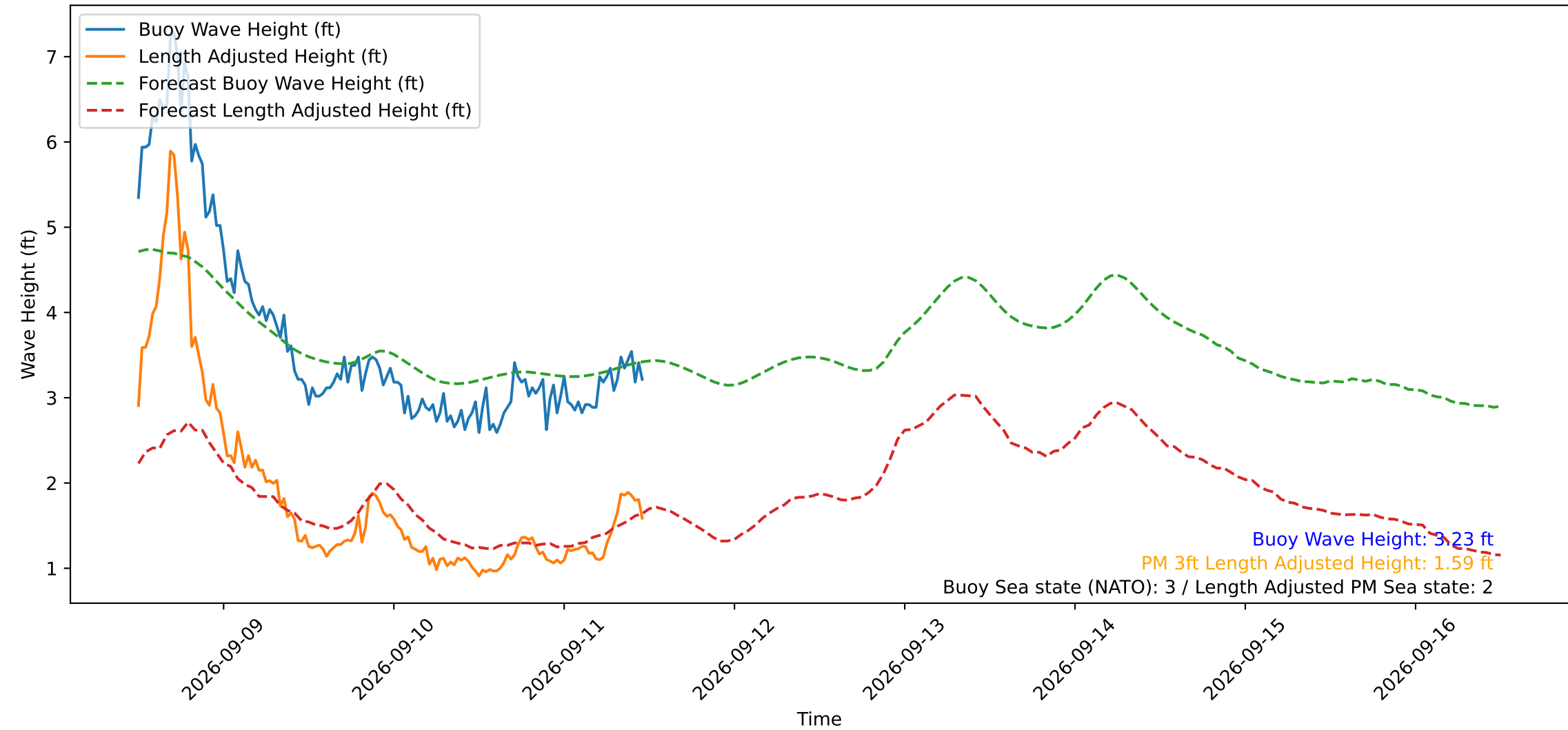
Wave Heights over Time for Green Beach at 2026-09-11 11:41:11
