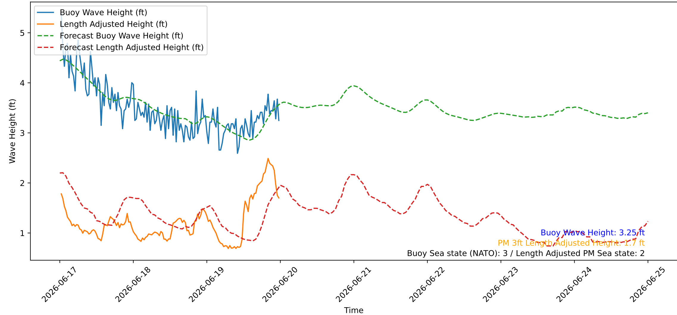
Wave Heights over Time for Red Beach at 2026-06-20 00:10:45
