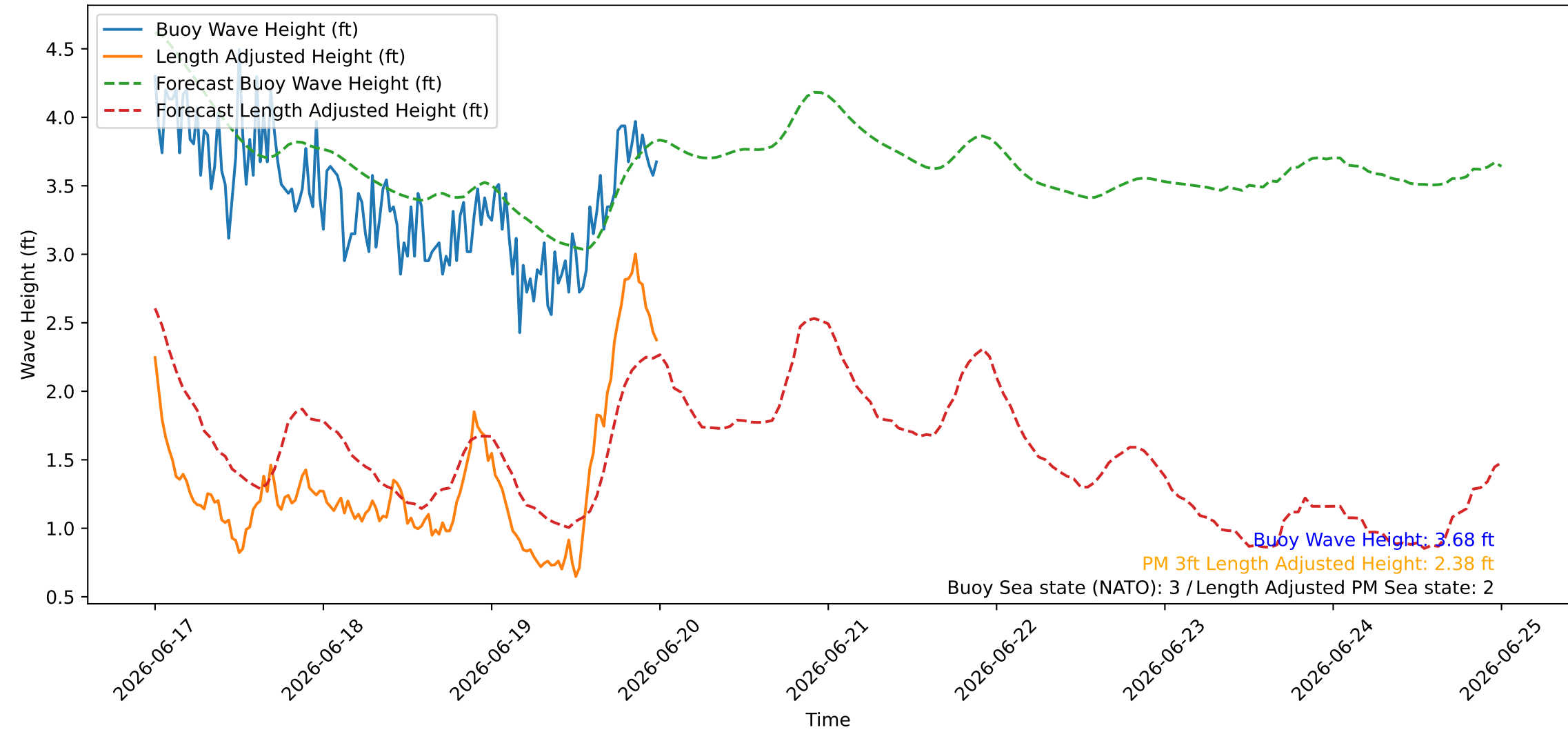
Wave Heights over Time for Green Beach at 2026-06-20 00:11:07
