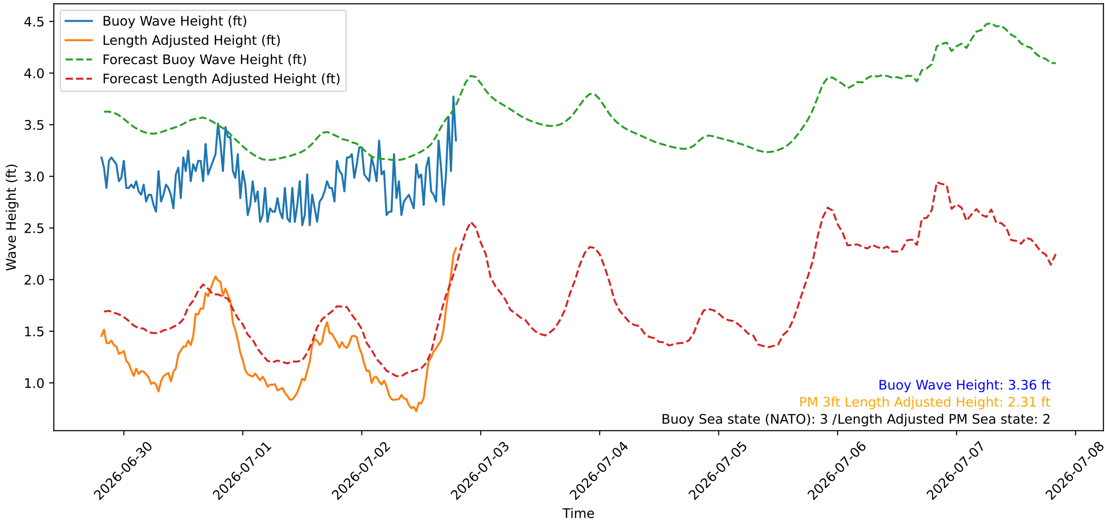
Wave Heights over Time for Green Beach at 2026-07-02 19:41:08
