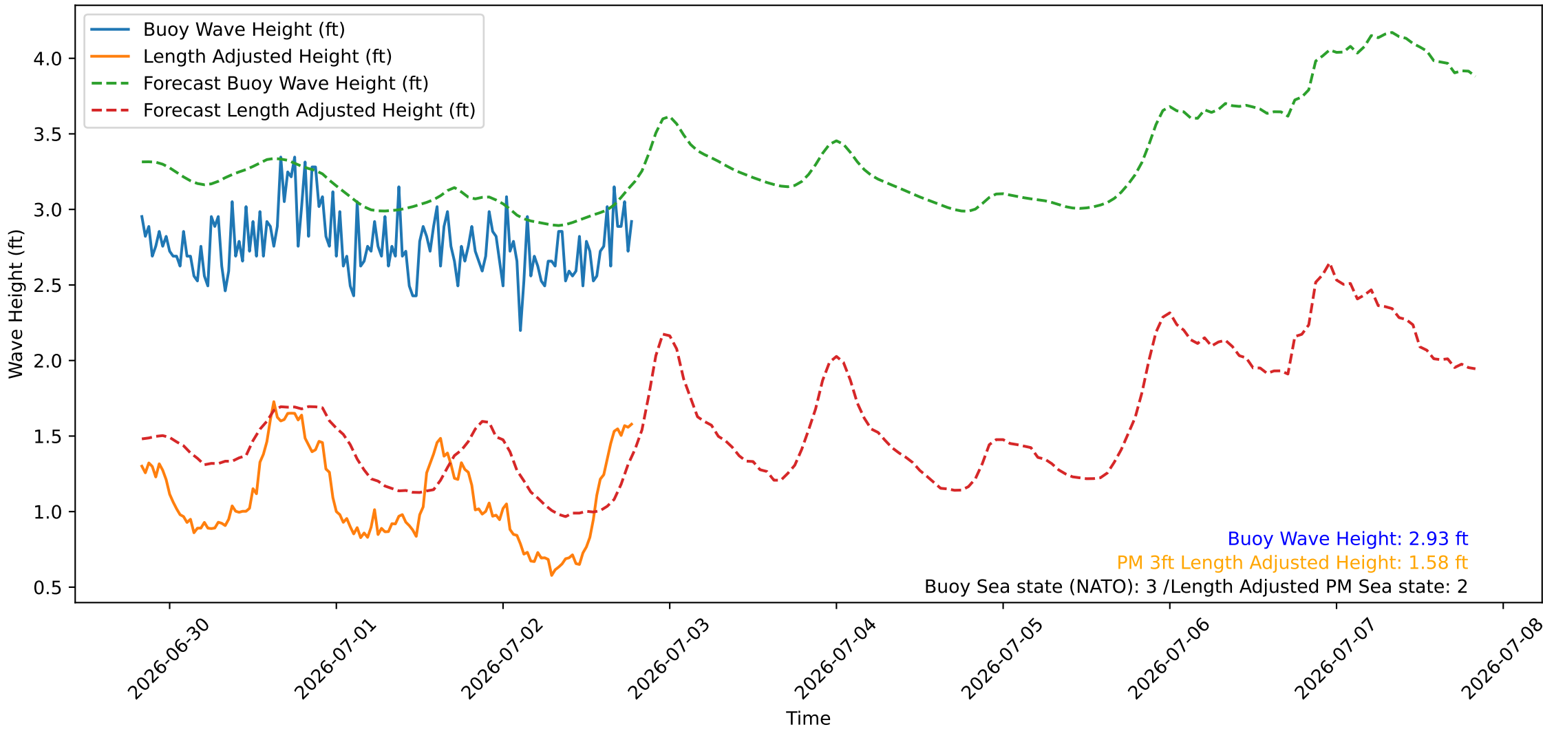
Wave Heights over Time for Red Beach at 2026-07-02 19:40:45
