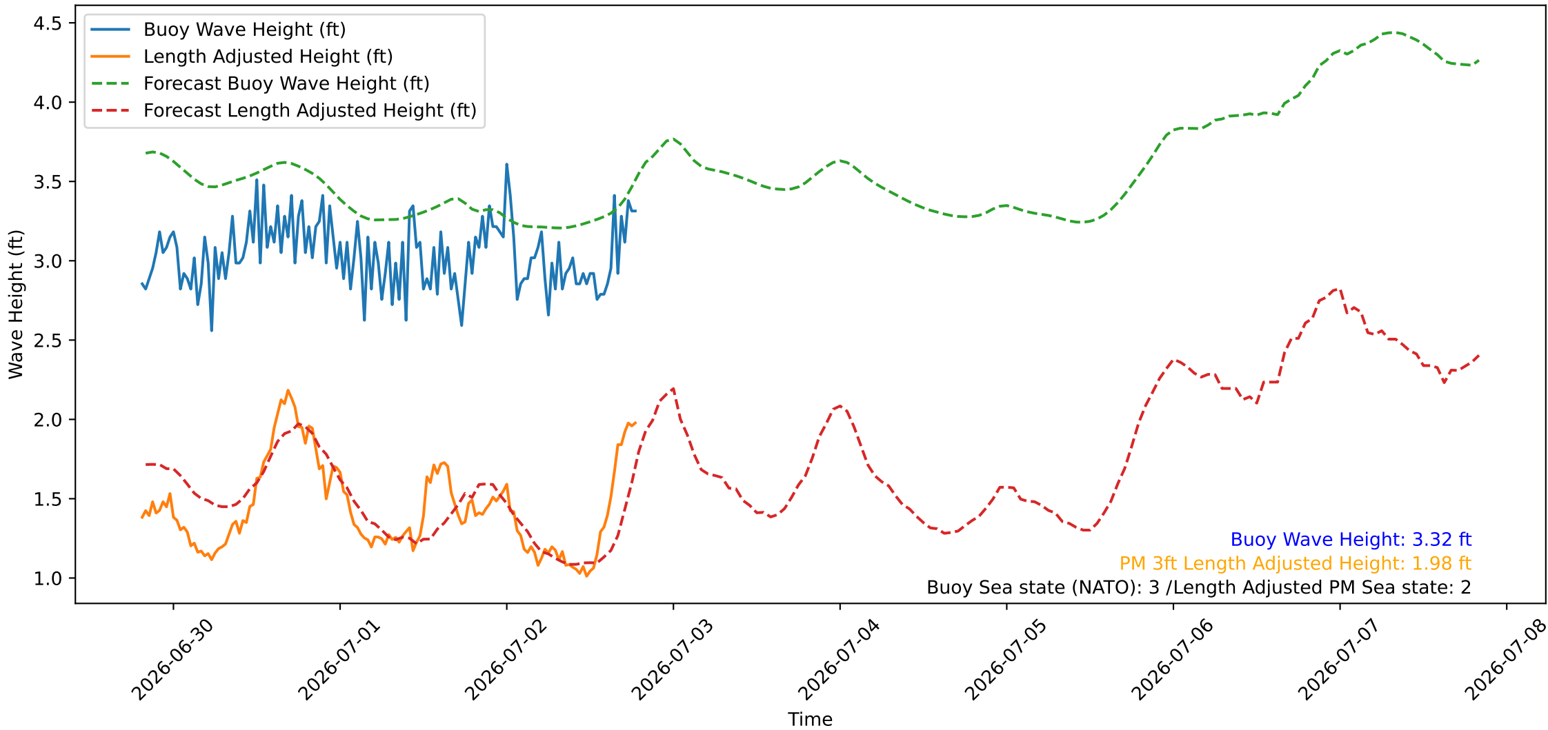
Wave Heights over Time for Oceanside Harbor at 2026-07-02 19:40:26
