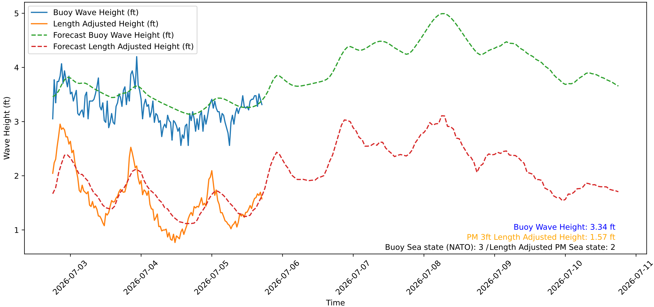
Wave Heights over Time for Green Beach at 2026-07-05 17:51:10
