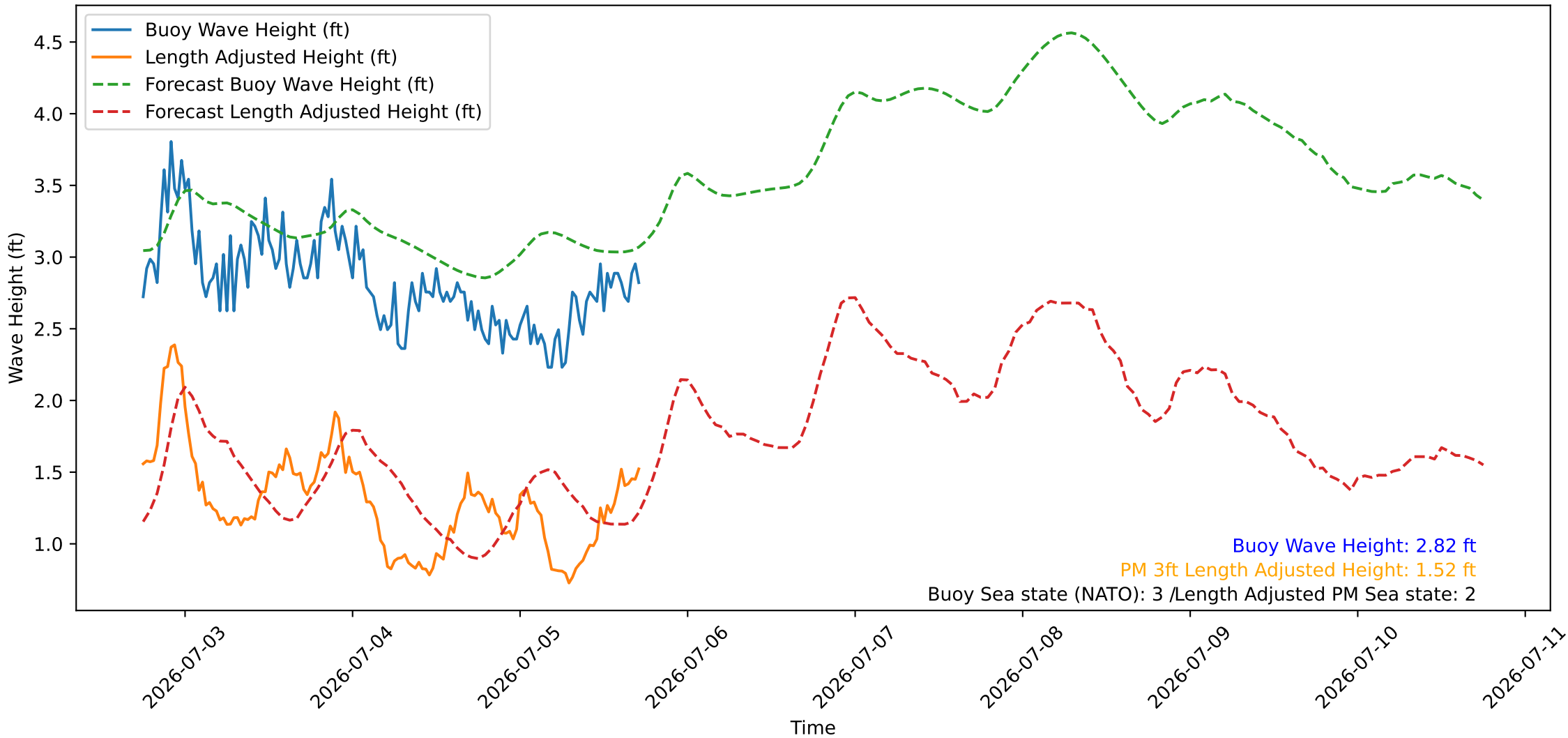
Wave Heights over Time for Red Beach at 2026-07-05 17:50:47
