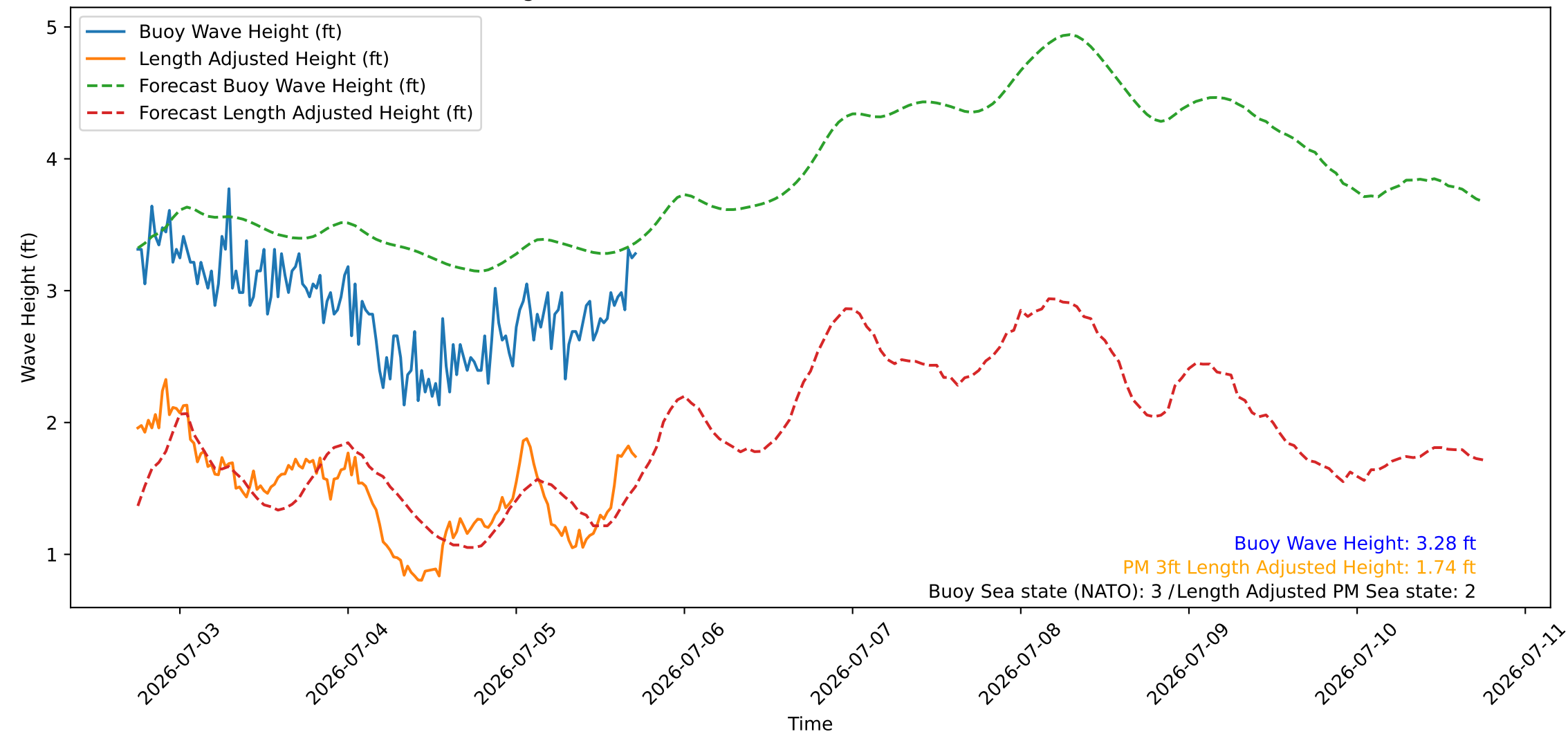
Wave Heights over Time for Oceanside Harbor at 2026-07-05 17:50:26
