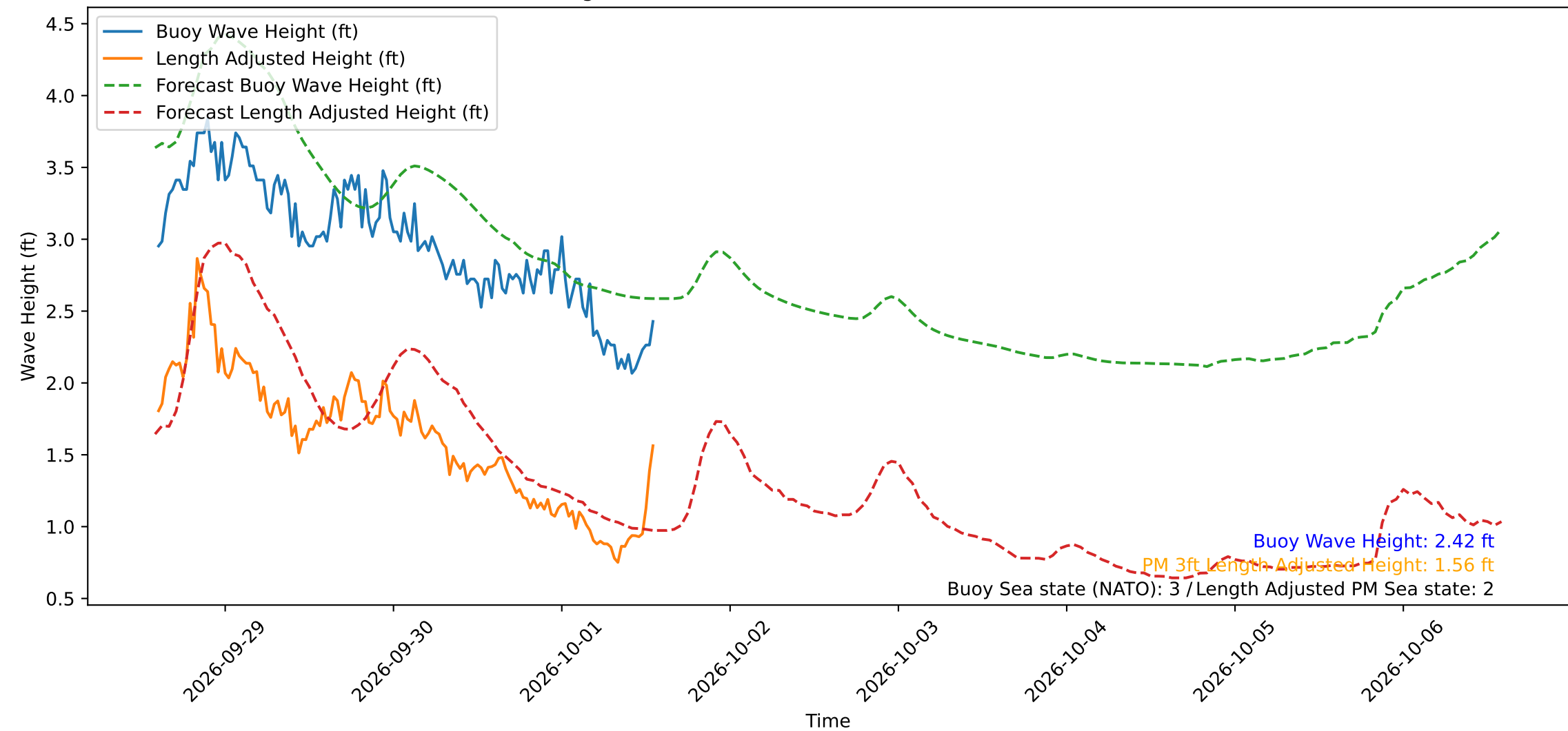
Wave Heights over Time for Red Beach at 2026-10-01 14:00:49
