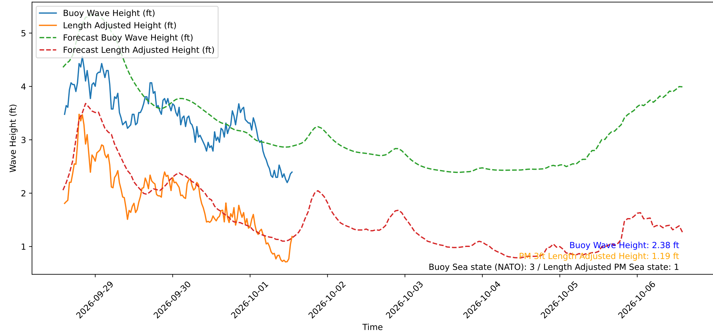
Wave Heights over Time for Green Beach at 2026-10-01 14:01:12
