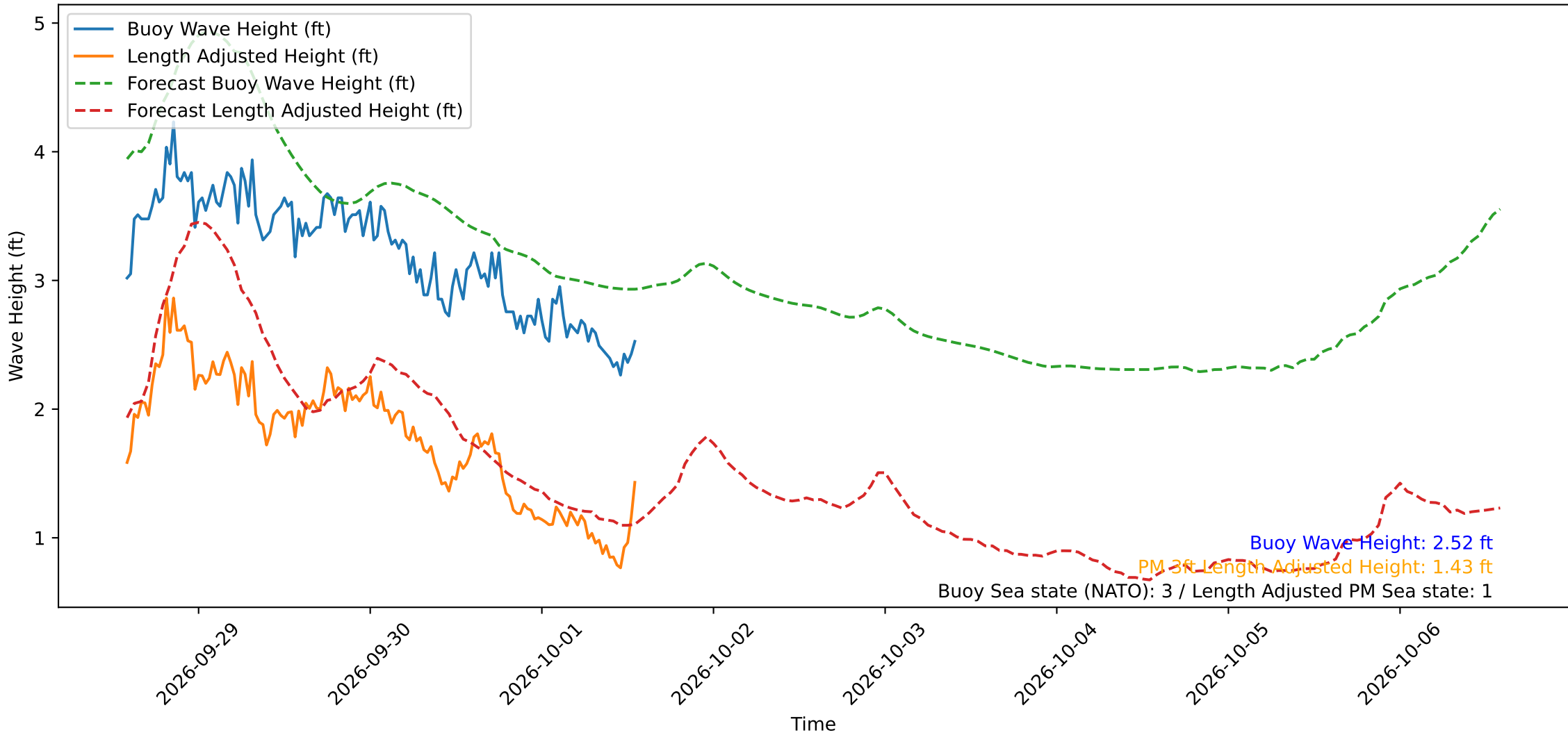
Wave Heights over Time for Oceanside Harbor at 2026-10-01 14:00:30
