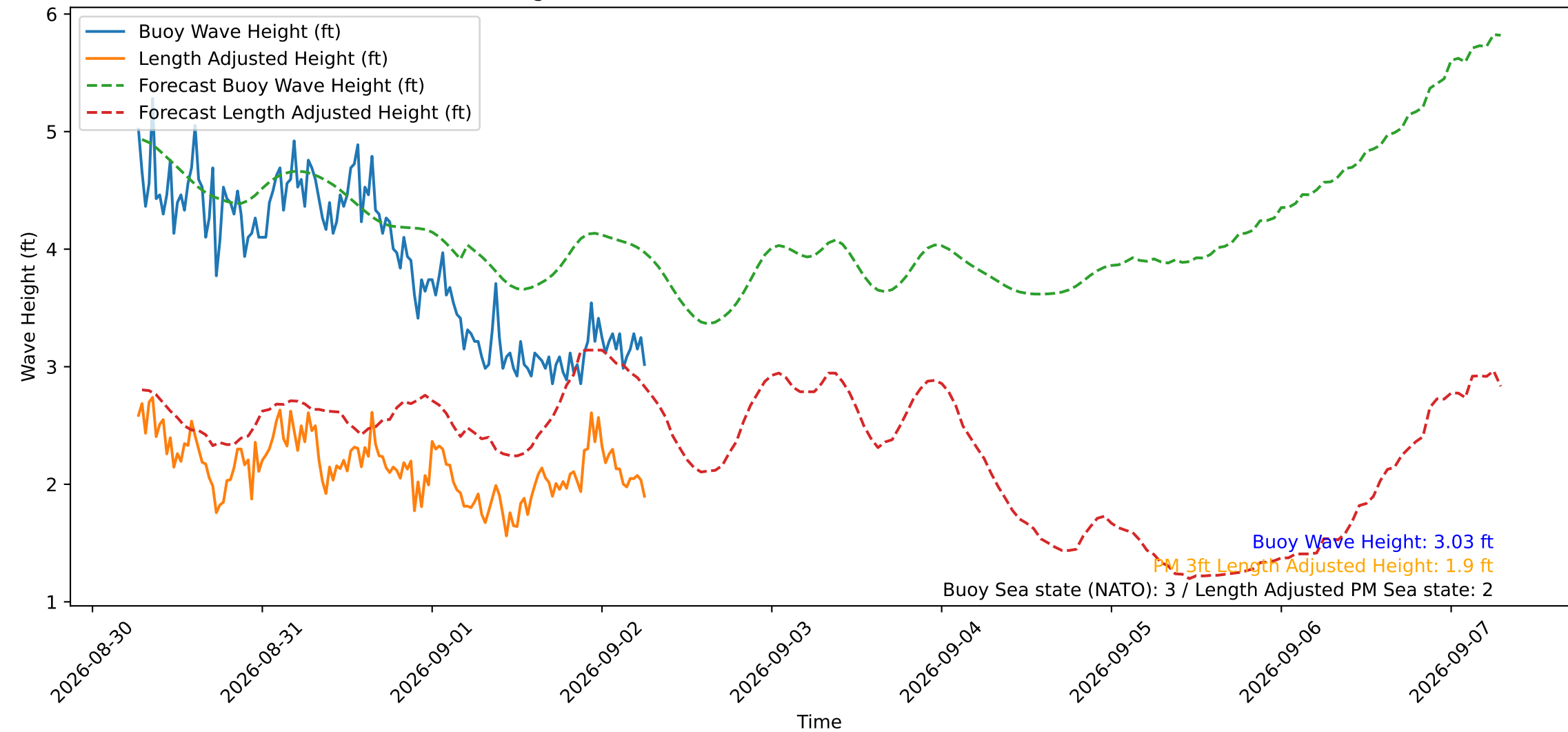
Wave Heights over Time for Oceanside Harbor at 2026-09-02 06:30:29
