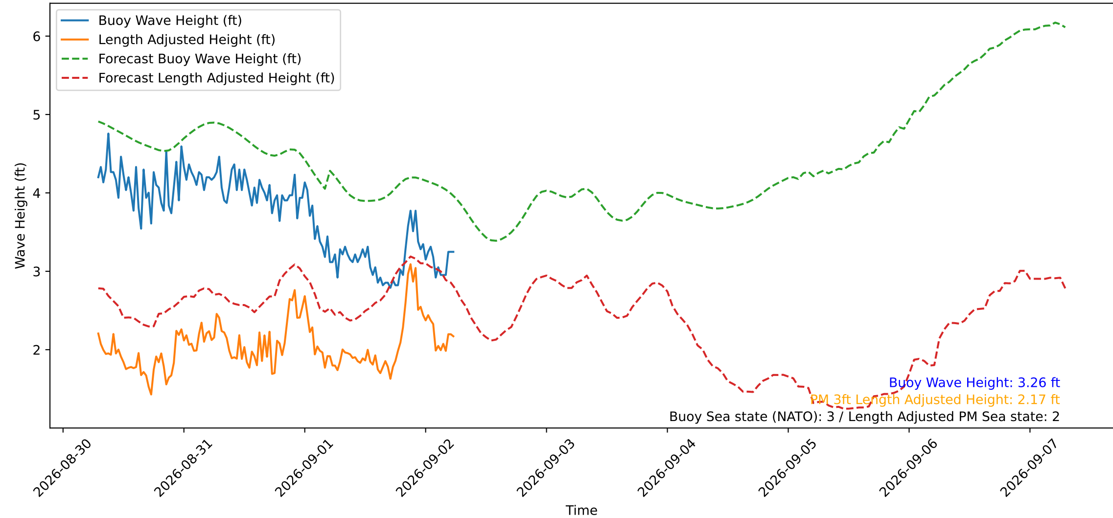
Wave Heights over Time for Green Beach at 2026-09-02 06:31:11
