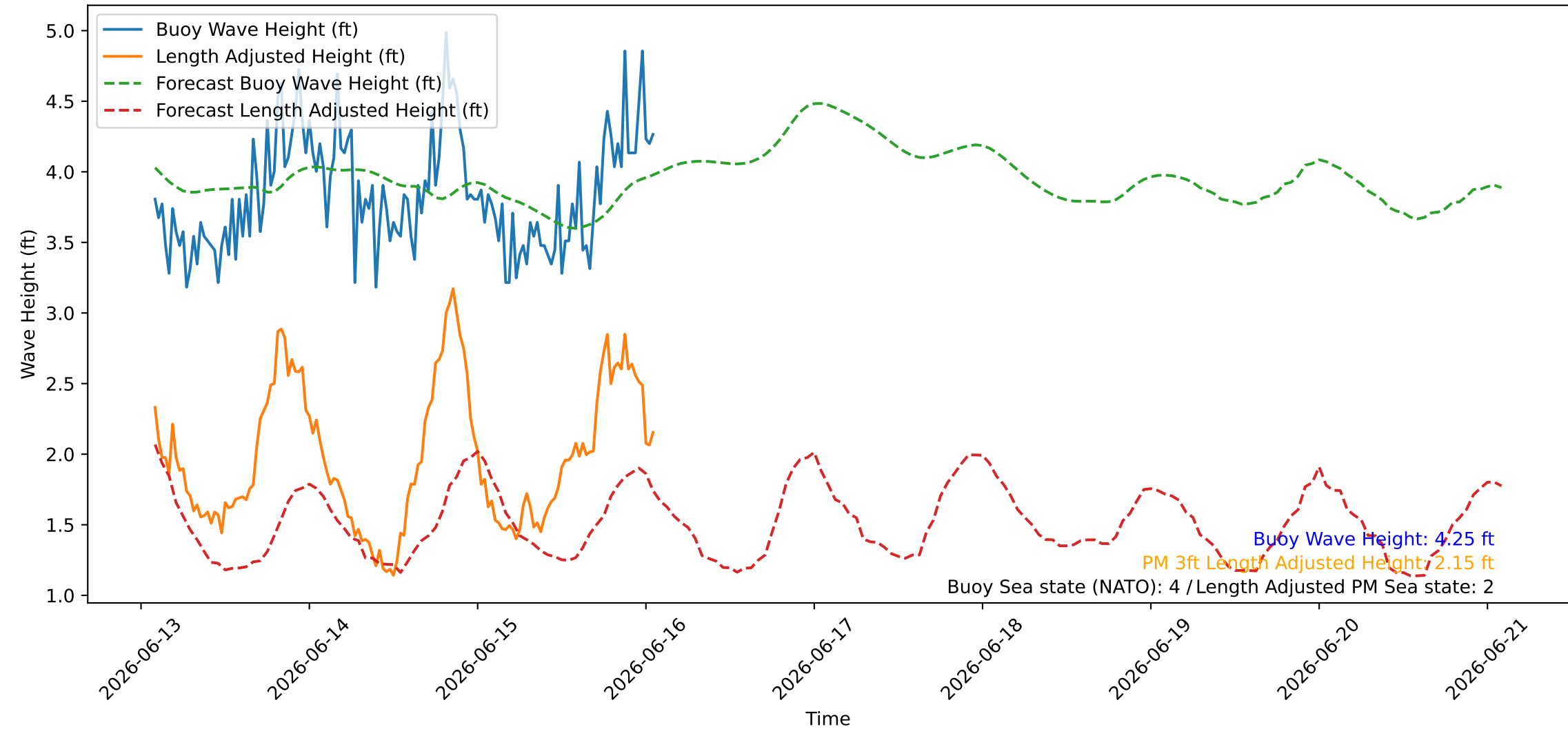
Wave Heights over Time for Oceanside Harbor at 2026-06-16 01:50:26
