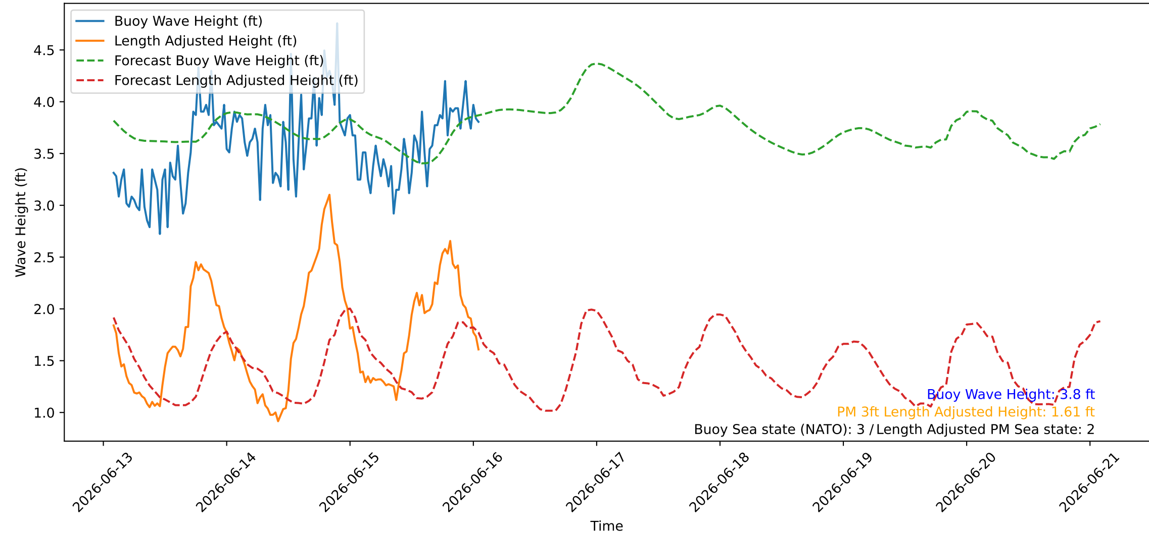
Wave Heights over Time for Red Beach at 2026-06-16 01:50:47
