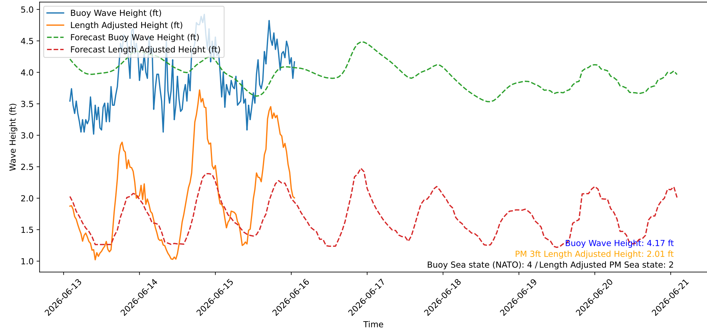
Wave Heights over Time for Green Beach at 2026-06-16 01:51:09
